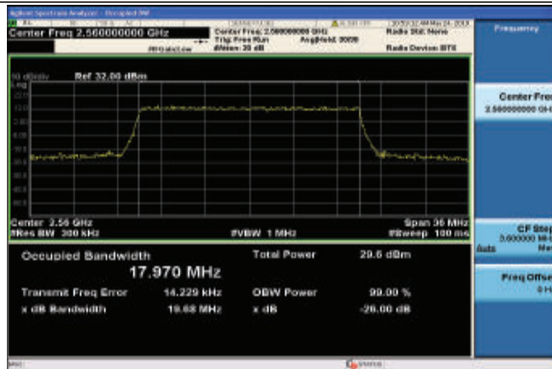
Band7-20MHz-16QAM-21350-100RB#0-17.970
