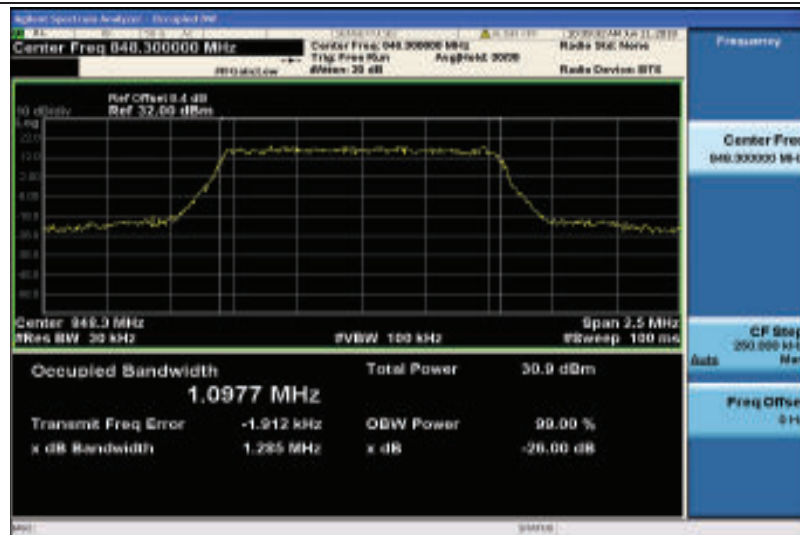
Band5-1.4MHz-QPSK-20643-6RB#0-1.0977
