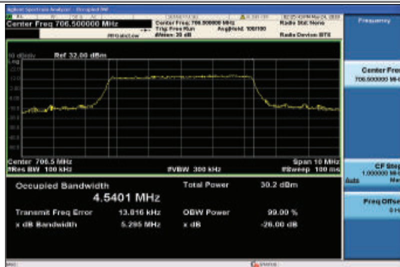
Band17-5MHz-16QAM-23755-25RB#0-4.5401
