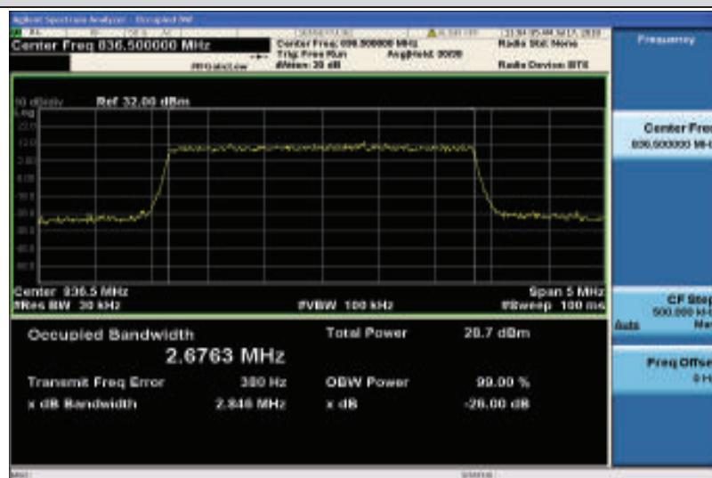
Band26-3MHz-16QAM-26915-15RB#0-2.6763
