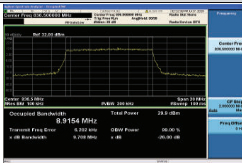
Band26-10MHz-QPSK-26915-50RB#0-8.9154
