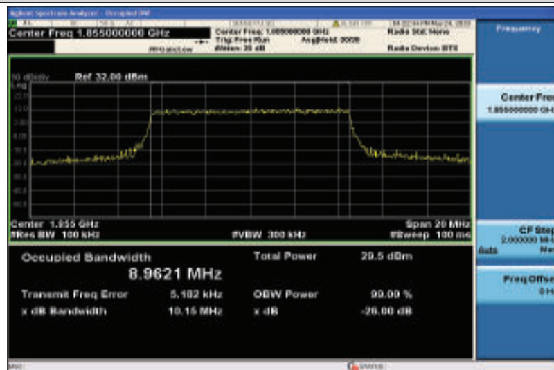
Band25-10MHz-16QAM-26090-50RB#0-8.9621
