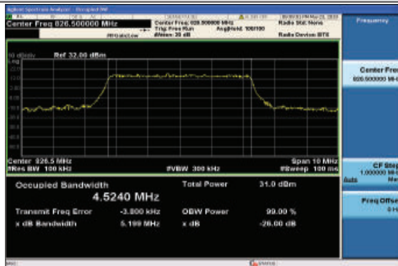
Band5-5MHz-16QAM-20425-25RB#0-4.5240
