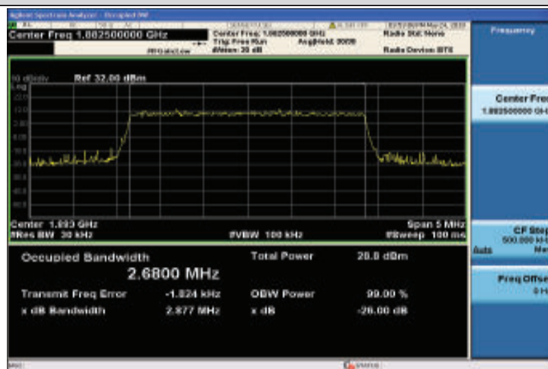
Band25-3MHz-16QAM-26365-15RB#0-2.6800
