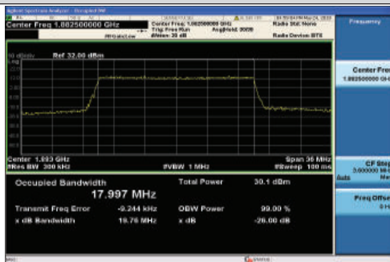
Band25-20MHz-16QAM-26365-100RB#0-17.997
