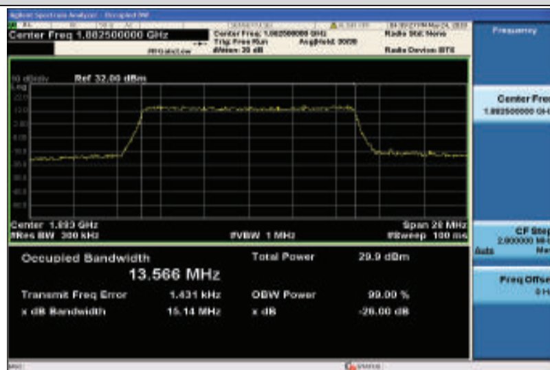
Band25-15MHz-16QAM-26365-75RB#0-13.566
