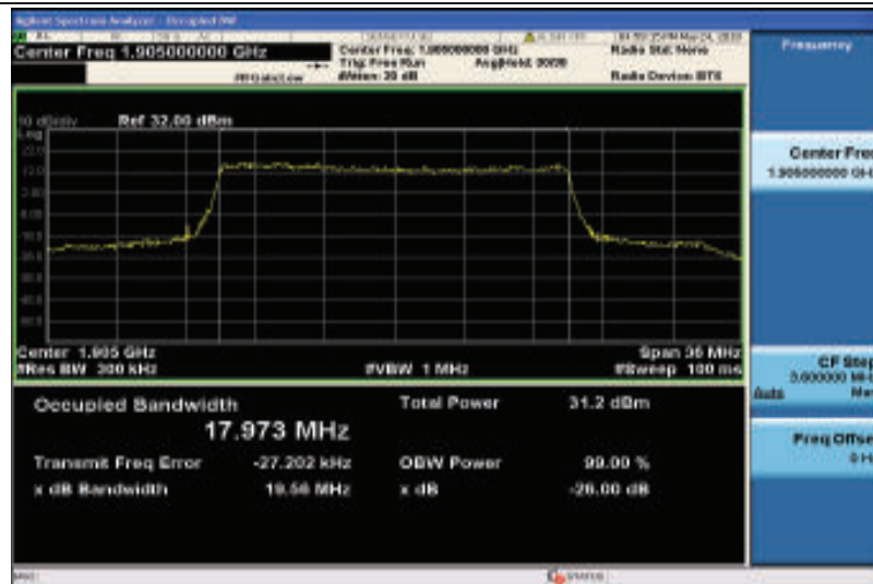
Band25-20MHz-QPSK-26590-100RB#0-17.973
