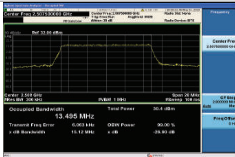
Band7-15MHz-QPSK-20825-75RB#0-13.495
