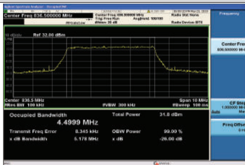
Band5-5MHz-QPSK-20525-25RB#0-4.4999
