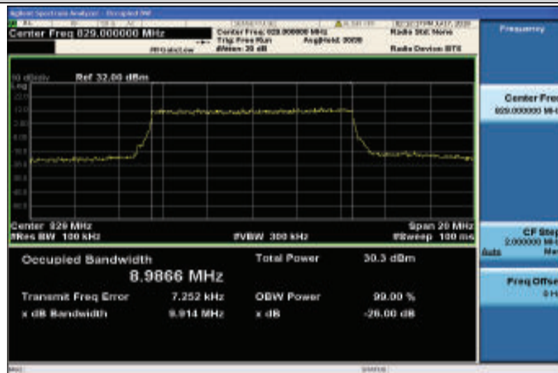
Band26-10MHz-QPSK-26840-50RB#0-8.9866
