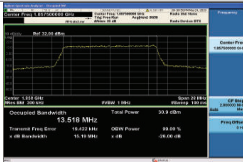
Band25-15MHz-QPSK-26115-75RB#0-13.518
