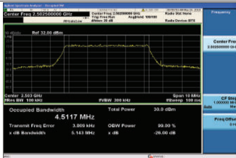
Band7-5MHz-QPSK-20775-25RB#0-4.5117
