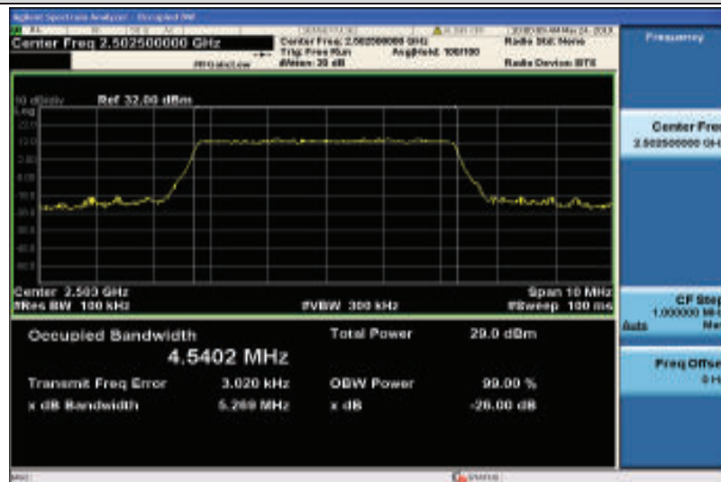
Band7-5MHz-16QAM-20775-25RB#0-4.5402
