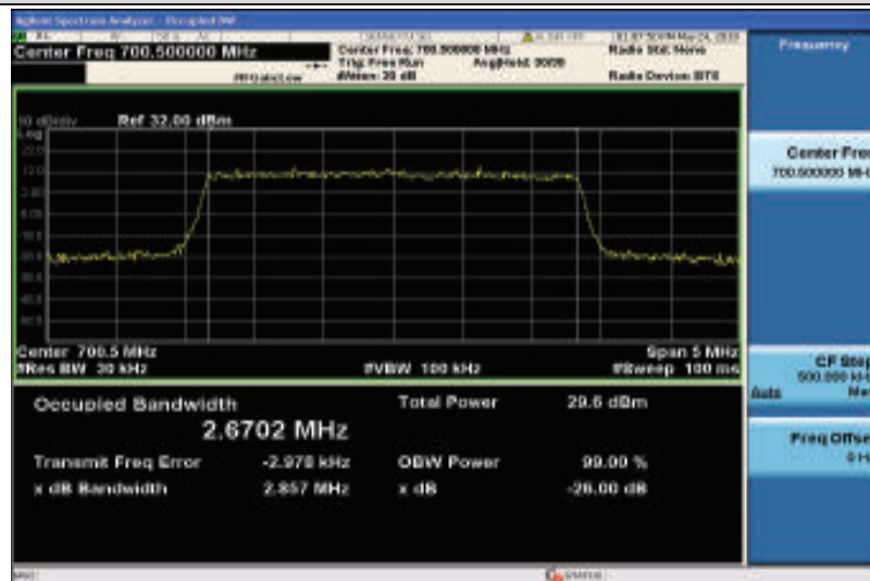
Band12-3MHz-16QAM-23025-15RB#0-2.6702
