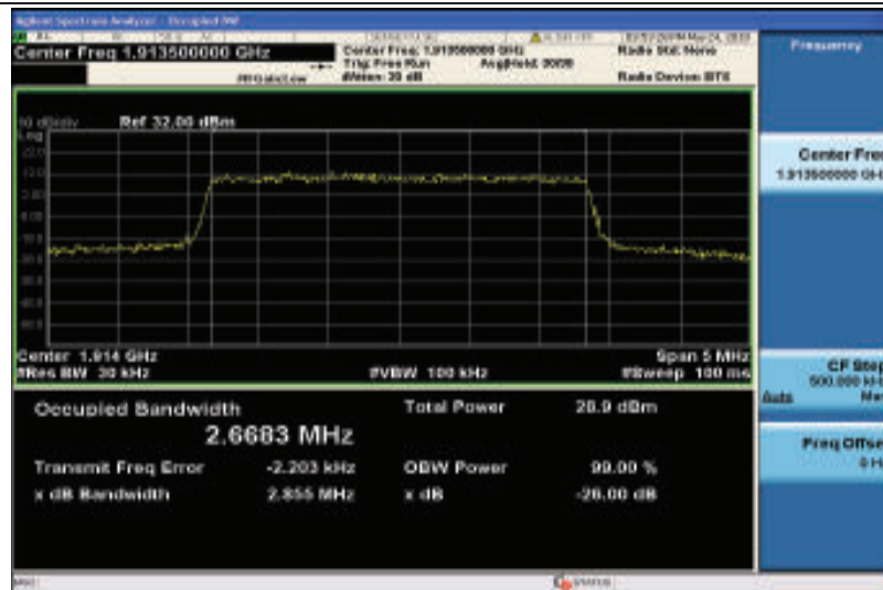
Band25-3MHz-16QAM-26675-15RB#0-2.6683
