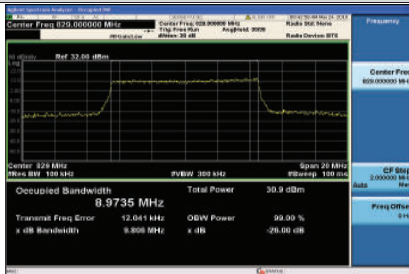
Band5-10MHz-16QAM-20450-50RB#0-8.9735
