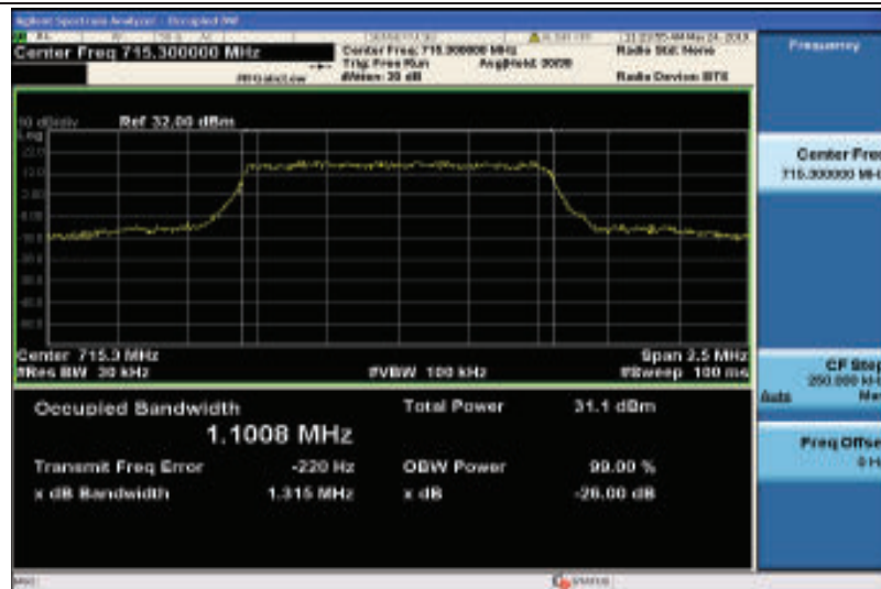
Band12-1.4MHz-QPSK-23173-6RB#0-1.1008
