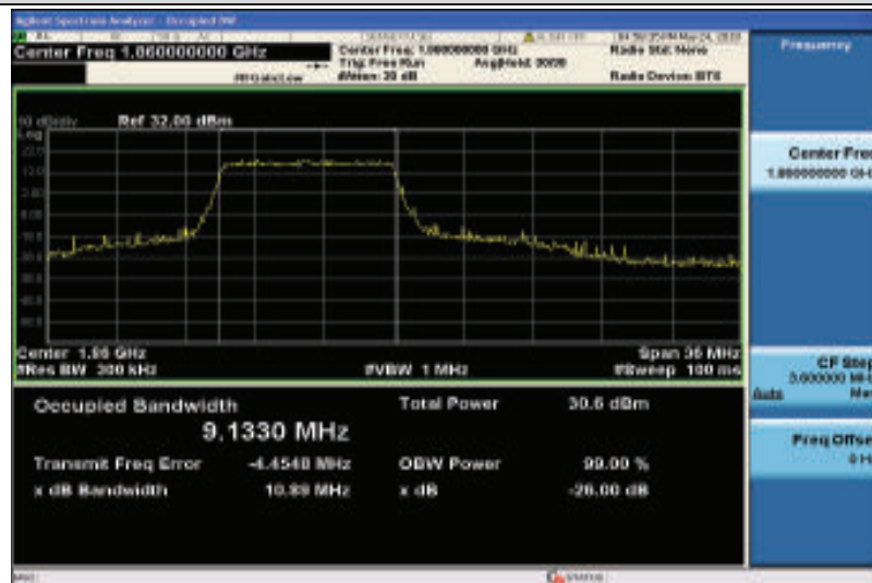
Band25-20MHz-QPSK-26140-100RB#0-9.1330
