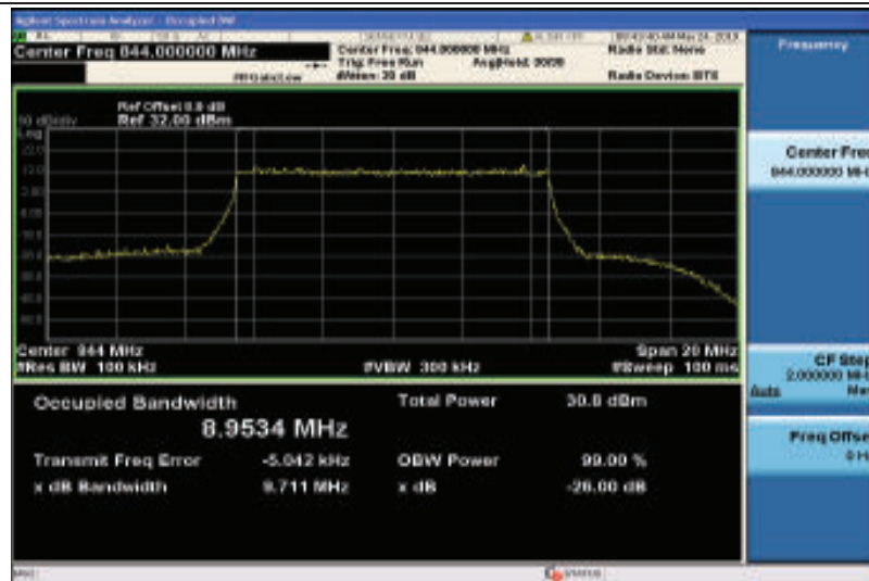
Band5-10MHz-16QAM-20600-50RB#0-8.9534
