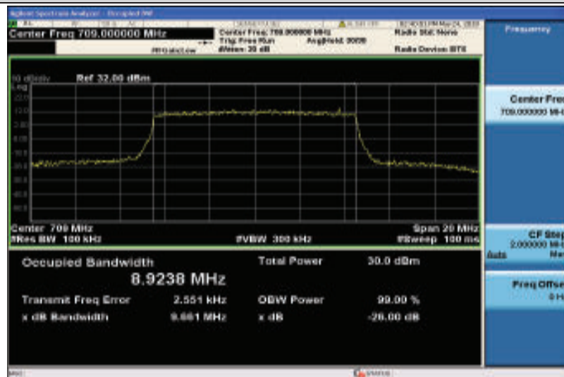
Band17-10MHz-16QAM-23780-50RB#0-8.9238
