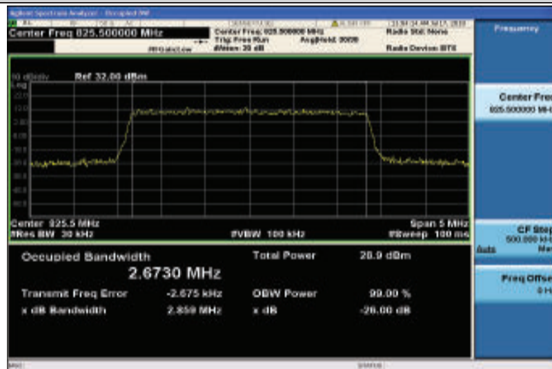
Band26-3MHz-16QAM-26805-15RB#0-2.6730
