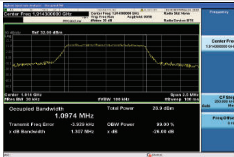
Band25-1.4MHz-16QAM-26683-6RB#0-1.0974
