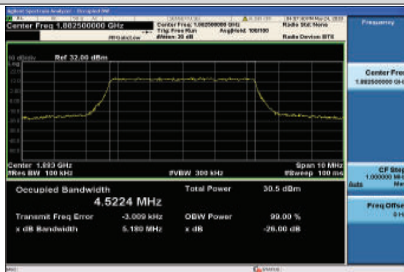
Band25-5MHz-QPSK-26365-25RB#0-4.5224
