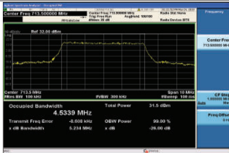
Band12-5MHz-QPSK-23155-25RB#0-4.5339
