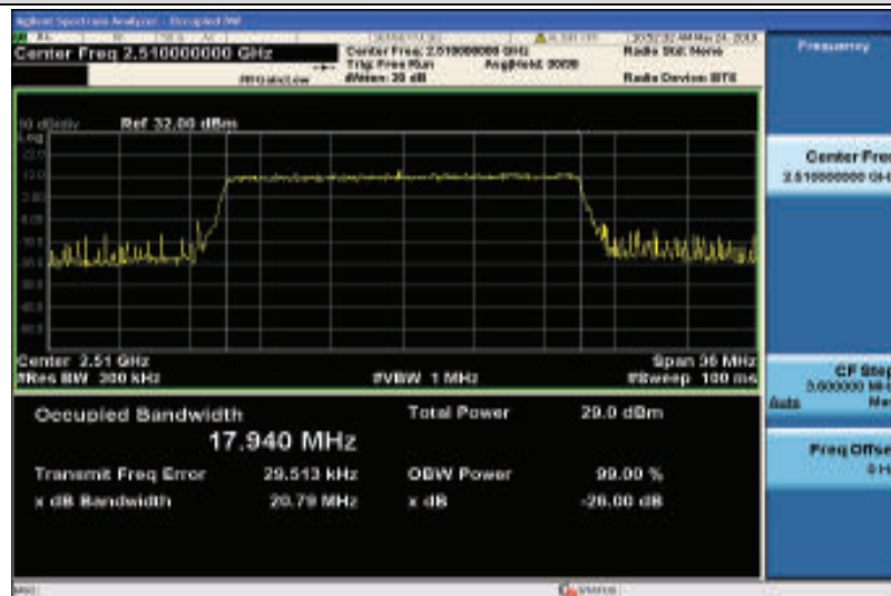
Band7-20MHz-16QAM-20850-100RB#0-17.940
