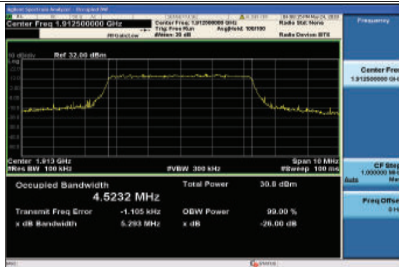
Band25-5MHz-QPSK-26665-25RB#0-4.5232
