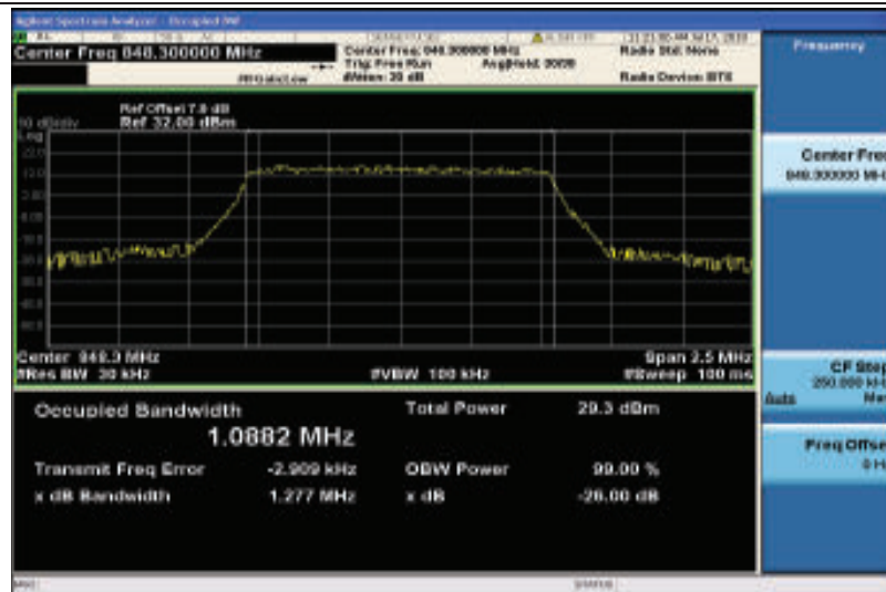
Band26-1.4MHz-QPSK-27033-6RB#0-1.0882
