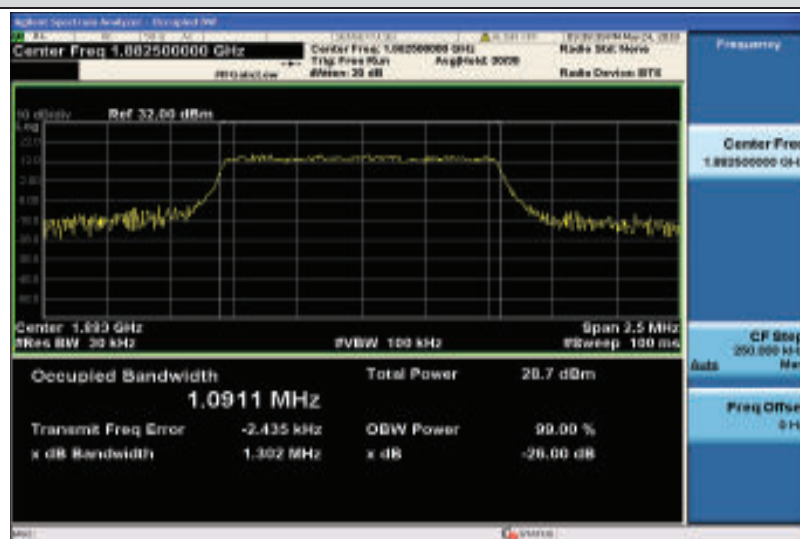
Band25-1.4MHz-16QAM-26365-6RB#0-1.0911
