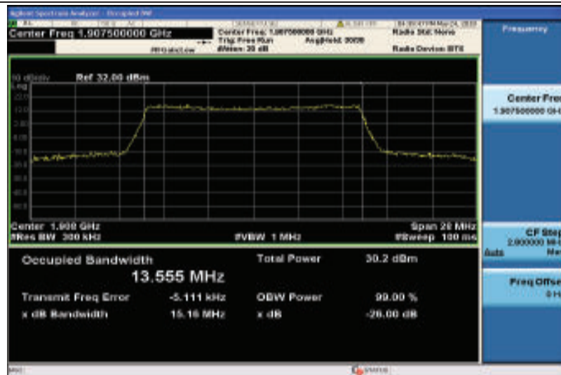
Band25-15MHz-16QAM-26615-75RB#0-13.555
