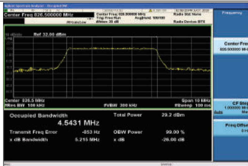
Band26-5MHz-16QAM-26815-25RB#0-4.5431
