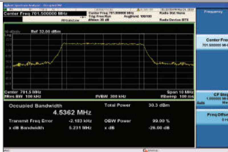
Band12-5MHz-16QAM-23035-25RB#0-4.5362
