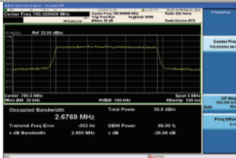
Band12-3MHz-QPSK-23025-15RB#0-2.6769
