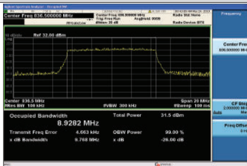
Band5-10MHz-QPSK-20525-50RB#0-8.9282
