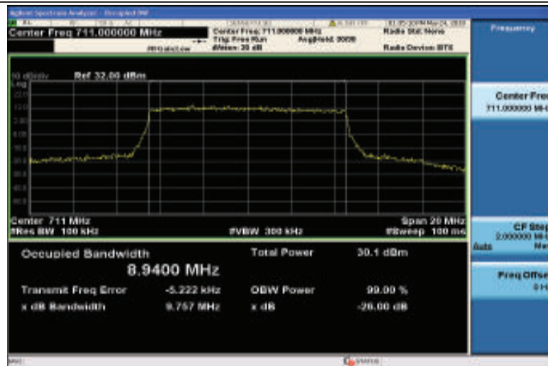
Band12-10MHz-16QAM-23130-50RB#0-8.9400
