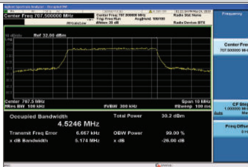
Band12-5MHz-16QAM-23095-25RB#0-4.5246
