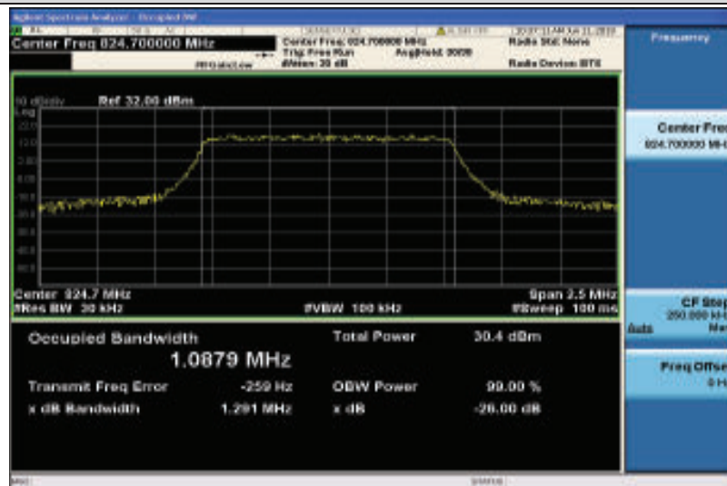
Band5-1.4MHz-QPSK-20407-6RB#0-1.0879
