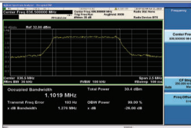
Band5-1.4MHz-QPSK-20525-6RB#0-1.1019
