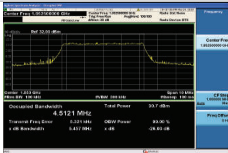
Band25-5MHz-QPSK-26065-25RB#0-4.5121
