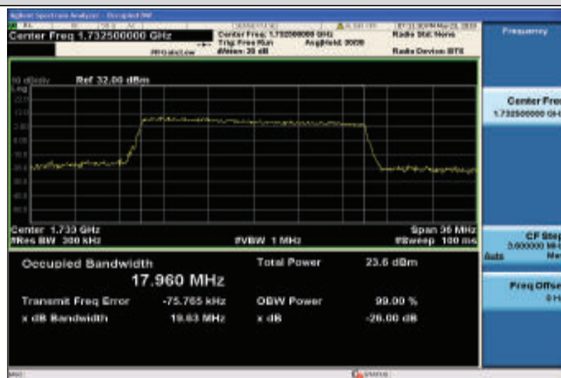
Band4-20MHz-16QAM-20175-100RB#0-17.960
