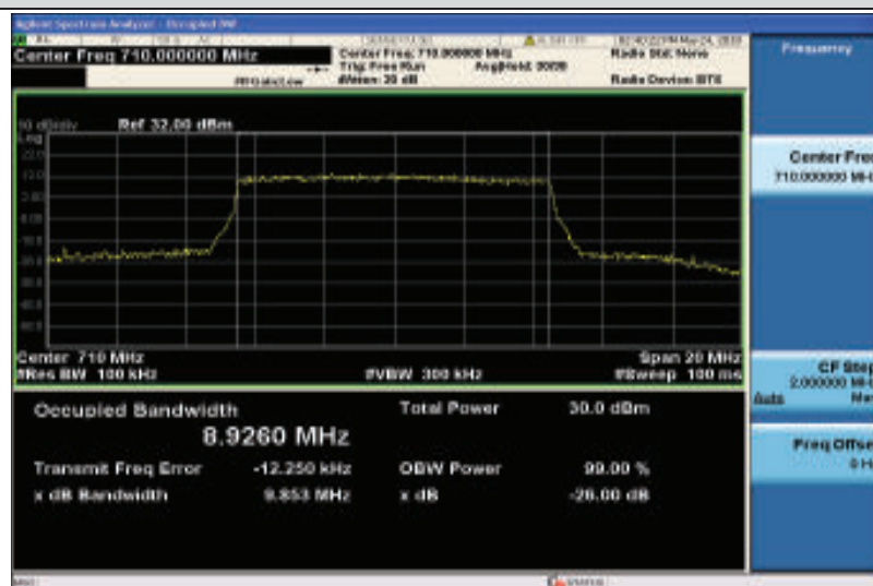
Band17-10MHz-16QAM-23790-50RB#0-8.9260
