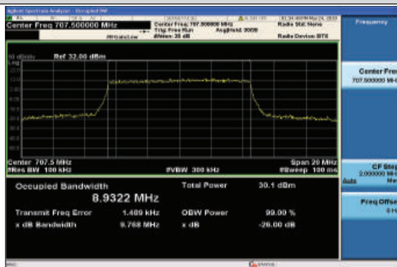
Band12-10MHz-16QAM-23095-50RB#0-8.9322
