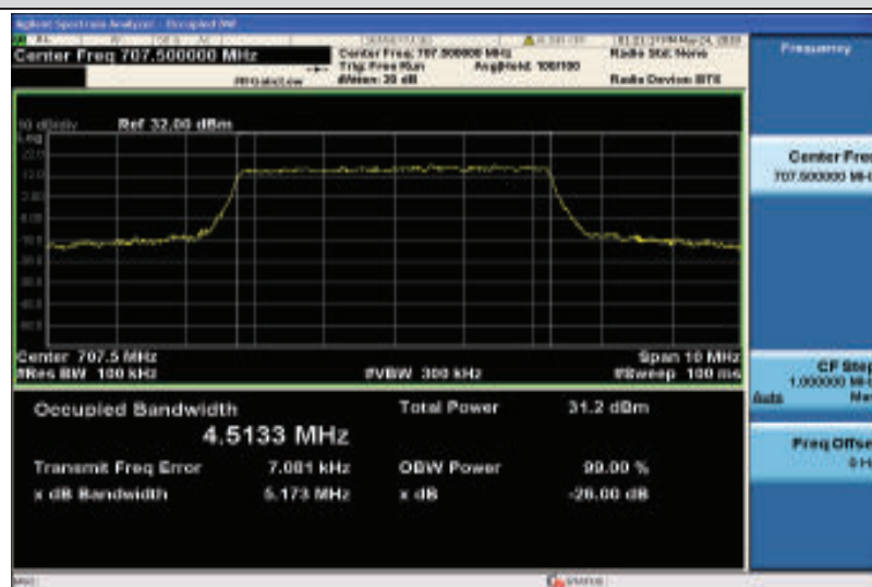
Band12-5MHz-QPSK-23095-25RB#0-4.5133
