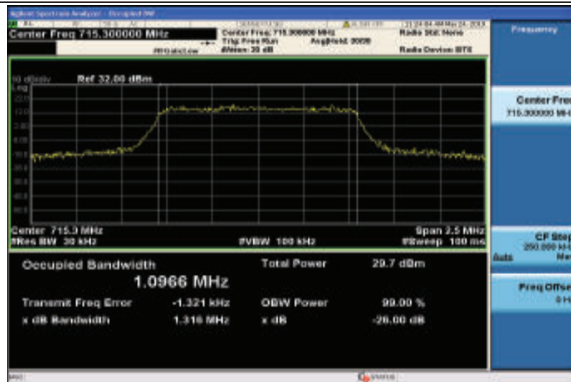
Band12-1.4MHz-16QAM-23173-6RB#0-1.0966
