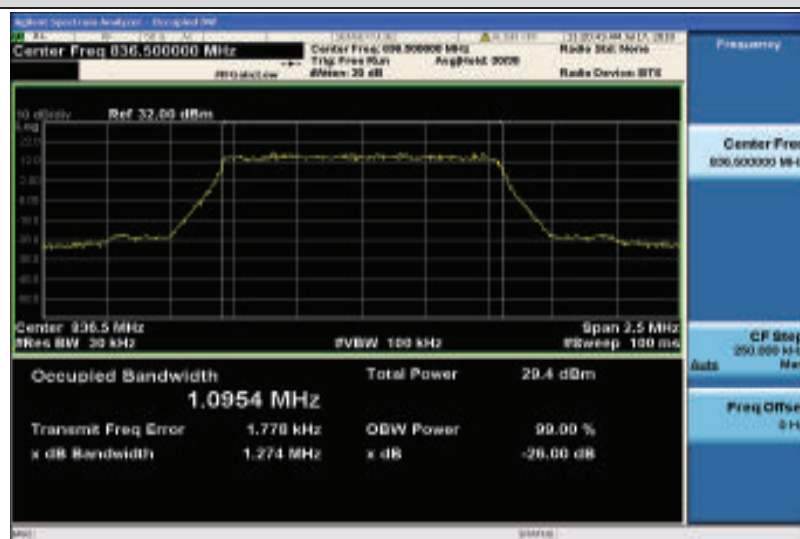
Band26-1.4MHz-QPSK-26915-6RB#0-1.0954
