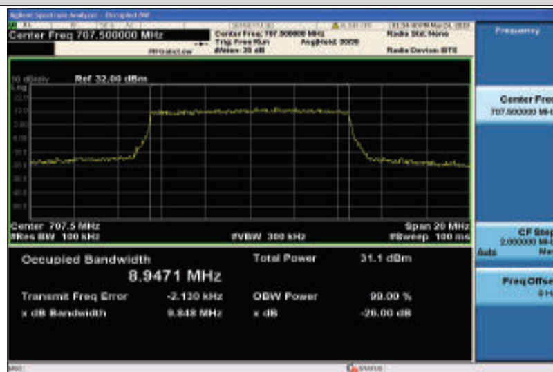
Band12-10MHz-QPSK-23095-50RB#0-8.9471
