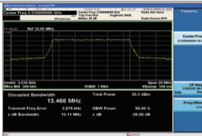
Band7-15MHz-QPSK-21100-75RB#0-13.466
