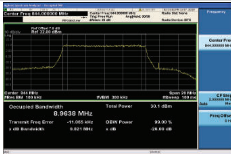
Band26-10MHz-QPSK-26990-50RB#0-8.9638
