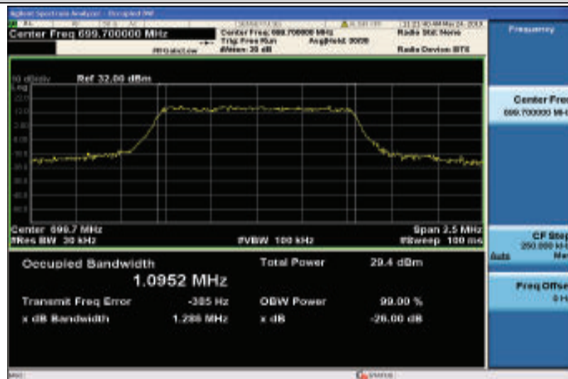
Band12-1.4MHz-16QAM-23017-6RB#0-1.0952
