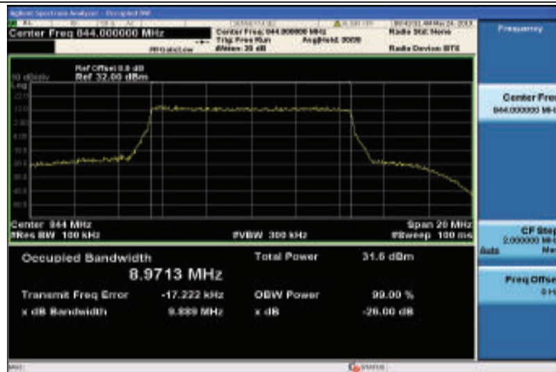
Band5-10MHz-QPSK-20600-50RB#0-8.9713
