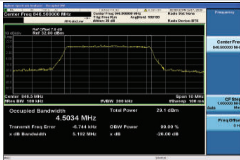
Band26-5MHz-16QAM-27015-25RB#0-4.5034
