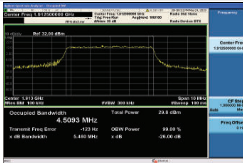
Band25-5MHz-16QAM-26665-25RB#0-4.5093
