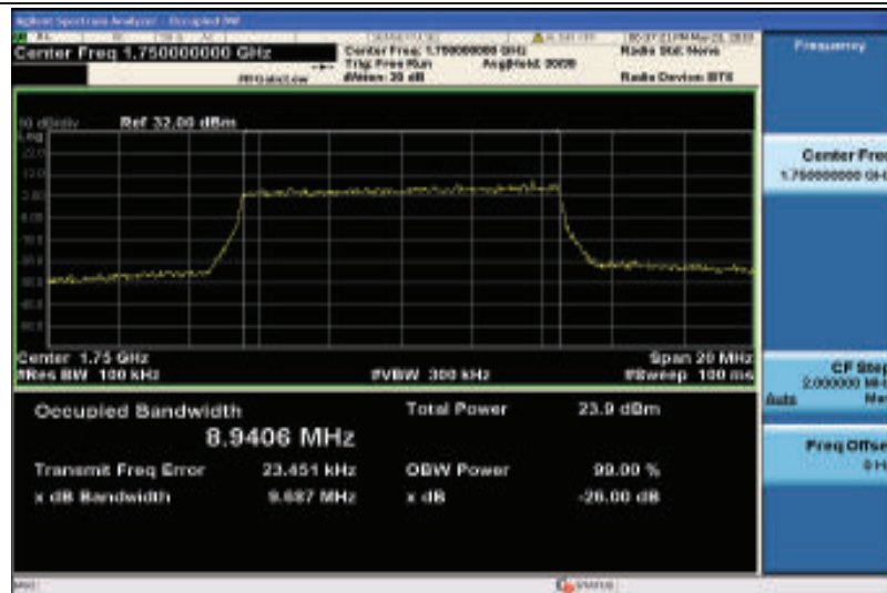
Band4-10MHz-16QAM-20350-50RB#0-8.9406
