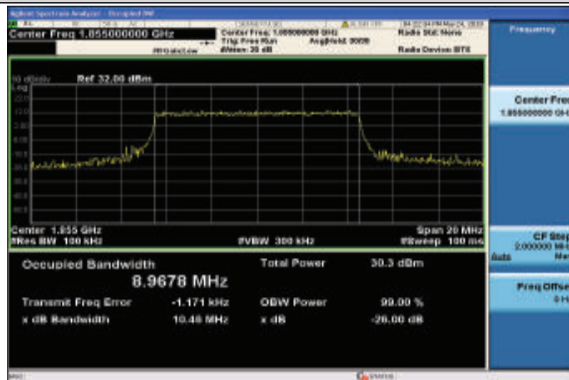
Band25-10MHz-QPSK-26090-50RB#0-8.9678
