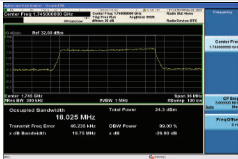
Band4-20MHz-16QAM-20300-100RB#0-18.025
