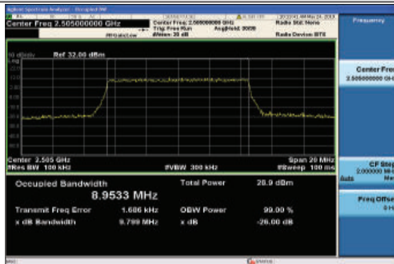
Band7-10MHz-16QAM-20800-50RB#0-8.9533
