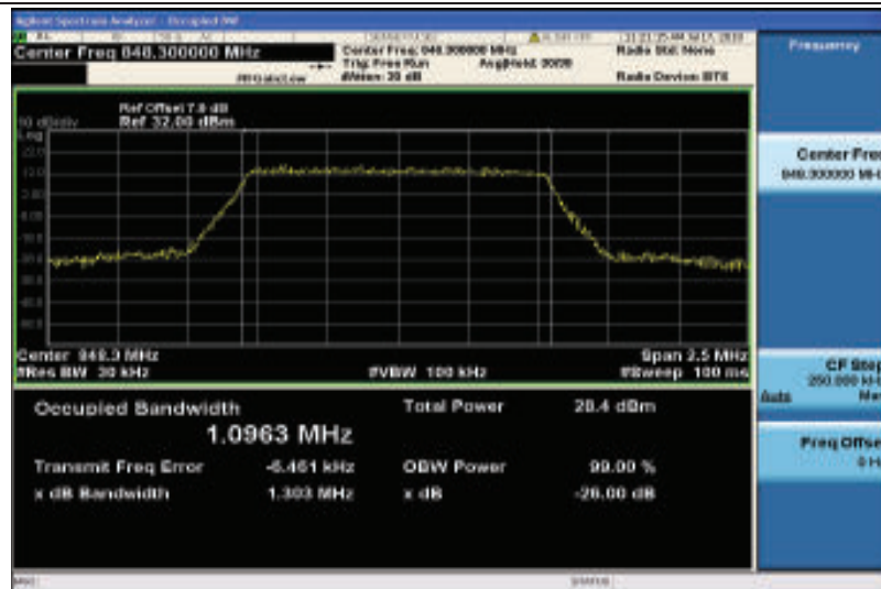
Band26-1.4MHz-16QAM-27033-6RB#0-1.0963
