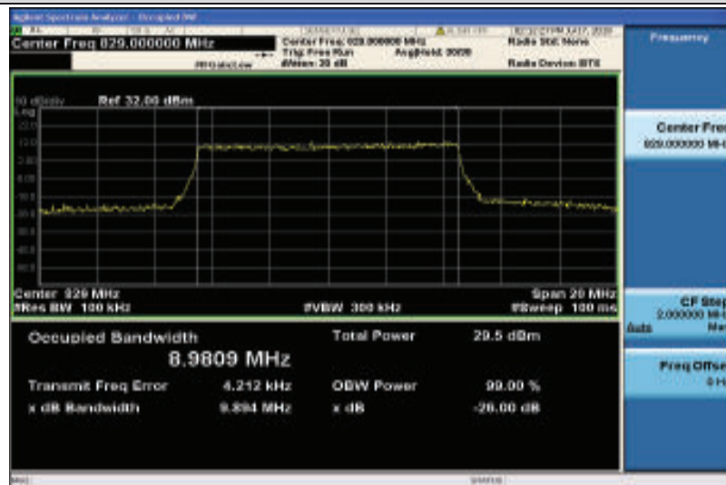
Band26-10MHz-16QAM-26840-50RB#0-8.9809
