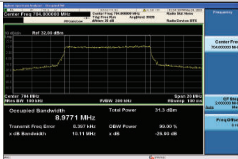
Band12-10MHz-QPSK-23060-50RB#0-8.9771
