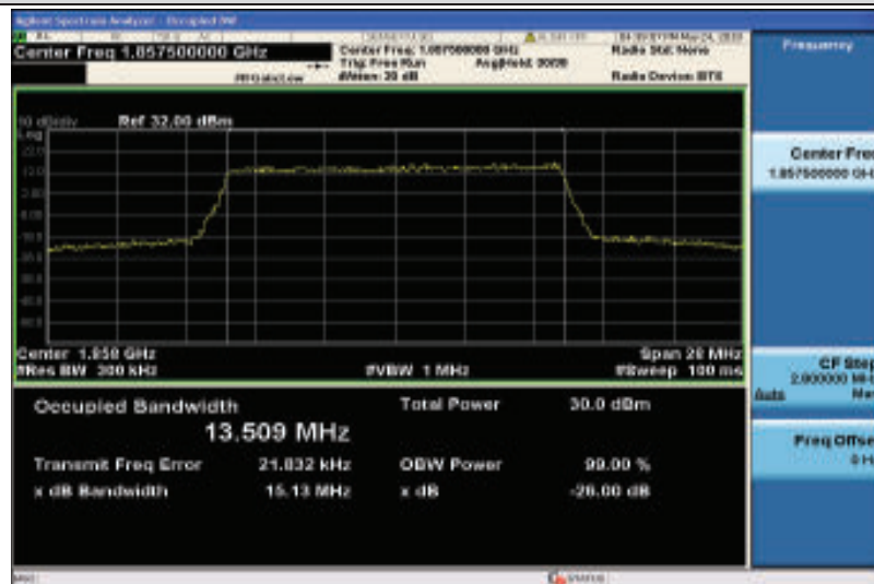
Band25-15MHz-16QAM-26115-75RB#0-13.509
