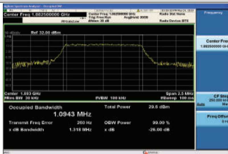
Band25-1.4MHz-QPSK-26365-6RB#0-1.0943
