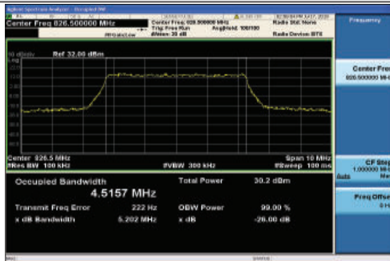
Band26-5MHz-QPSK-26815-25RB#0-4.5157
