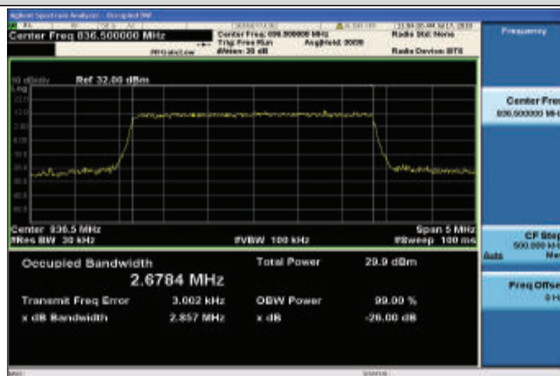
Band26-3MHz-QPSK-26915-15RB#0-2.6784
