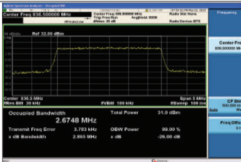
Band5-3MHz-QPSK-20525-15RB#0-2.6748
