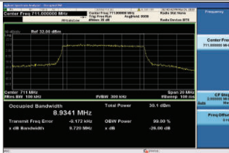
Band17-10MHz-16QAM-23800-50RB#0-8.9341
