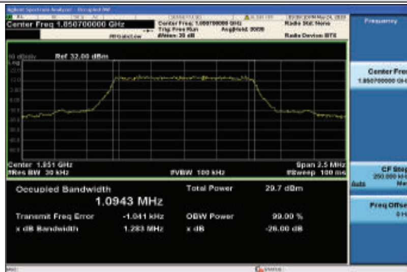
Band25-1.4MHz-QPSK-26047-6RB#0-1.0943
