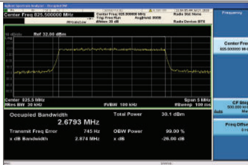
Band26-3MHz-QPSK-26805-15RB#0-2.6793
