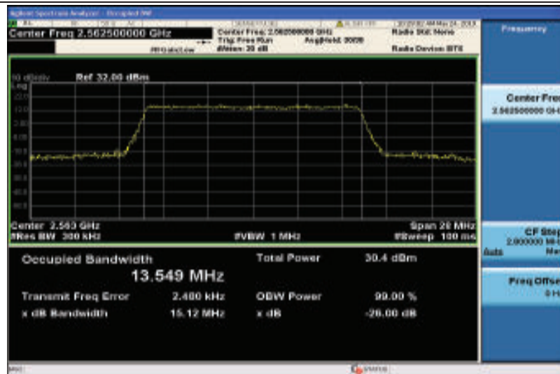
Band7-15MHz-QPSK-21375-75RB#0-13.549
