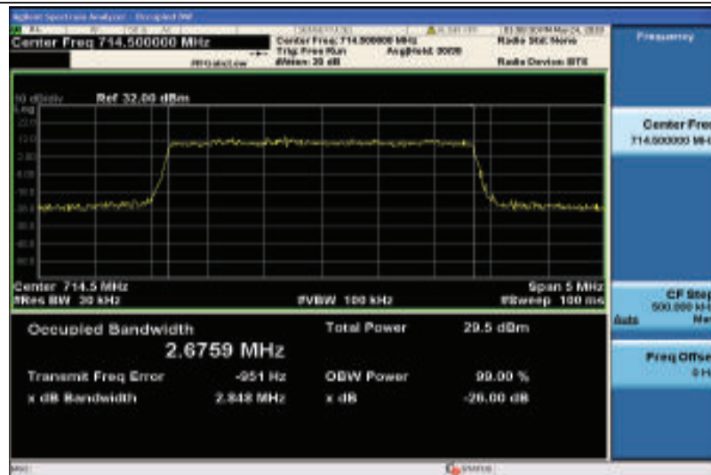
Band12-3MHz-16QAM-23165-15RB#0-2.6759
