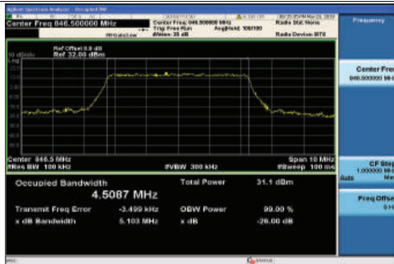
Band5-5MHz-16QAM-20625-25RB#0-4.5087
