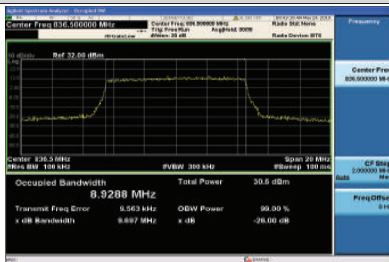
Band5-10MHz-16QAM-20525-50RB#0-8.9288
