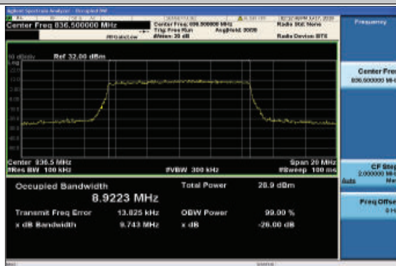
Band26-10MHz-16QAM-26915-50RB#0-8.9223
