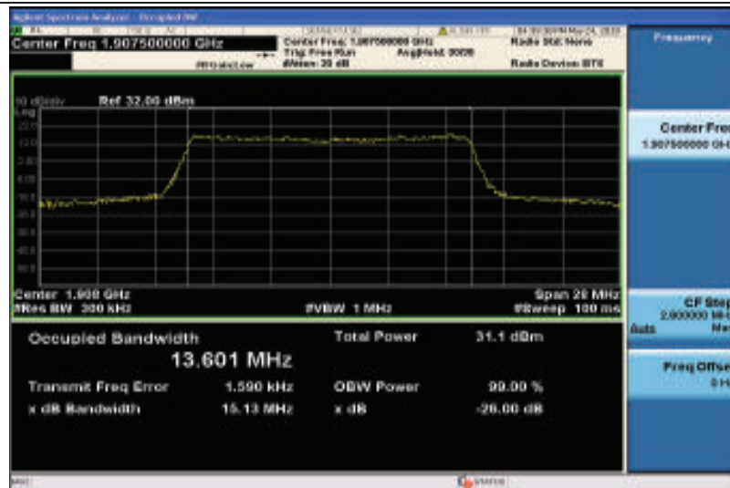
Band25-15MHz-QPSK-26615-75RB#0-13.601
