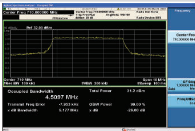
Band17-5MHz-QPSK-23790-25RB#0-4.5097
