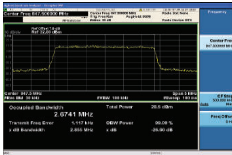
Band26-3MHz-16QAM-27025-15RB#0-2.6741
