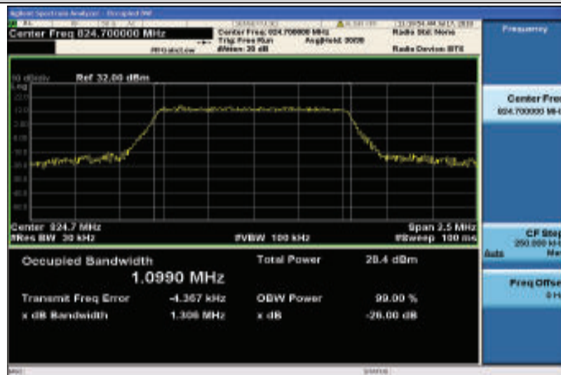
Band26-1.4MHz-16QAM-26797-6RB#0-1.0990
