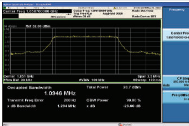
Band25-1.4MHz-16QAM-26047-6RB#0-1.0946
