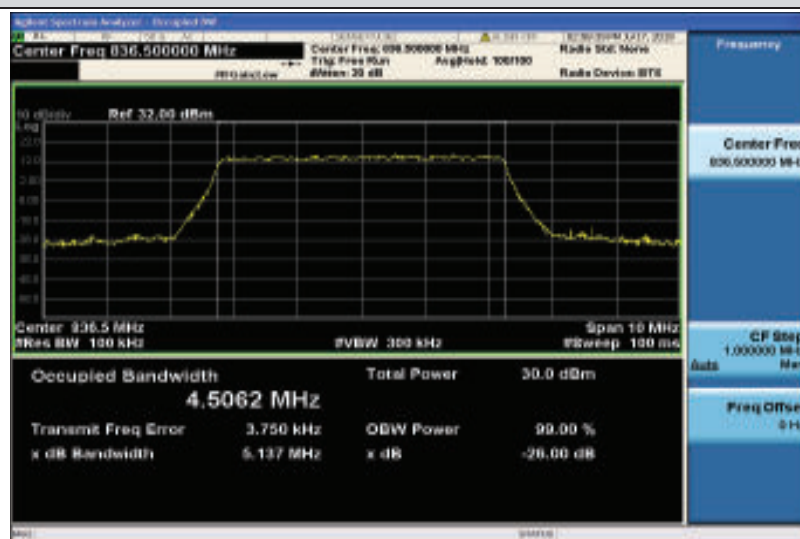
Band26-5MHz-QPSK-26915-25RB#0-4.5062
