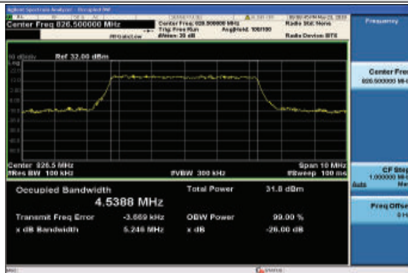
Band5-5MHz-QPSK-20425-25RB#0-4.5388
