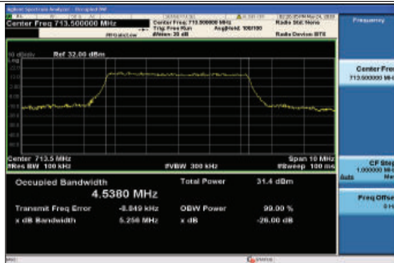
Band17-5MHz-QPSK-23825-25RB#0-4.5380
