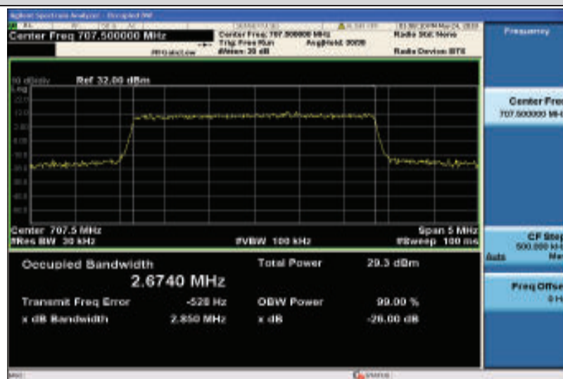
Band12-3MHz-16QAM-23095-15RB#0-2.6740
