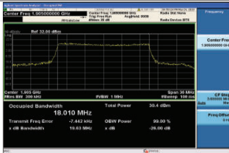
Band25-20MHz-16QAM-26590-100RB#0-18.010
