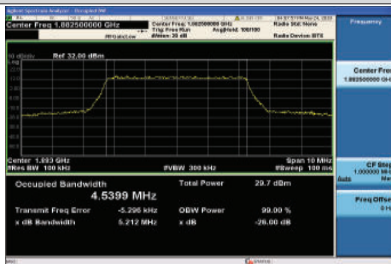
Band25-5MHz-16QAM-26365-25RB#0-4.5399
