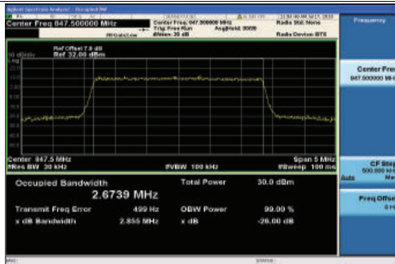
Band26-3MHz-QPSK-27025-15RB#0-2.6739
