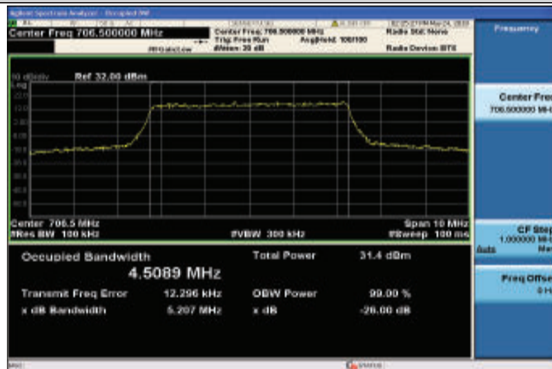
Band17-5MHz-QPSK-23755-25RB#0-4.5089
