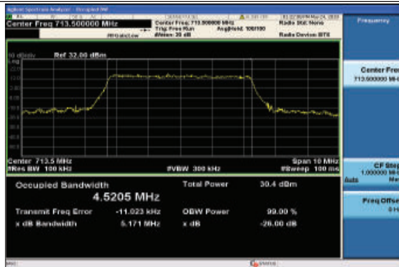
Band12-5MHz-16QAM-23155-25RB#0-4.5205
