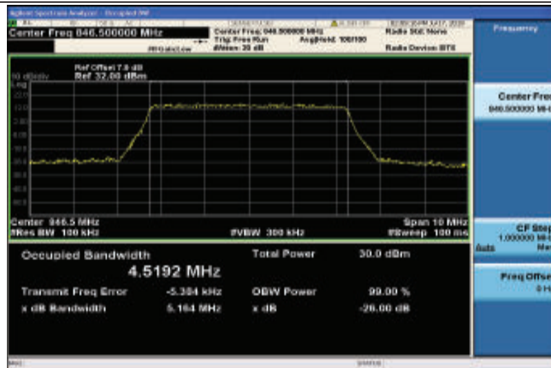
Band26-5MHz-QPSK-27015-25RB#0-4.5192
