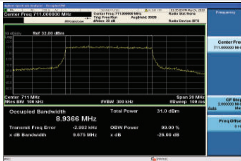
Band12-10MHz-QPSK-23130-50RB#0-8.9366
