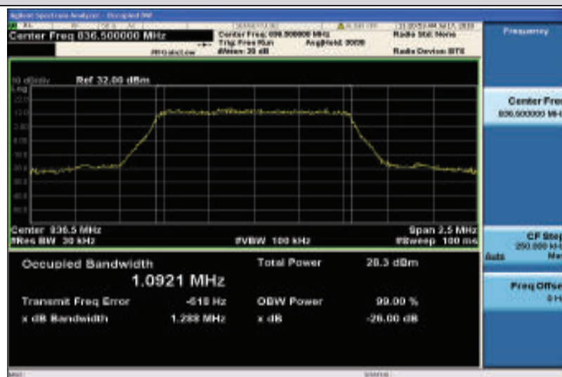
Band26-1.4MHz-16QAM-26915-6RB#0-1.0921
