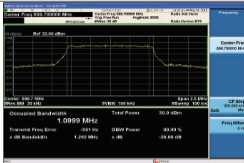
Band12-1.4MHz-QPSK-23017-6RB#0-1.0999
