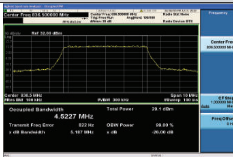
Band26-5MHz-16QAM-26915-25RB#0-4.5227
