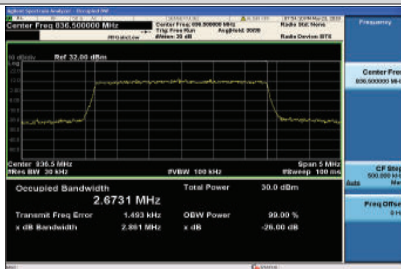
Band5-3MHz-16QAM-20525-15RB#0-2.6731
