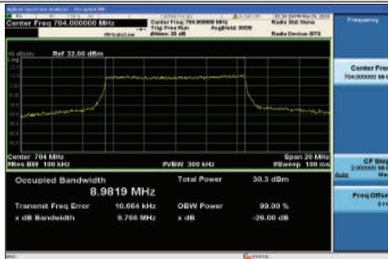
Band12-10MHz-16QAM-23060-50RB#0-8.9819
