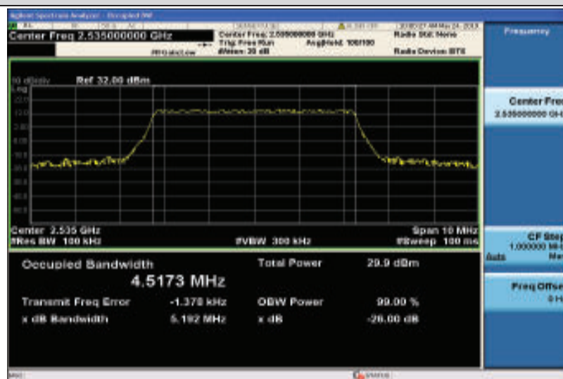
Band7-5MHz-QPSK-21100-25RB#0-4.5173
