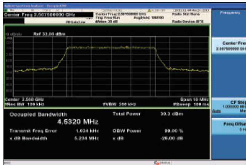
Band7-5MHz-QPSK-21425-25RB#0-4.5320
