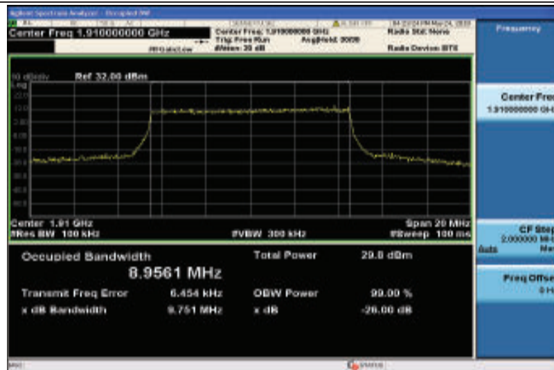
Band25-10MHz-16QAM-26640-50RB#0-8.9561
