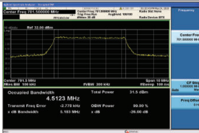
Band12-5MHz-QPSK-23035-25RB#0-4.5123
