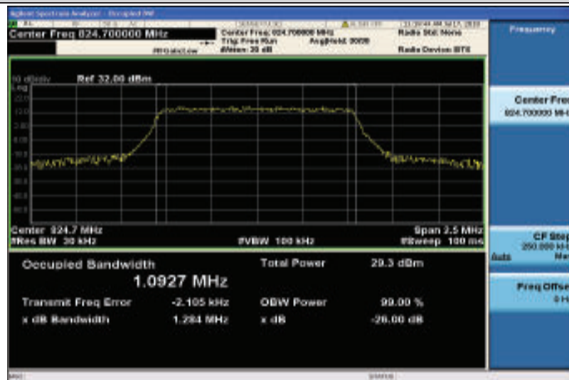
Band26-1.4MHz-QPSK-26797-6RB#0-1.0927
