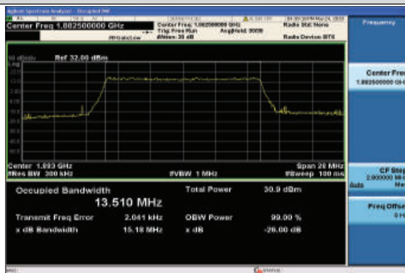
Band25-15MHz-QPSK-26365-75RB#0-13.510
