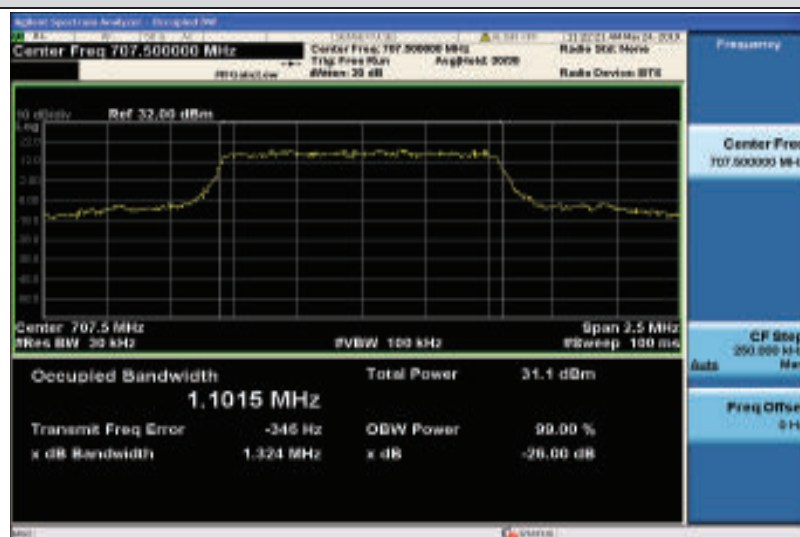
Band12-1.4MHz-QPSK-23095-6RB#0-1.1015
