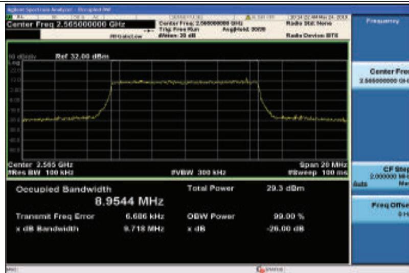
Band7-10MHz-16QAM-21400-50RB#0-8.9544
