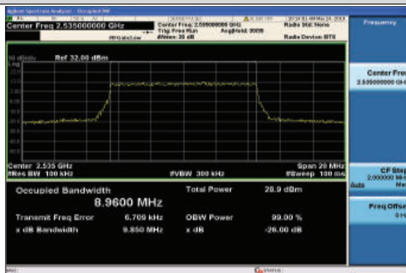
Band7-10MHz-16QAM-21100-50RB#0-8.9600
