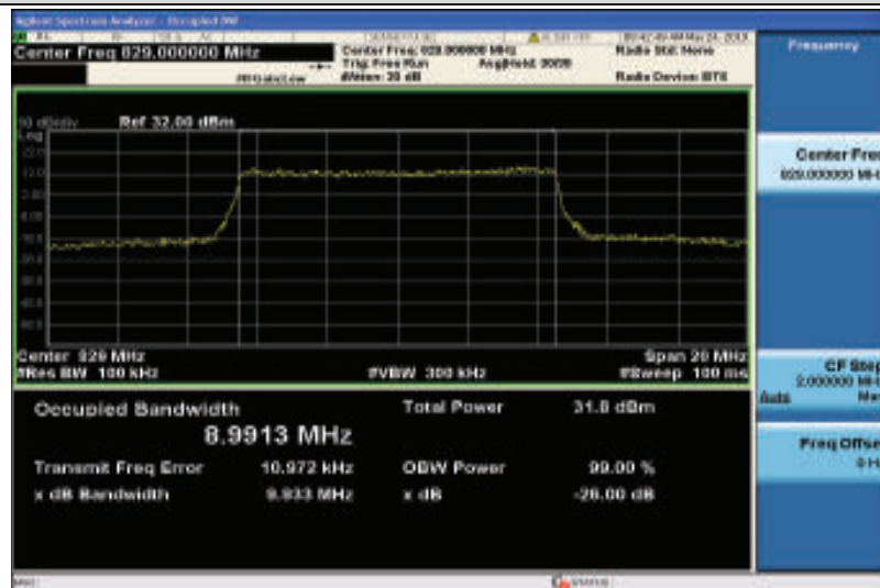
Band5-10MHz-QPSK-20450-50RB#0-8.9913
