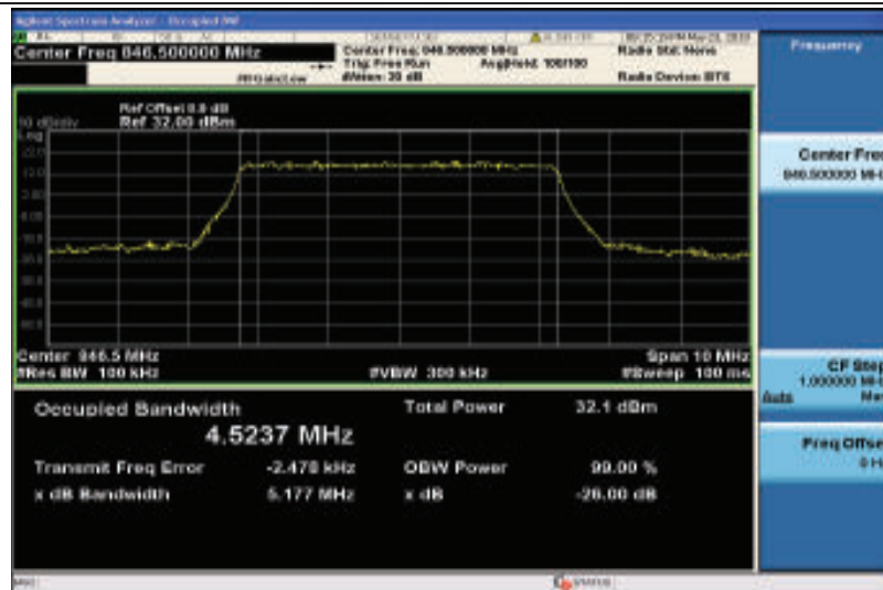
Band5-5MHz-QPSK-20625-25RB#0-4.5237
