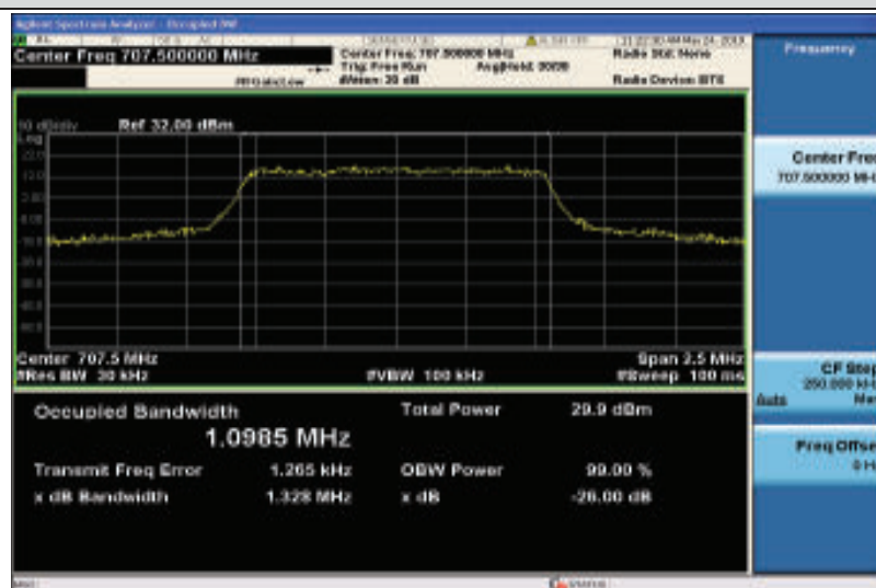
Band12-1.4MHz-16QAM-23095-6RB#0-1.0985
