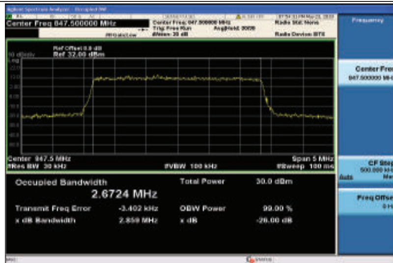
Band5-3MHz-16QAM-20635-15RB#0-2.6724
