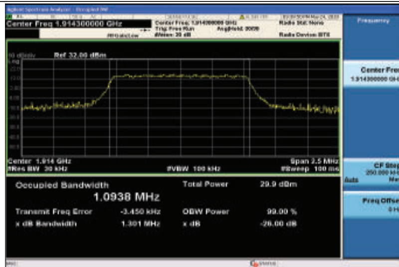
Band25-1.4MHz-QPSK-26683-6RB#0-1.0938
