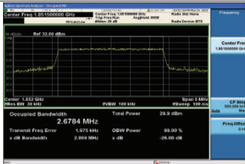
Band25-3MHz-QPSK-26055-15RB#0-2.6784
