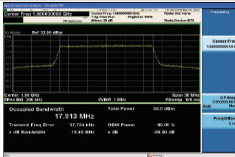
Band25-20MHz-16QAM-26140-100RB#0-17.913
