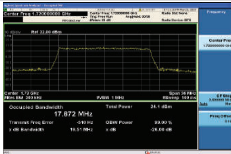
Band4-20MHz-16QAM-20050-100RB#0-17.872
