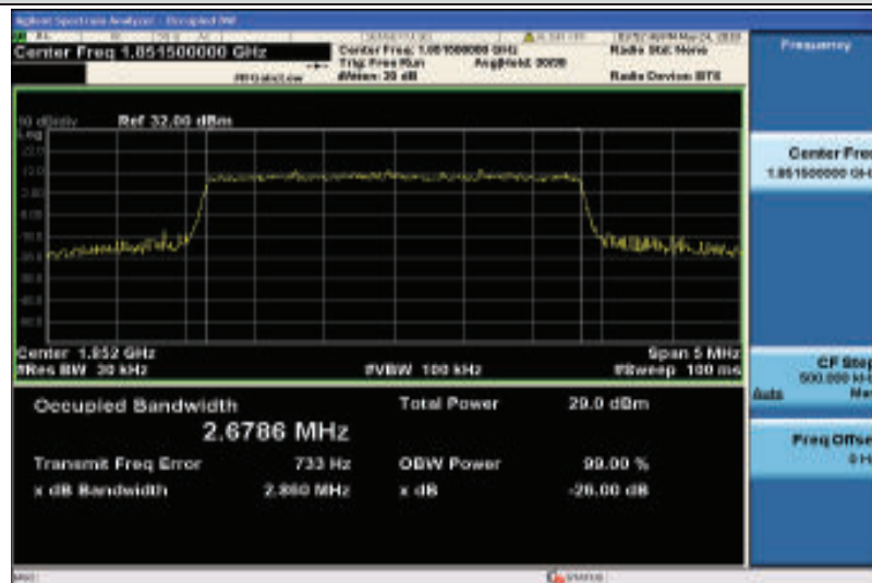
Band25-3MHz-16QAM-26055-15RB#0-2.6786
