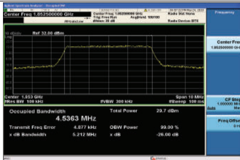
Band25-5MHz-16QAM-26065-25RB#0-4.5363
