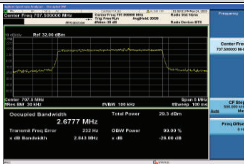
Band12-3MHz-QPSK-23095-15RB#0-2.6777
