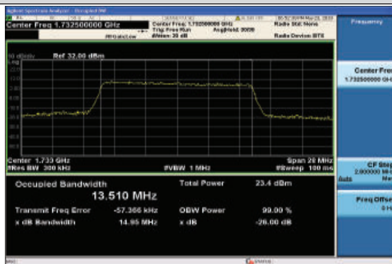
Band4-15MHz-16QAM-20175-75RB#0-13.510
