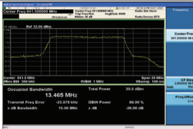
Band26-15MHz-QPSK-26965-75RB#0-13.465
