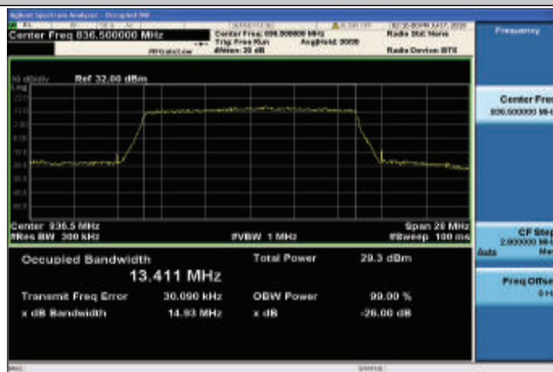
Band26-15MHz-16QAM-26915-75RB#0-13.411
