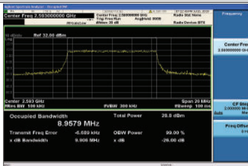
Band41-10MHz-QPSK-40620-50RB#0-8.9579
