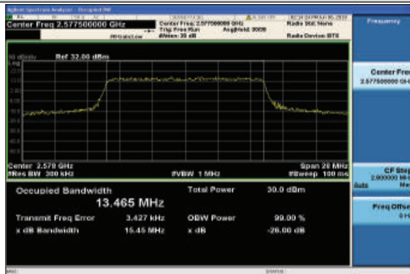
Band38-15MHz-QPSK-37825-75RB#0-13.465
