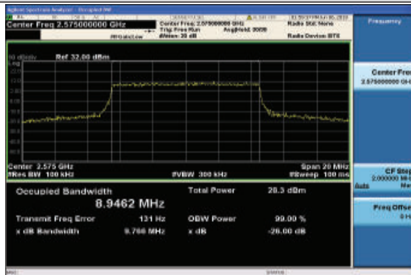
Band38-10MHz-16QAM-37800-50RB#0-8.9462
