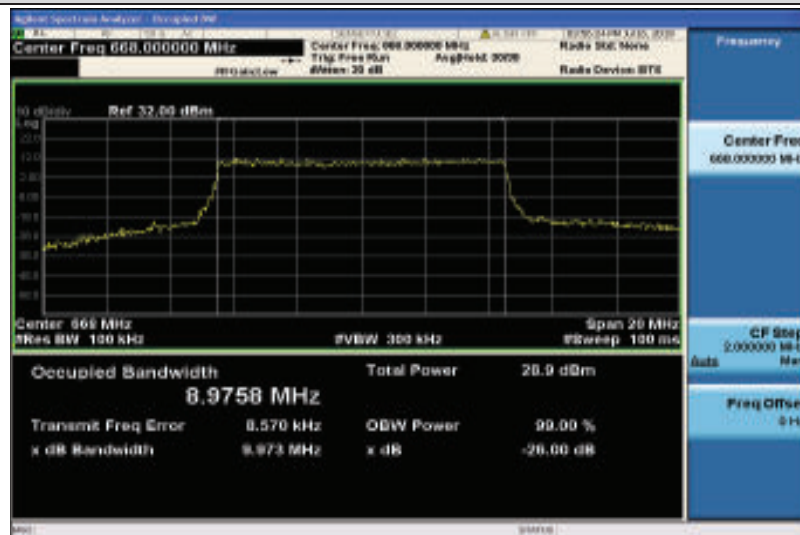
Band71-10MHz-16QAM-133172-50RB#0-8.9758
