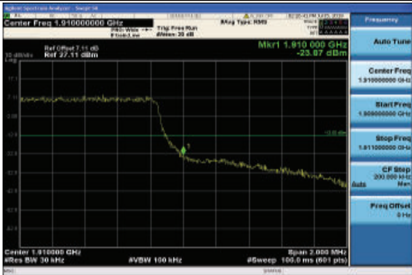
Band2-1.4MHz-QPSK-19193-6RB#0
