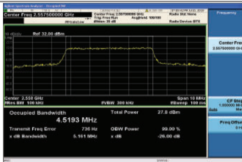
Band41-5MHz-16QAM-40265-25RB#0-4.5193
