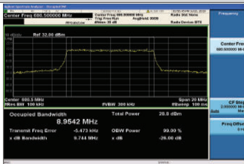
Band71-10MHz-16QAM-133297-50RB#0-8.9542
