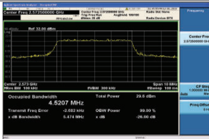
Band38-5MHz-QPSK-37775-25RB#0-4.5207
