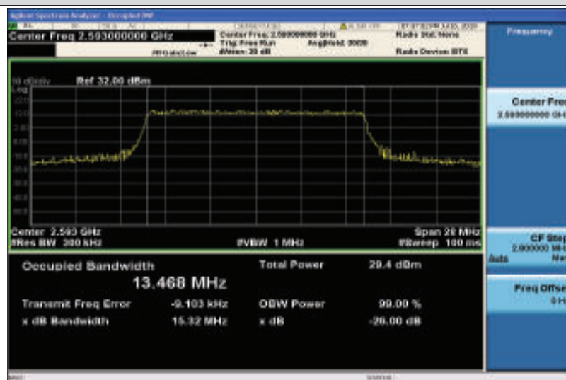
Band41-15MHz-QPSK-40620-75RB#0-13.468
