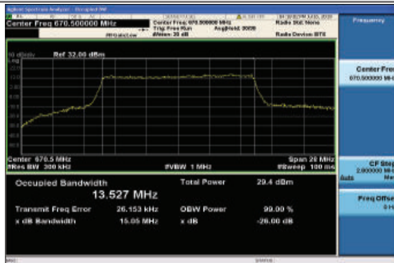
Band71-15MHz-16QAM-133197-75RB#0-13.527
