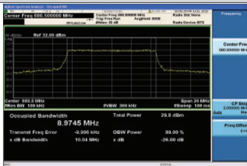
Band71-10MHz-QPSK-133297-50RB#0-8.9745
