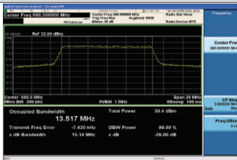
Band71-15MHz-QPSK-133297-75RB#0-13.517
