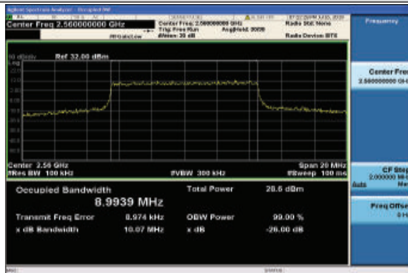
Band41-10MHz-QPSK-40290-50RB#0-8.9939
