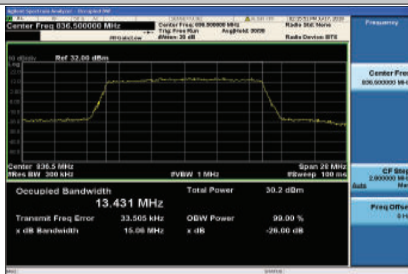
Band26-15MHz-QPSK-26915-75RB#0-13.431
