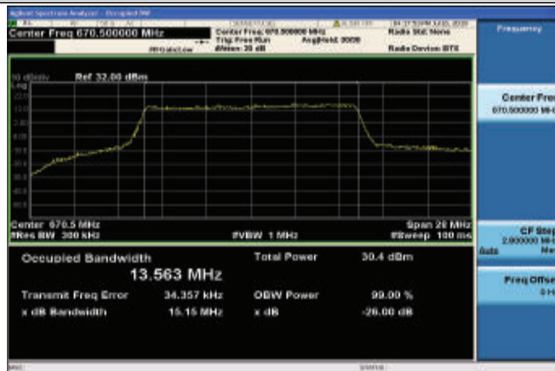
Band71-15MHz-QPSK-133197-75RB#0-13.563
