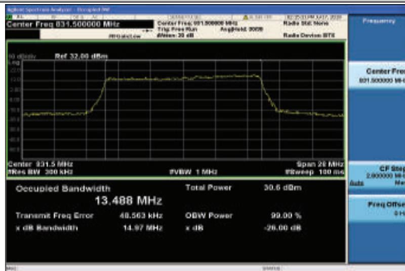
Band26-15MHz-QPSK-26915-75RB#0-13.488
