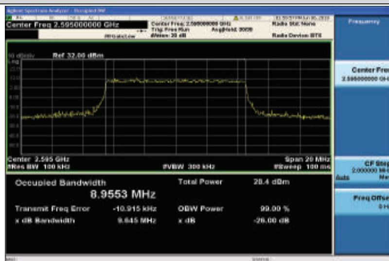
Band38-10MHz-16QAM-38000-50RB#0-8.9553
