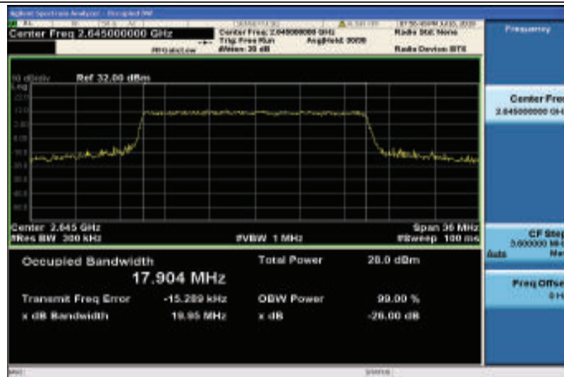
Band41-20MHz-16QAM-41140-100RB#0-17.904
