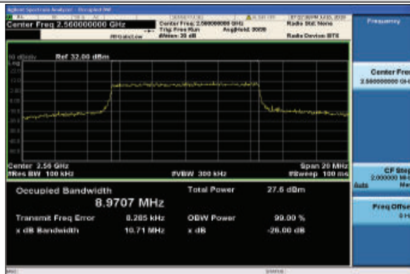
Band41-10MHz-16QAM-40290-50RB#0-8.9707
