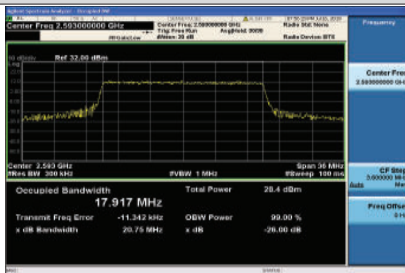
Band41-20MHz-16QAM-40620-100RB#0-17.917
