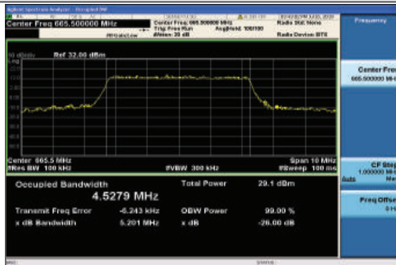
Band71-5MHz-16QAM-133147-25RB#0-4.5279
