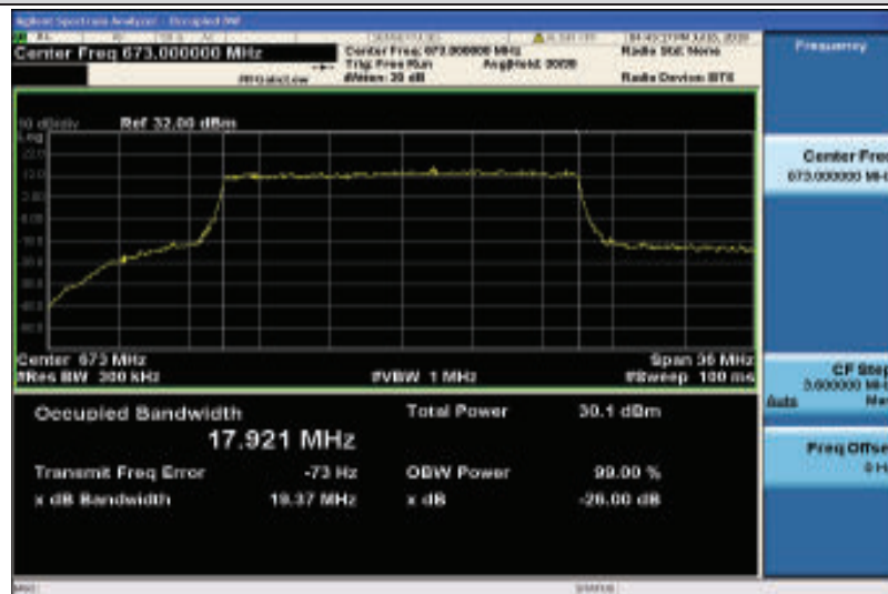
Band71-20MHz-QPSK-133222-100RB#0-17.921
