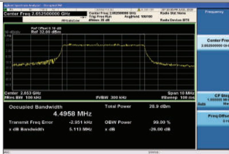
Band41-5MHz-QPSK-41215-25RB#0-4.4958
