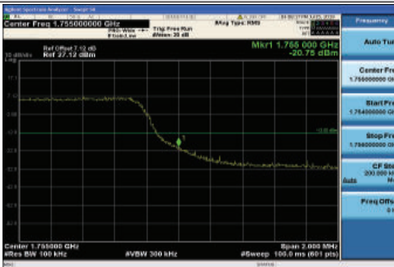
Band4-5MHz-QPSK-20375-25RB#0
