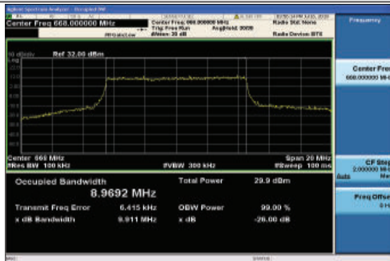
Band71-10MHz-QPSK-133172-50RB#0-8.9692
