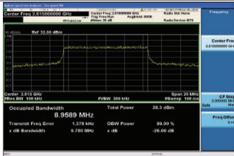
Band38-10MHz-16QAM-38200-50RB#0-8.9589
