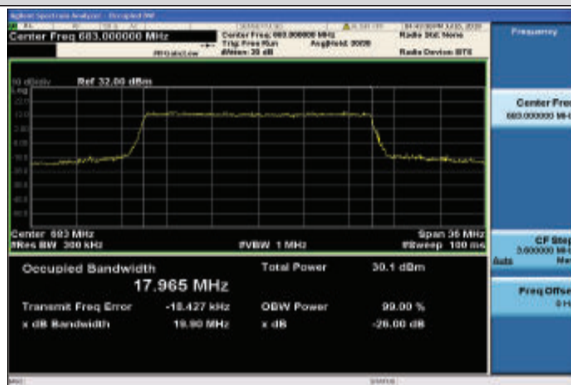
Band71-20MHz-QPSK-133322-100RB#0-17.965
