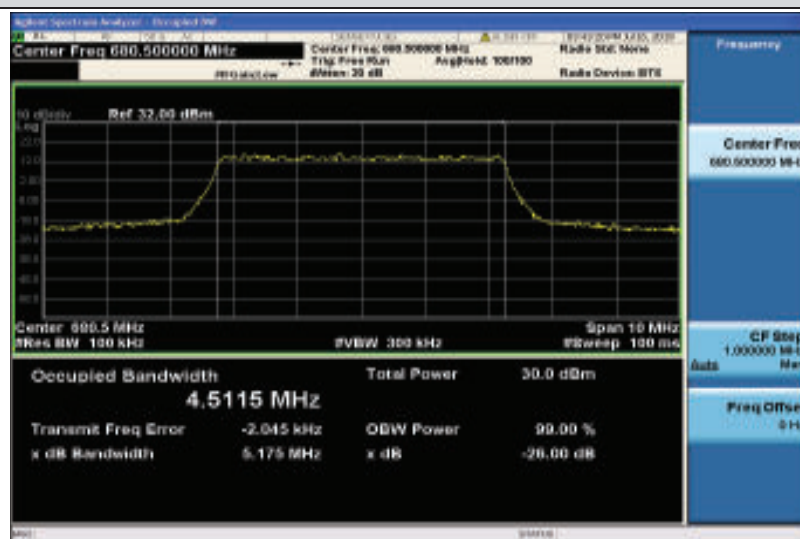
Band71-5MHz-QPSK-133297-25RB#0-4.5115
