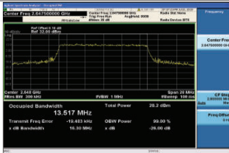
Band41-15MHz-QPSK-41165-75RB#0-13.517
