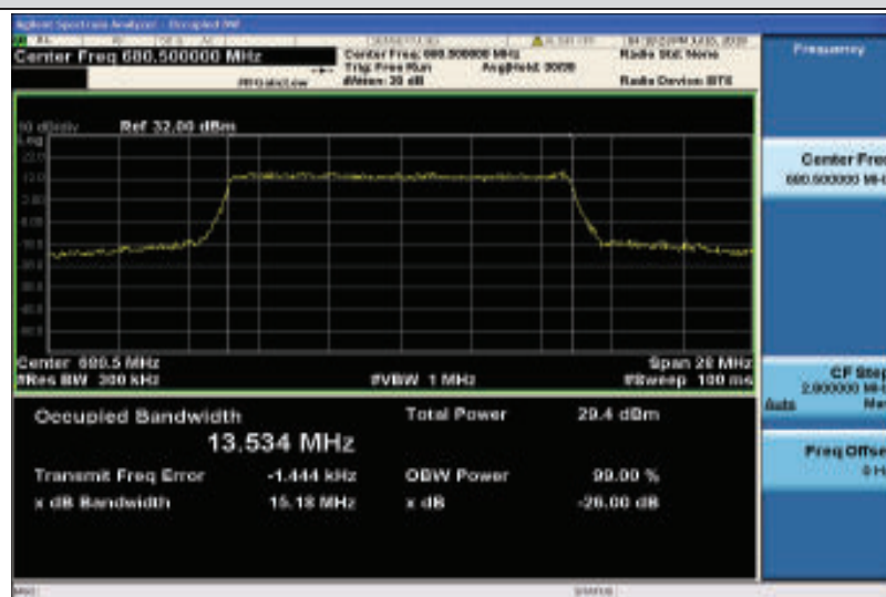
Band71-15MHz-16QAM-133297-75RB#0-13.534
