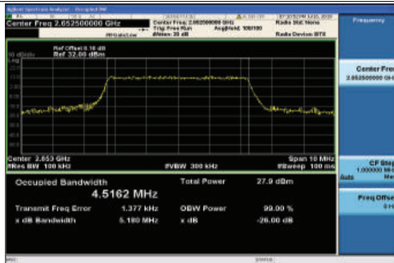
Band41-5MHz-16QAM-41215-25RB#0-4.5162
