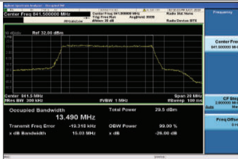
Band26-15MHz-16QAM-26965-75RB#0-13.490
