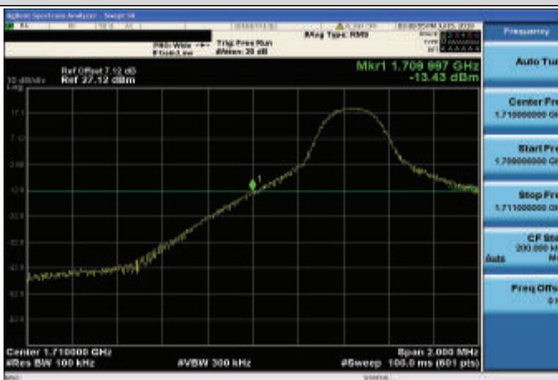
Band4-5MHz-16QAM-19975-1RB#0
