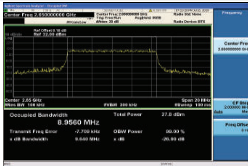
Band41-10MHz-16QAM-41190-50RB#0-8.9560
