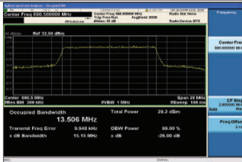
Band71-15MHz-16QAM-133397-75RB#0-13.506
