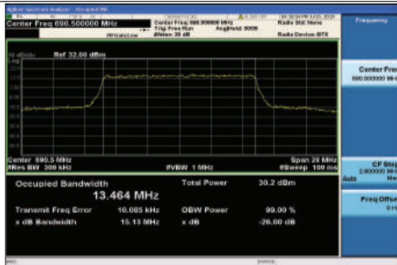
Band71-15MHz-QPSK-133397-75RB#0-13.464
