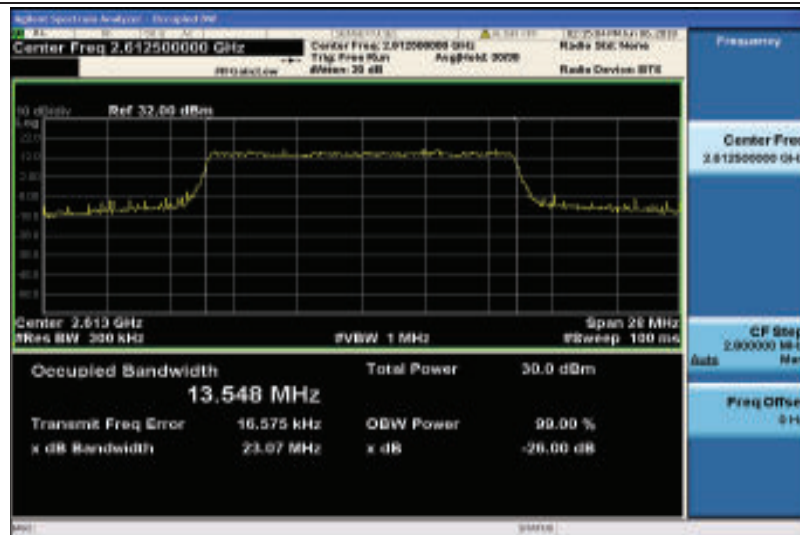
Band38-15MHz-QPSK-38175-75RB#0-13.548
