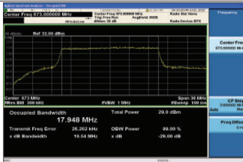
Band71-20MHz-16QAM-133222-100RB#0-17.948
