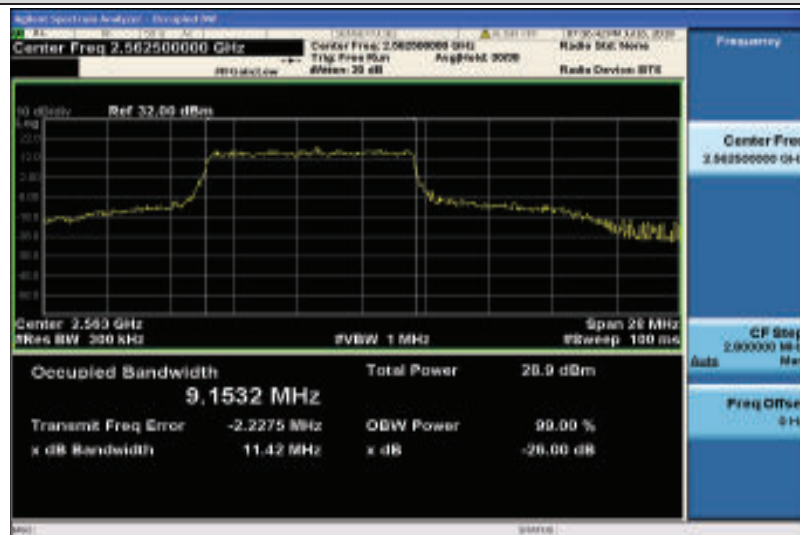
Band41-15MHz-QPSK-40315-75RB#0-9.1532
