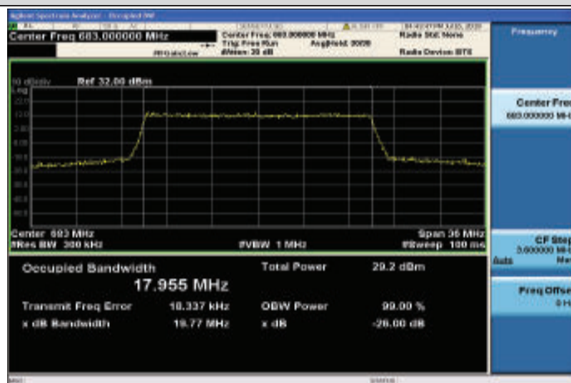
Band71-20MHz-16QAM-133322-100RB#0-17.955
