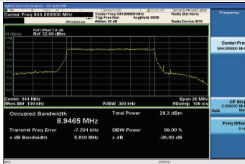
Band26-10MHz-16QAM-26990-50RB#0-8.9465
