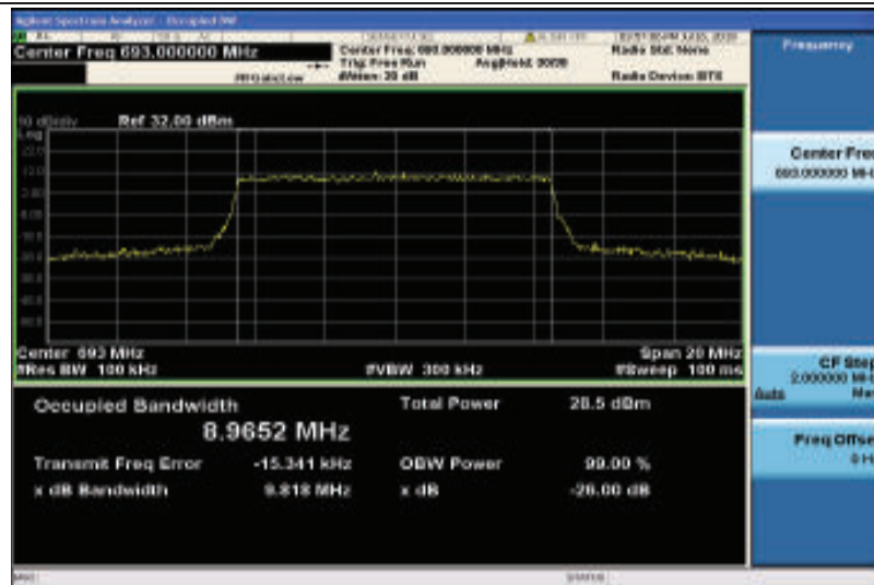
Band71-10MHz-16QAM-133422-50RB#0-8.9652
