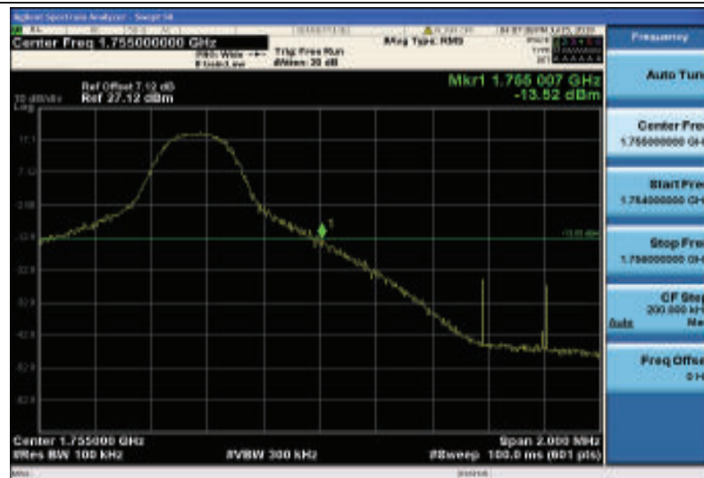
Band4-5MHz-QPSK-20375-1RB#24
