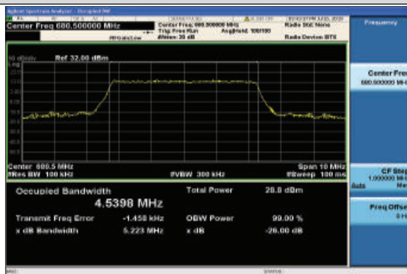
Band71-5MHz-16QAM-133297-25RB#0-4.5398
