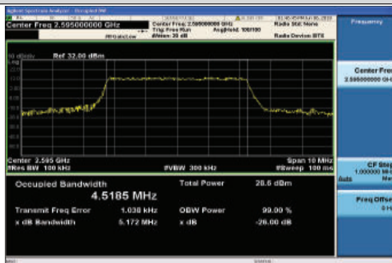
Band38-5MHz-16QAM-38000-25RB#0-4.5185
