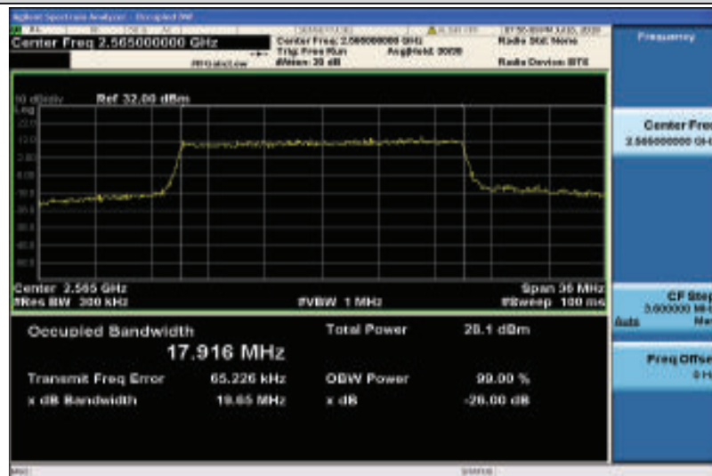
Band41-20MHz-16QAM-40340-100RB#0-17.916
