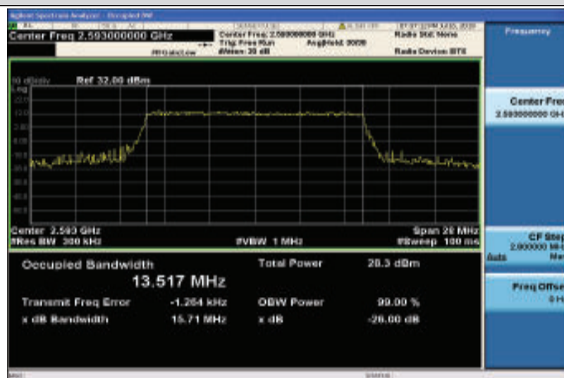
Band41-15MHz-16QAM-40620-75RB#0-13.517
