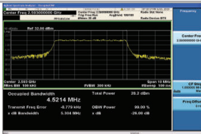
Band41-5MHz-16QAM-40620-25RB#0-4.5214
