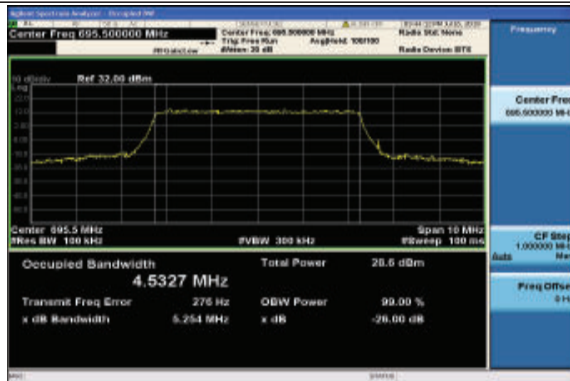
Band71-5MHz-16QAM-133447-25RB#0-4.5327
