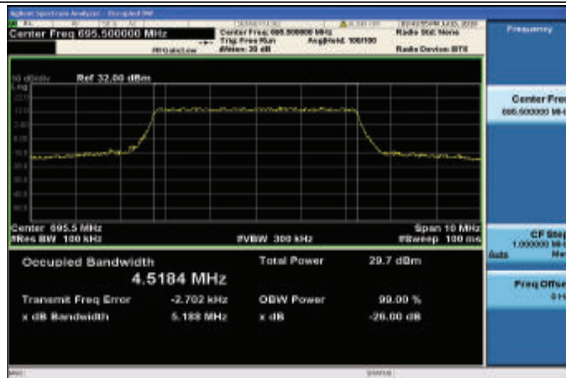
Band71-5MHz-QPSK-133447-25RB#0-4.5184
