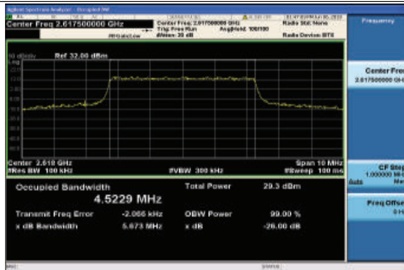
Band38-5MHz-QPSK-38225-25RB#0-4.5229
