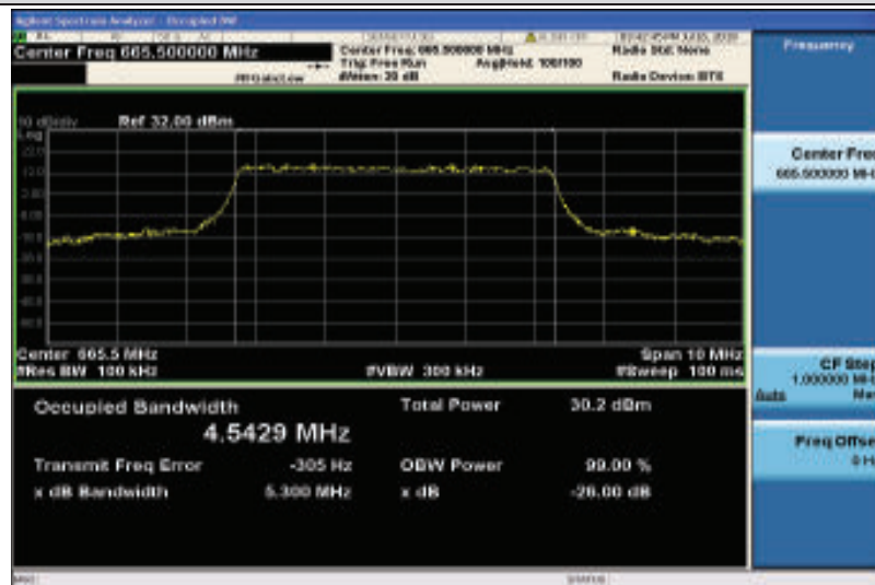
Band71-5MHz-QPSK-133147-25RB#0-4.5429
