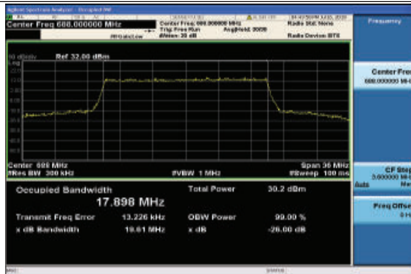
Band71-20MHz-QPSK-133372-100RB#0-17.898
