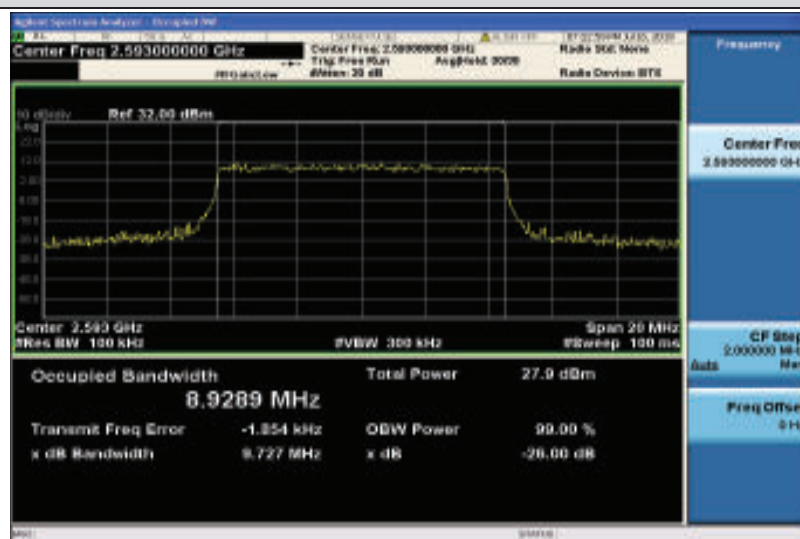
Band41-10MHz-16QAM-40620-50RB#0-8.9289
