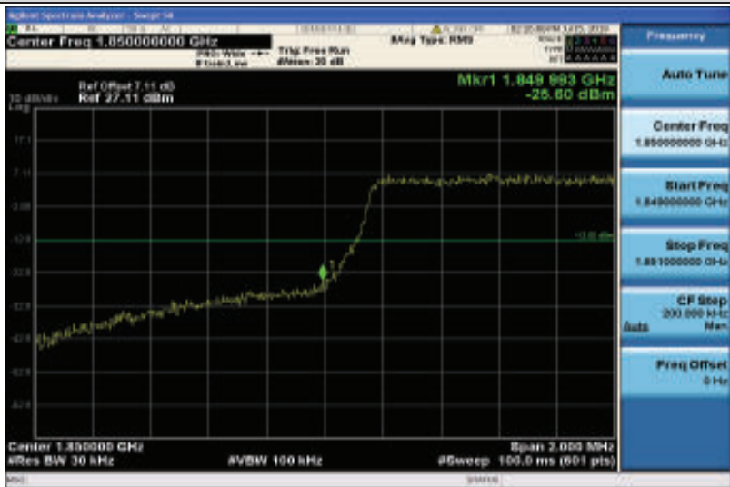
Band2-1.4MHz-16QAM-18607-6RB#0
