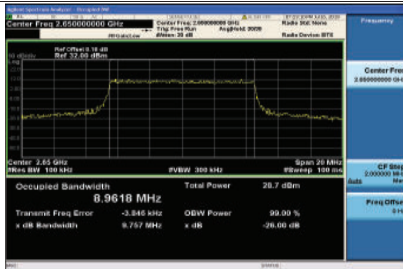
Band41-10MHz-QPSK-41190-50RB#0-8.9618
