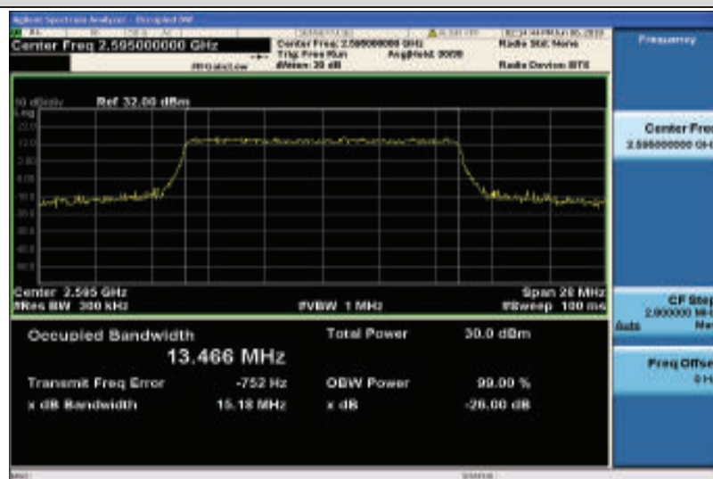
Band38-15MHz-QPSK-38000-75RB#0-13.466
