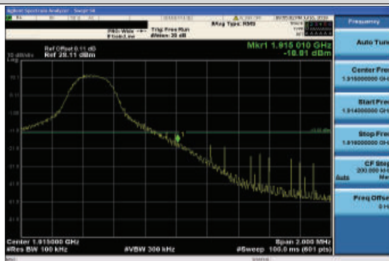
Band25-5MHz-16QAM-26665-1RB#24
