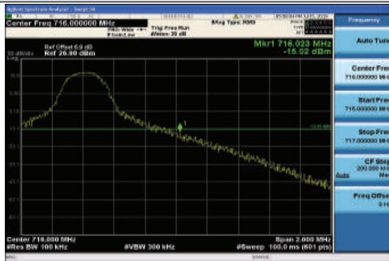
Band12-10MHz-16QAM-23130-1RB#49
