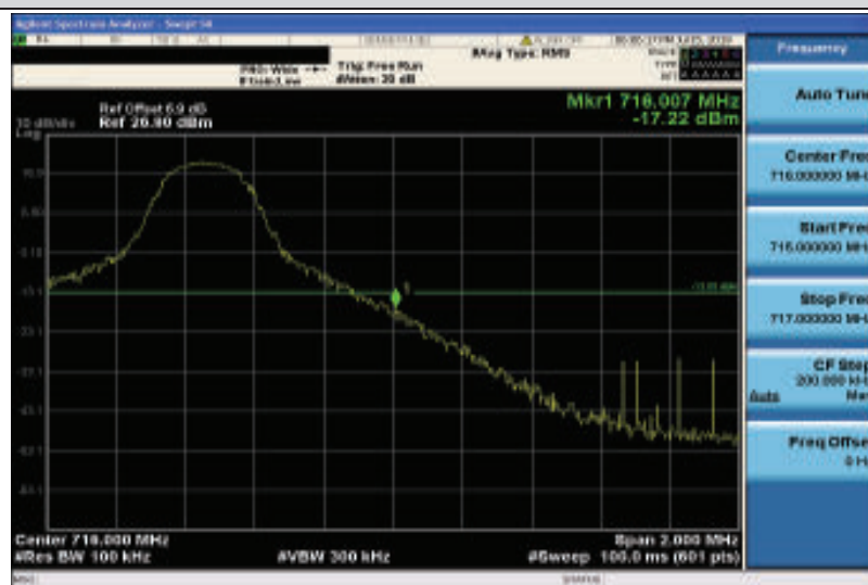
Band17-5MHz-QPSK-23825-1RB#24
