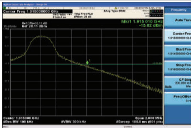
Band25-10MHz-16QAM-26640-1RB#49
