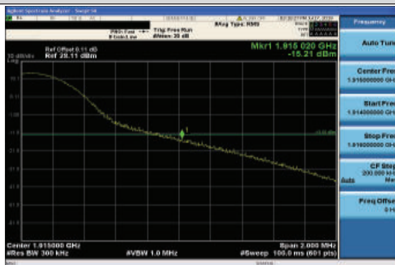
Band25-15MHz-QPSK-26615-1RB#74
