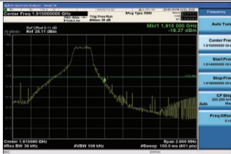
Band25-3MHz-16QAM-26675-1RB#14
