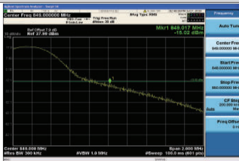
Band26-15MHz-QPSK-26965-1RB#74
