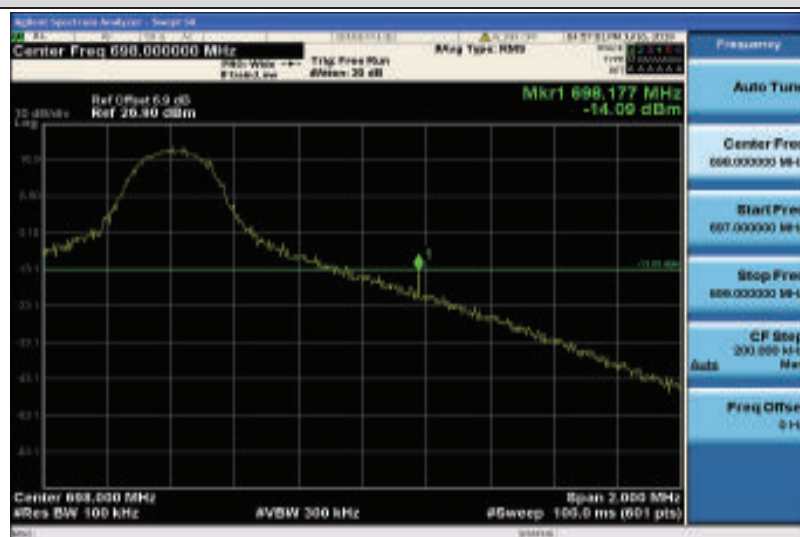
Band71-10MHz-16QAM-133422-1RB#49
