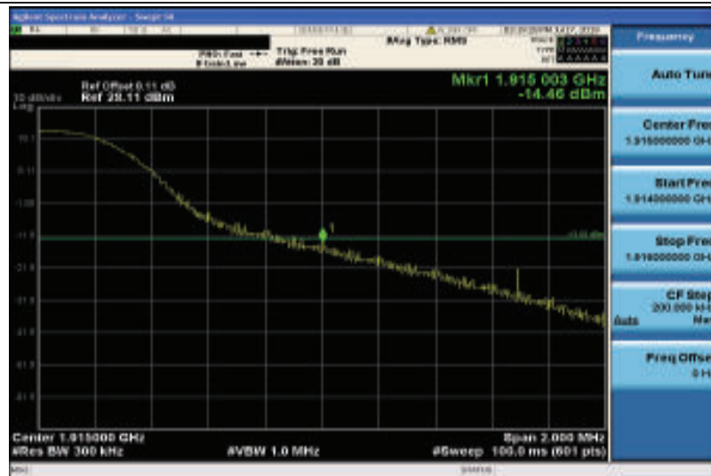
Band25-15MHz-16QAM-26615-1RB#74
