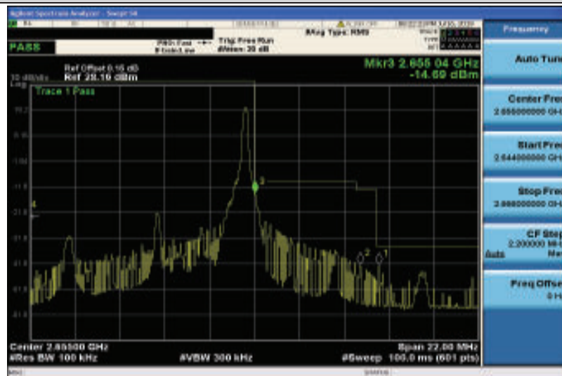
Band41-5MHz-16QAM-41215-1RB#24
