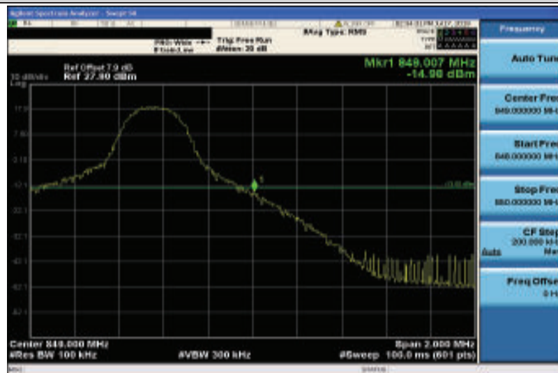
Band26-5MHz-QPSK-27015-1RB#24
