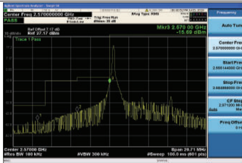
Band38-10MHz-QPSK-37800-1RB#0
