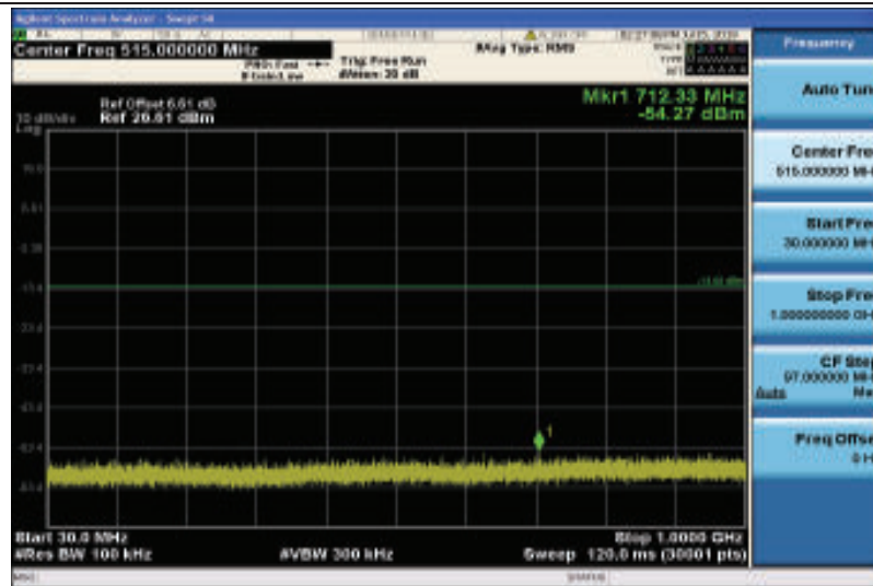
Band2-1.4MHz-QPSK-18607-1RB#0-Range1:30~1000MHz
