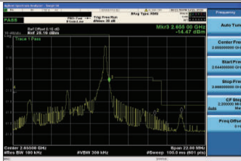
Band41-5MHz-QPSK-41215-1RB#24
