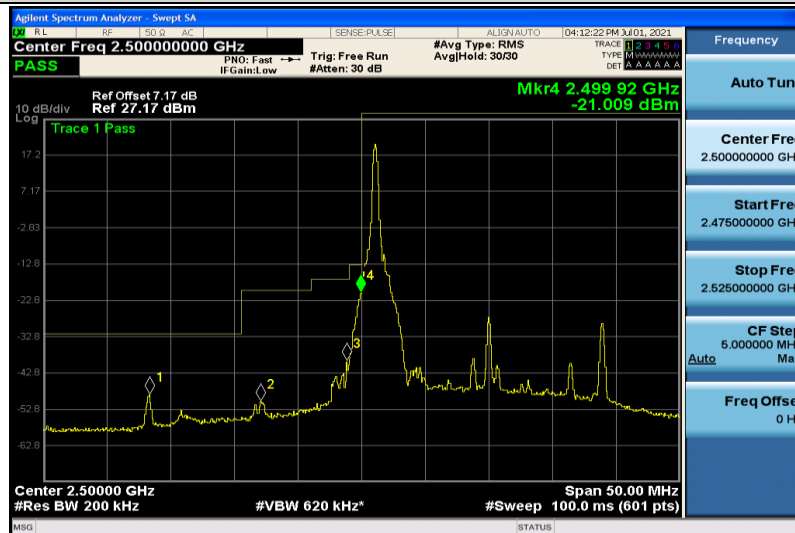
Band7-20MHz-16QAM-20850-1RB#0
