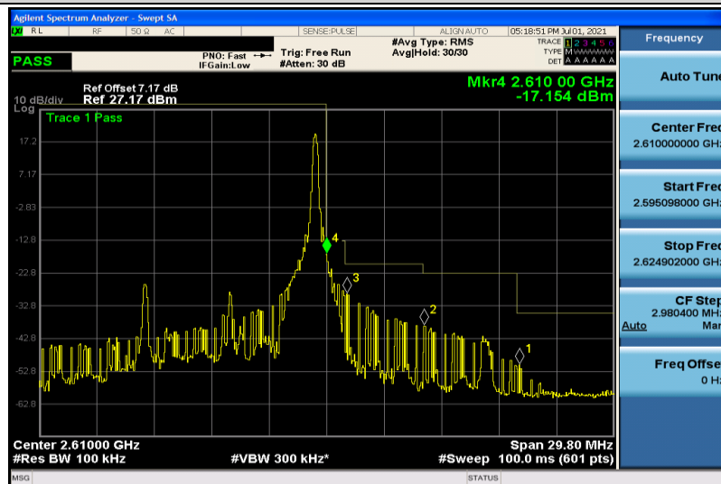
Band41-10MHz-QPSK-40740-1RB#49
