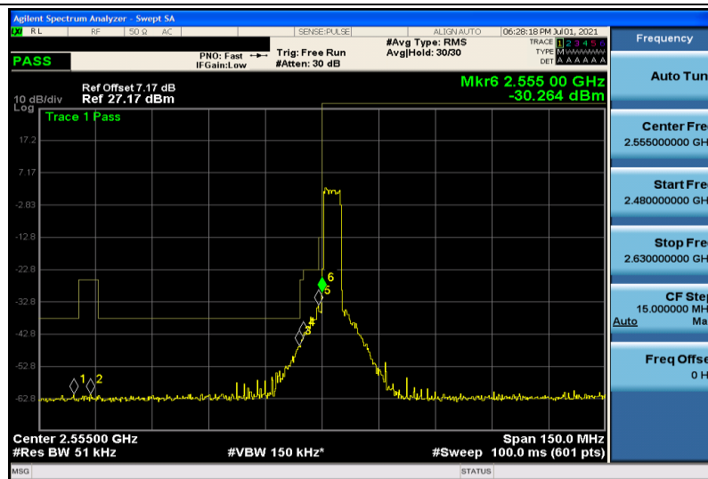
Band41-5MHz-16QAM-40265-25RB#0
