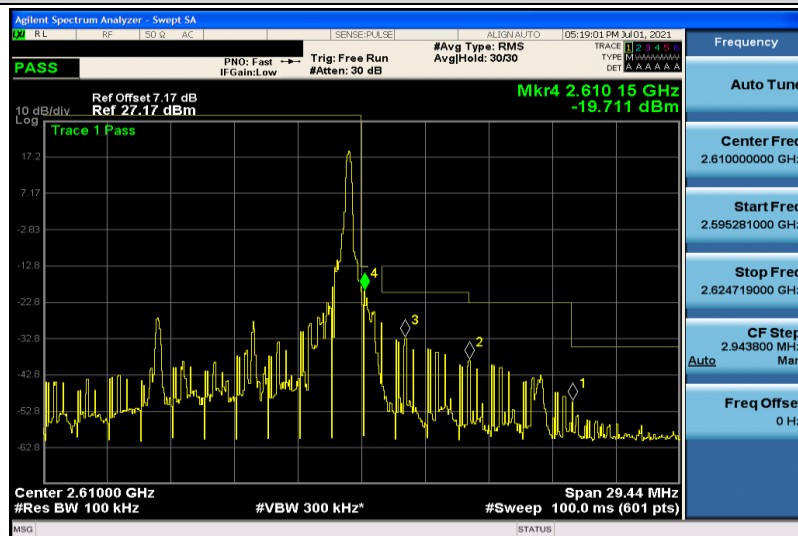
Band41-10MHz-16QAM-40740-1RB#49
