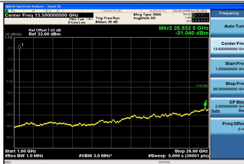
Band4-1.4MHz-16QAM-19957-1RB#0-1000~26000MHz
