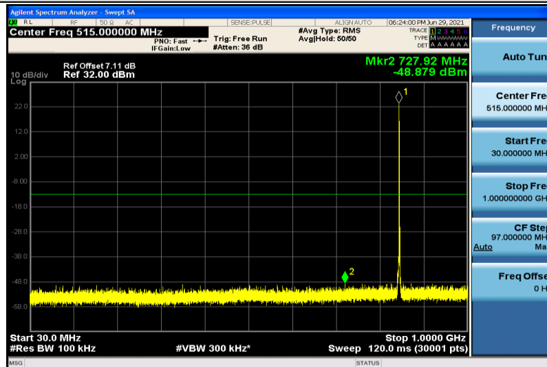
Band5-1.4MHz-QPSK-20643-1RB#0-30~1000MHz
