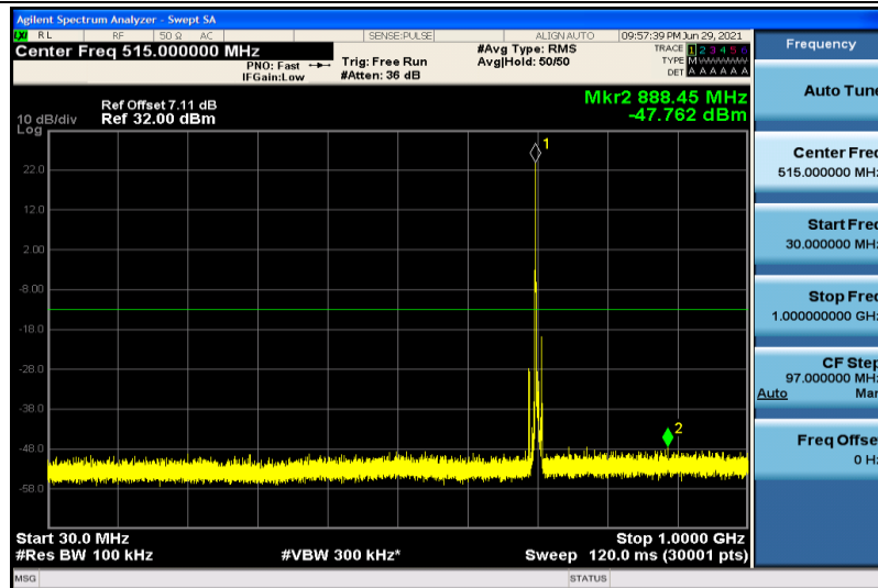
Band12-5MHz-16QAM-23095-1RB#0-30~1000MHz
