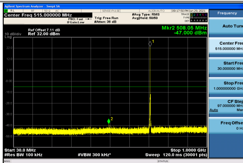
Band12-1.4MHz-QPSK-23173-1RB#0-30~1000MHz
