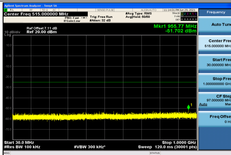
Band38-5MHz-QPSK-37775-1RB#0-30~1000MHz
