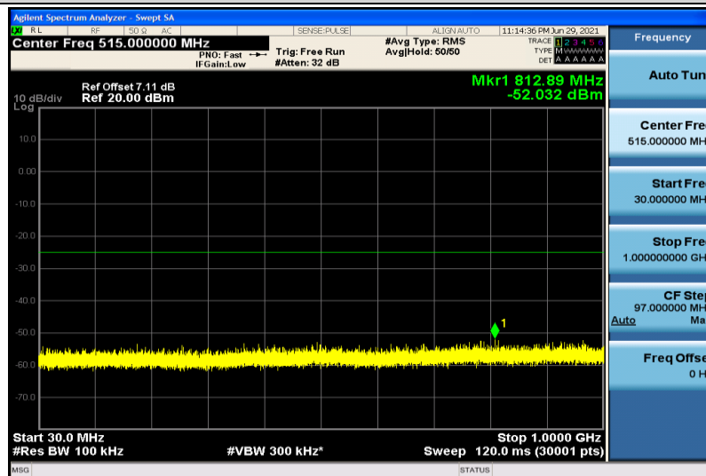
Band38-5MHz-16QAM-37775-1RB#0-30~1000MHz
