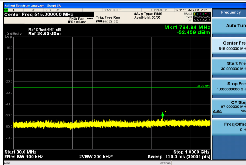
Band38-20MHz-16QAM-38150-1RB#0-30~1000MHz
