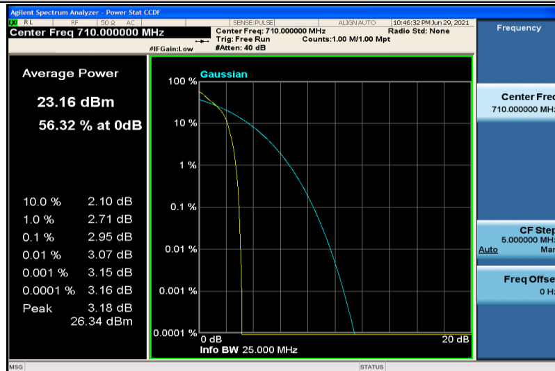
Band17-5MHz-QPSK-23790-1RB#0
