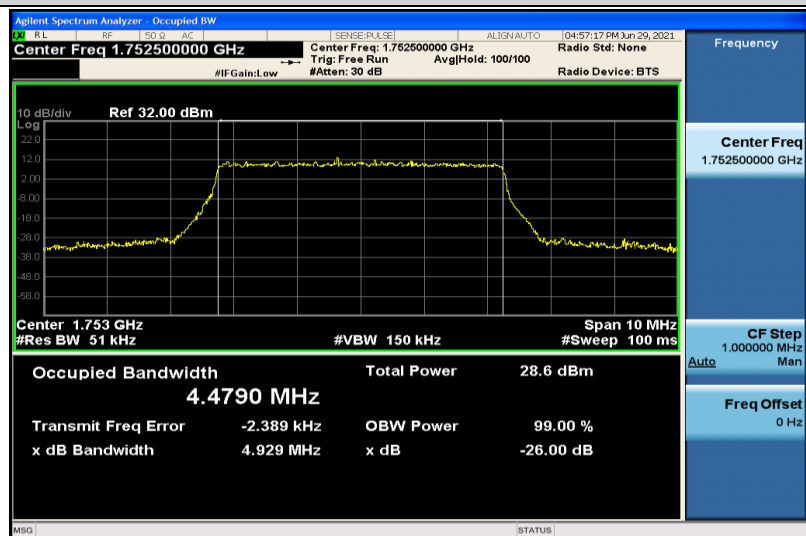
Band4-5MHz-16QAM-20375-25RB#0-4.4790
