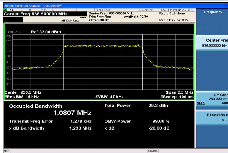
Band5-1.4MHz-QPSK-20525-6RB#0-1.0807
