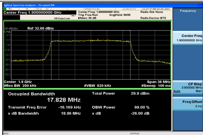
Band2-20MHz-QPSK-19100-100RB#0-17.828
