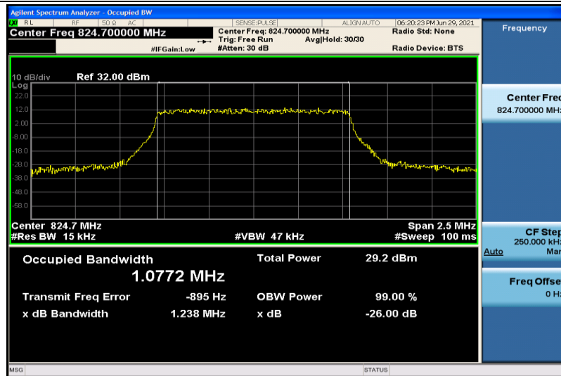
Band5-1.4MHz-QPSK-20407-6RB#0-1.0772
