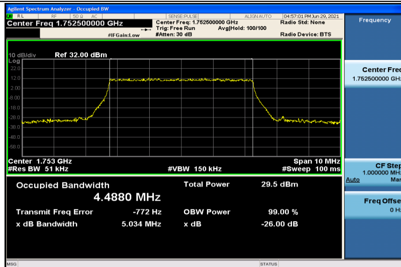
Band4-5MHz-QPSK-20375-25RB#0-4.4880
