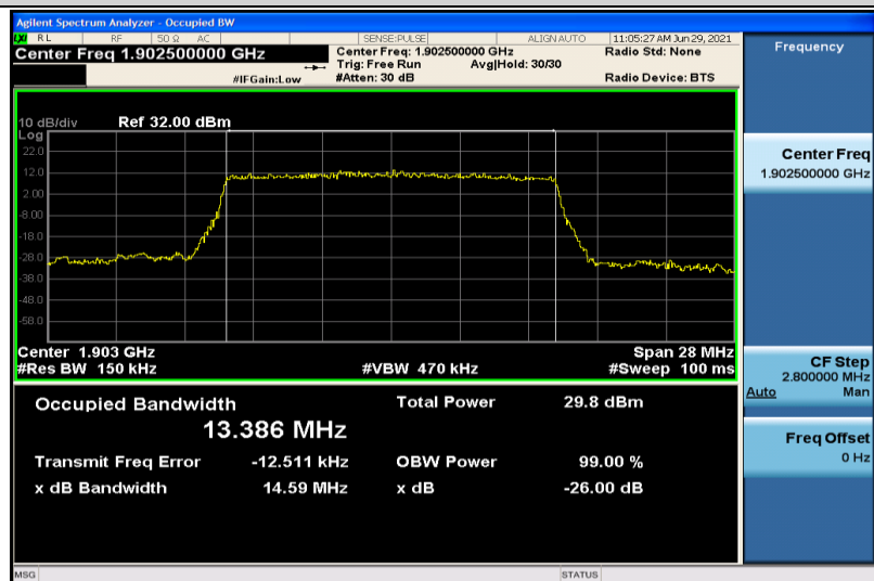
Band2-15MHz-QPSK-19125-75RB#0-13.386
