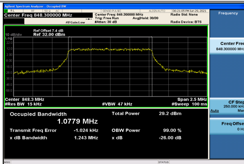
Band5-1.4MHz-QPSK-20643-6RB#0-1.0779
