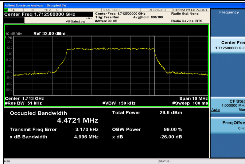
Band4-5MHz-QPSK-19975-25RB#0-4.4721
