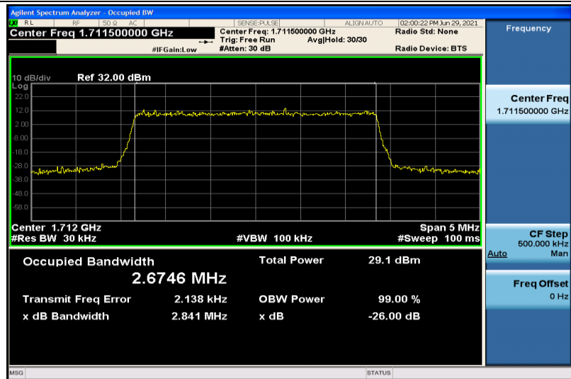
Band4-3MHz-QPSK-19965-15RB#0-2.6746
