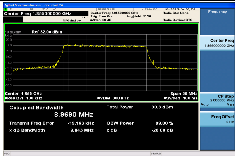
Band2-10MHz-QPSK-18650-50RB#0-8.9690
