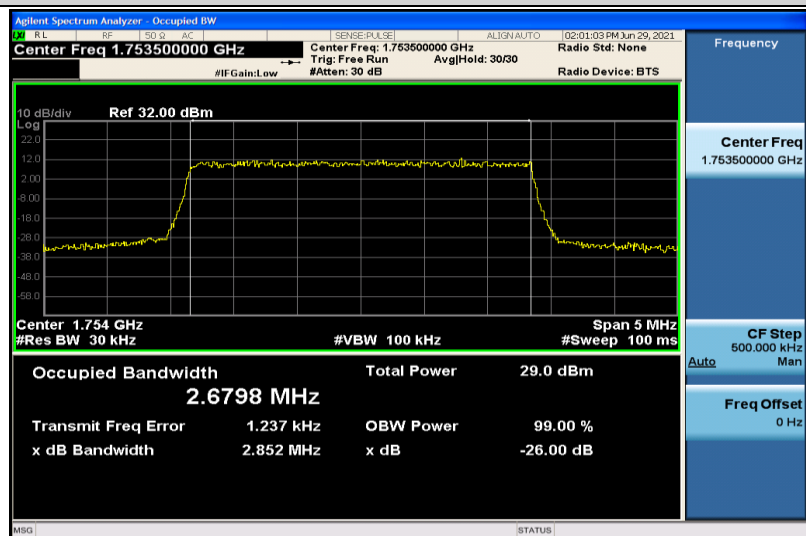
Band4-3MHz-QPSK-20385-15RB#0-2.6798
