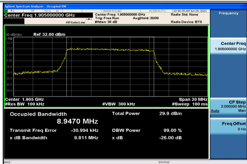
Band2-10MHz-QPSK-19150-50RB#0-8.9470
