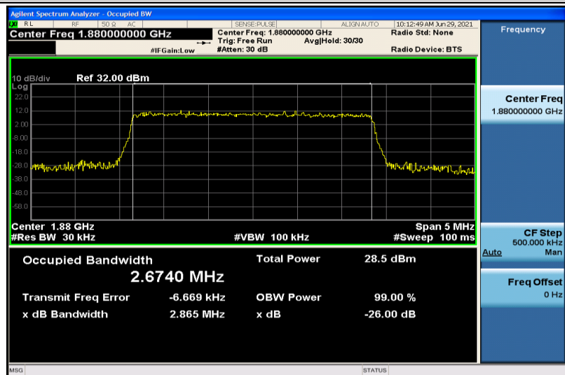
Band2-3MHz-16QAM-18900-15RB#0-2.6740
