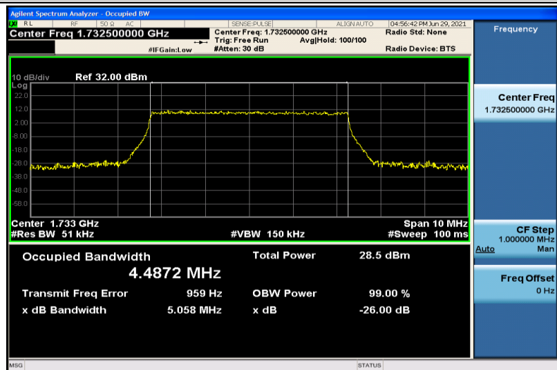
Band4-5MHz-16QAM-20175-25RB#0-4.4872
