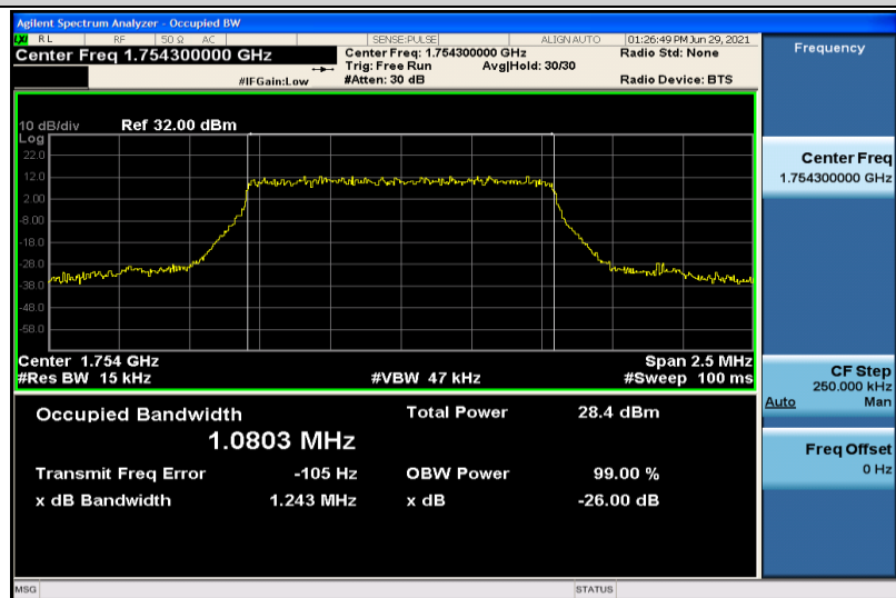
Band4-1.4MHz-QPSK-20393-6RB#0-1.0803
