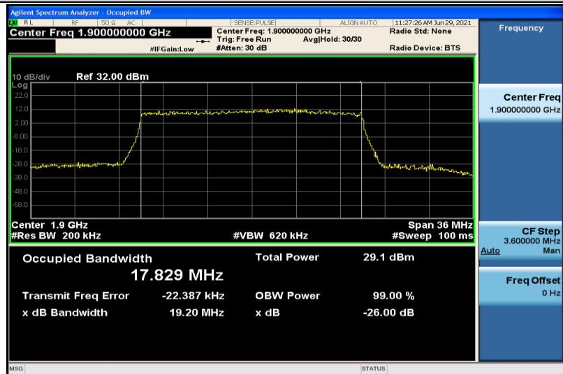
Band2-20MHz-16QAM-19100-100RB#0-17.829
