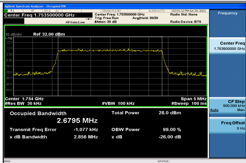
Band4-3MHz-16QAM-20385-15RB#0-2.6795
