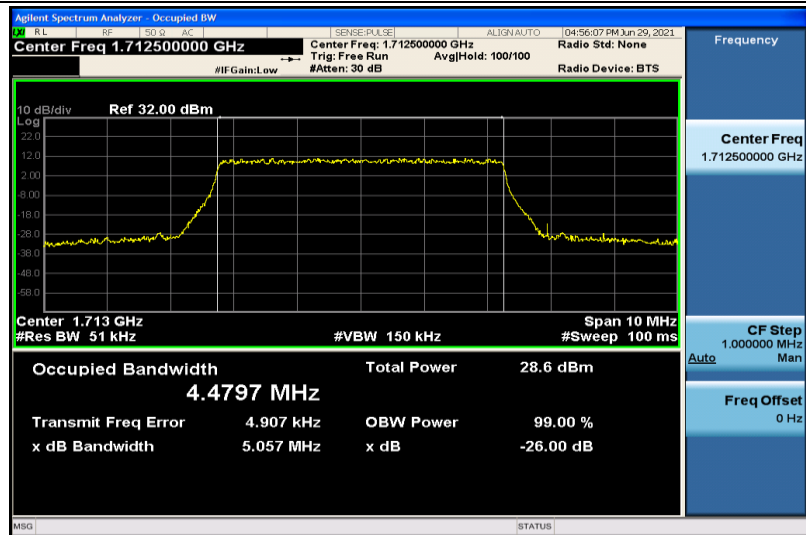
Band4-5MHz-16QAM-19975-25RB#0-4.4797
