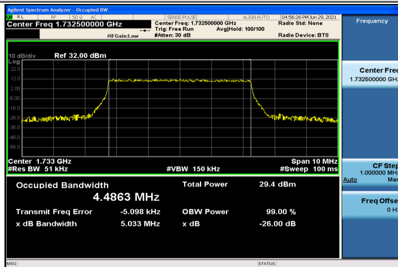
Band4-5MHz-QPSK-20175-25RB#0-4.4863
