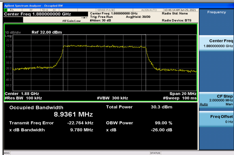
Band2-10MHz-QPSK-18900-50RB#0-8.9361
