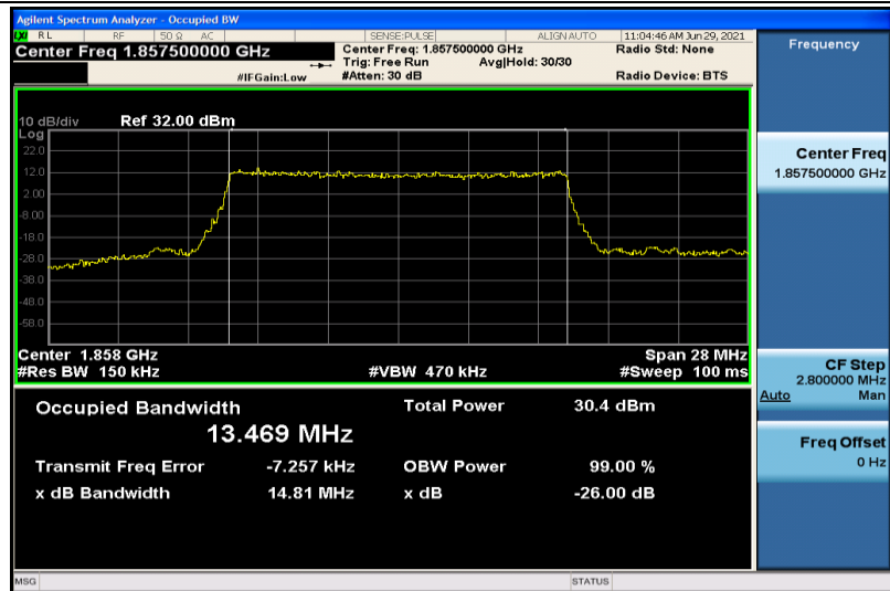
Band2-15MHz-QPSK-18675-75RB#0-13.469
