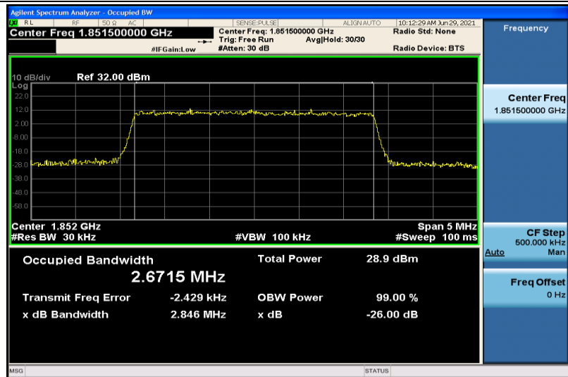
Band2-3MHz-16QAM-18615-15RB#0-2.6715
