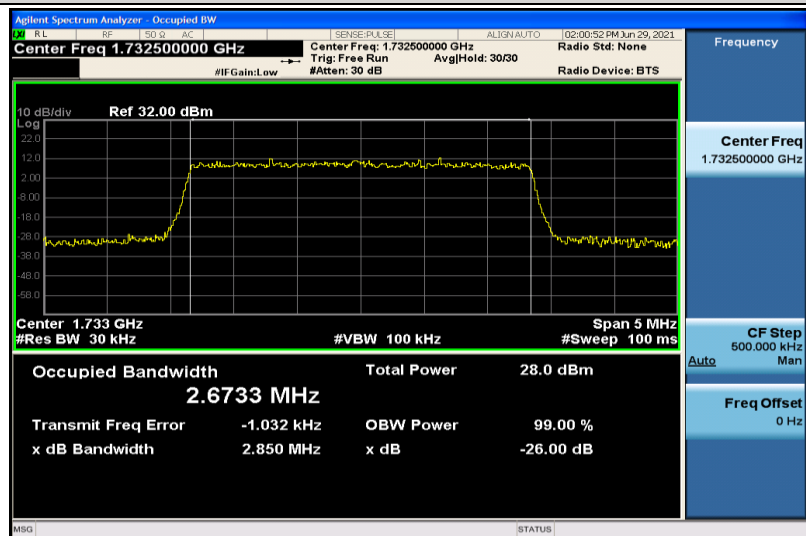
Band4-3MHz-16QAM-20175-15RB#0-2.6733
