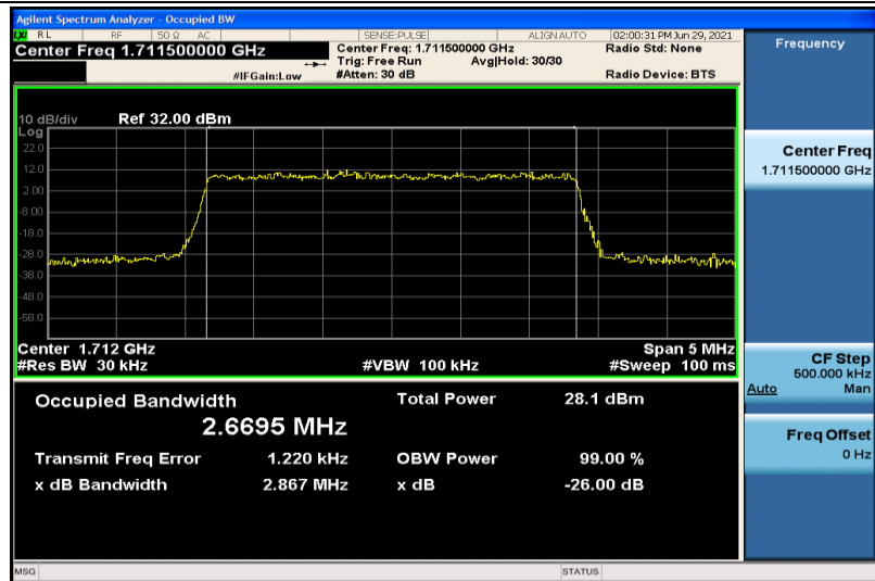
Band4-3MHz-16QAM-19965-15RB#0-2.6695
