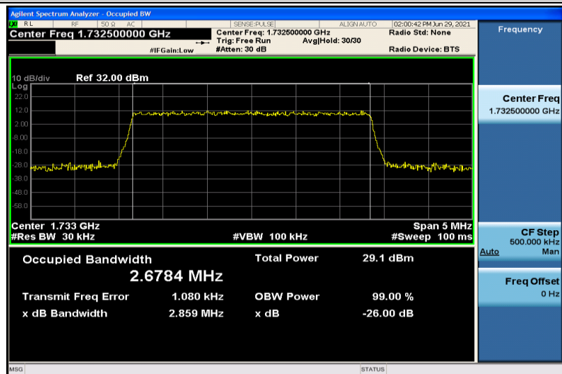
Band4-3MHz-QPSK-20175-15RB#0-2.6784
