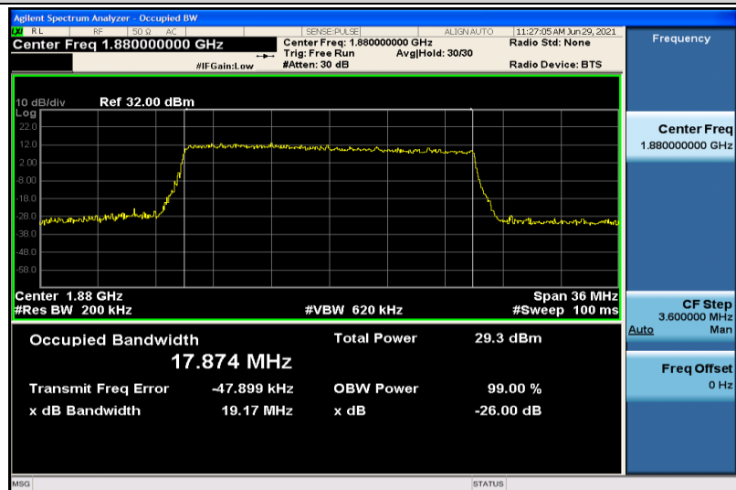
Band2-20MHz-16QAM-18900-100RB#0-17.874
