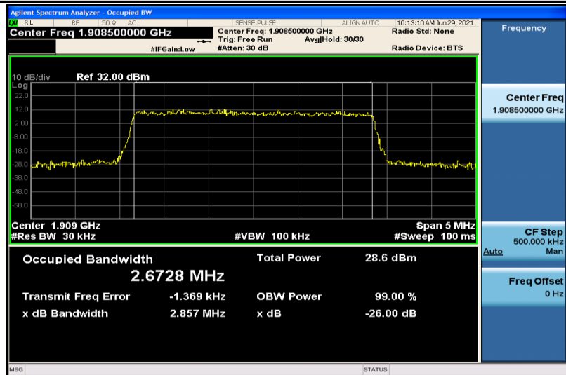
Band2-3MHz-16QAM-19185-15RB#0-2.6728
