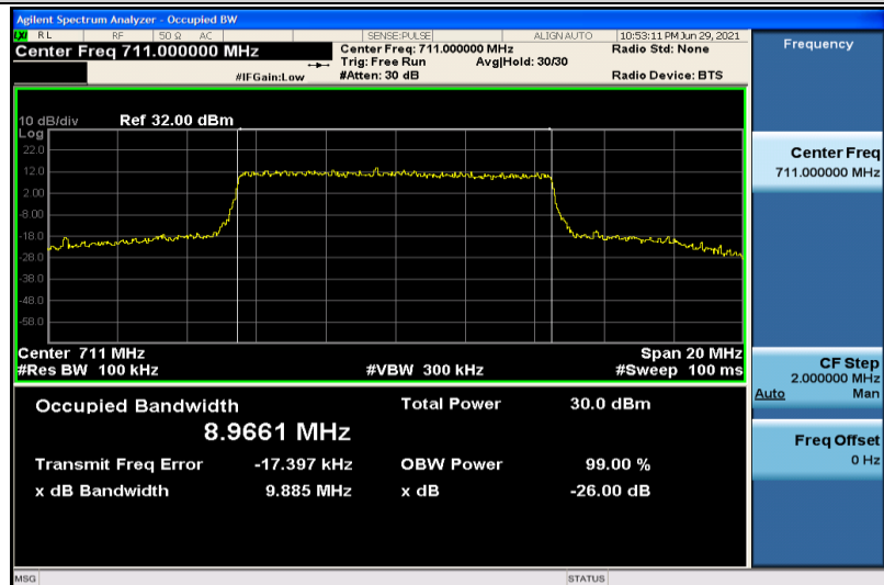
Band17-10MHz-16QAM-23800-50RB#0-8.9661
