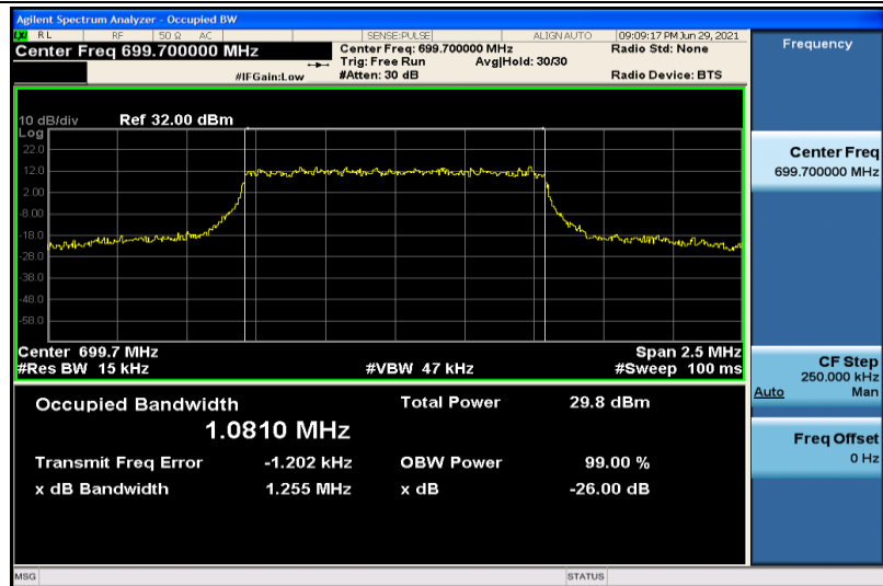
Band12-1.4MHz-QPSK-23017-6RB#0-1.0810
