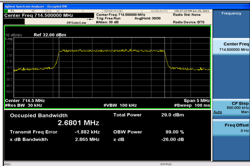
Band12-3MHz-16QAM-23165-15RB#0-2.6801
