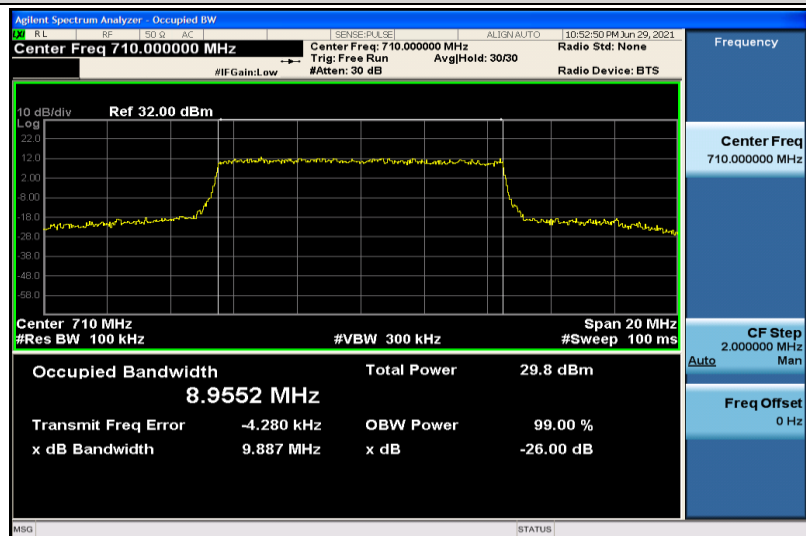
Band17-10MHz-16QAM-23790-50RB#0-8.9552
