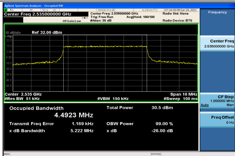
Band7-5MHz-QPSK-21100-25RB#0-4.4923
