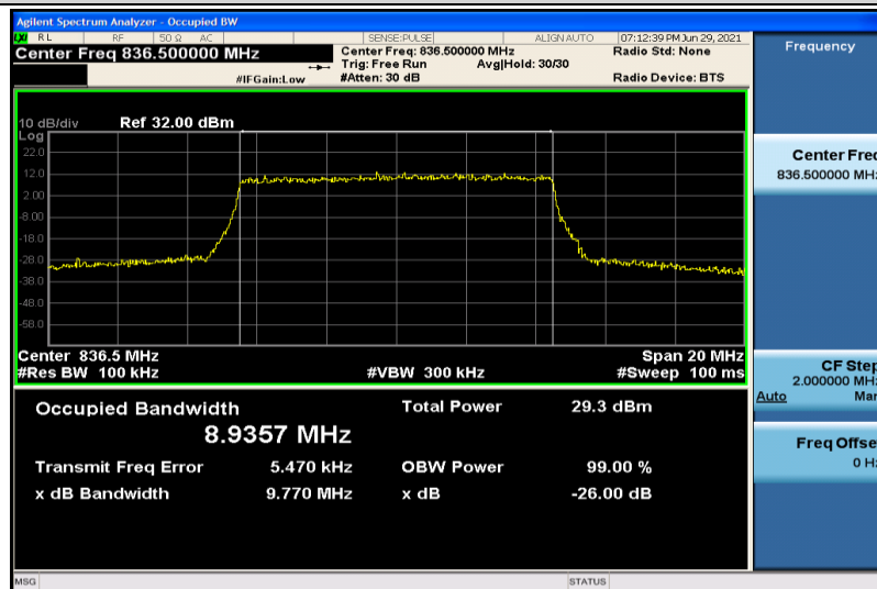
Band5-10MHz-16QAM-20525-50RB#0-8.9357
