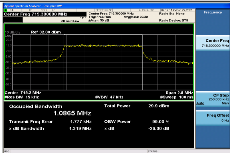
Band12-1.4MHz-QPSK-23173-6RB#0-1.0865
