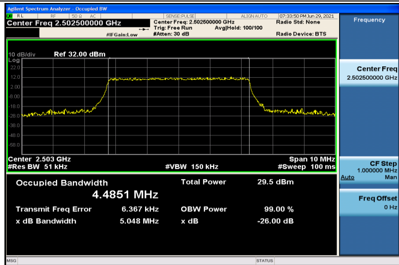
Band7-5MHz-16QAM-20775-25RB#0-4.4851
