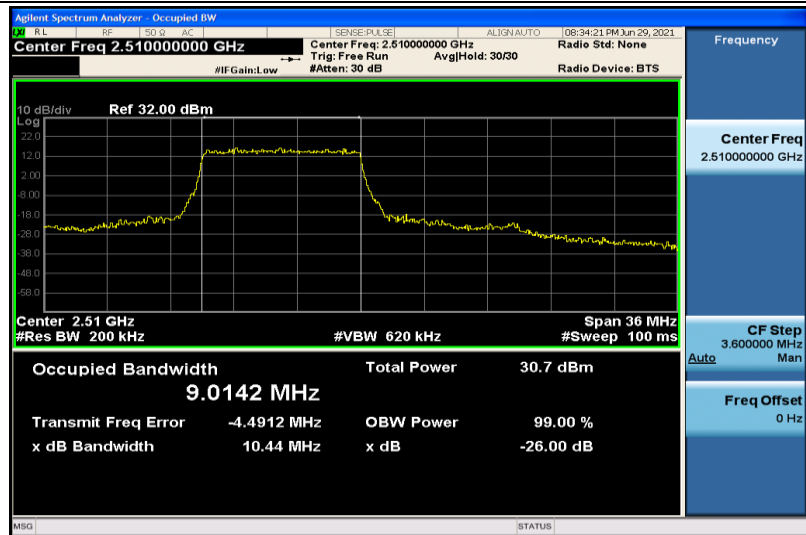
Band7-20MHz-QPSK-20850-100RB#0-9.0142
