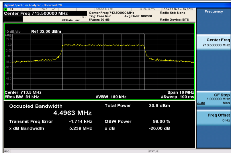
Band17-5MHz-QPSK-23825-25RB#0-4.4963
