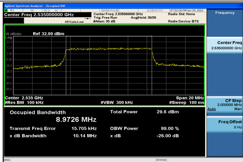
Band7-10MHz-16QAM-21100-50RB#0-8.9726
