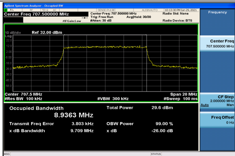
Band12-10MHz-16QAM-23095-50RB#0-8.9363
