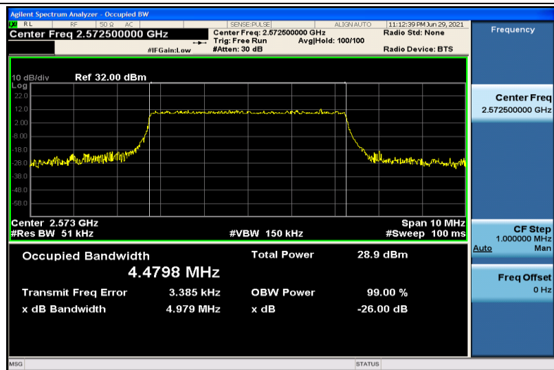
Band38-5MHz-16QAM-37775-25RB#0-4.4798
