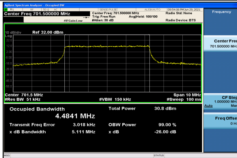
Band12-5MHz-QPSK-23035-25RB#0-4.4841
