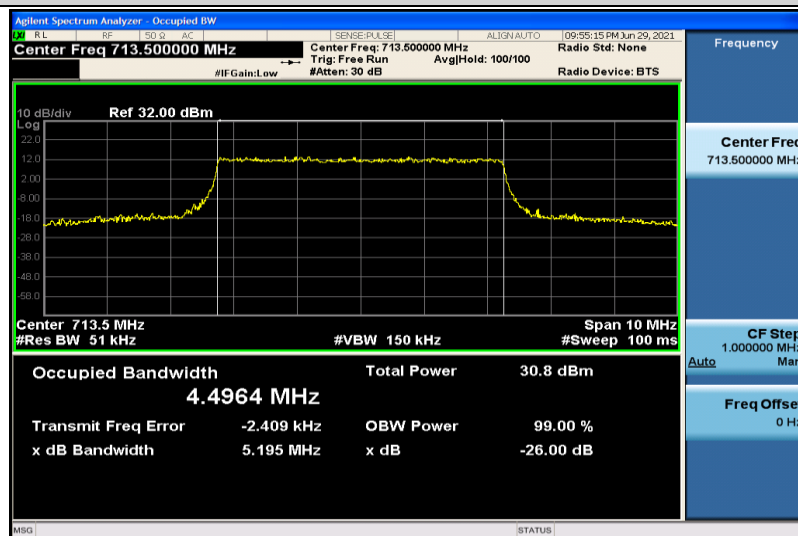
Band12-5MHz-QPSK-23155-25RB#0-4.4964
