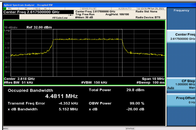
Band38-5MHz-QPSK-38225-25RB#0-4.4811
