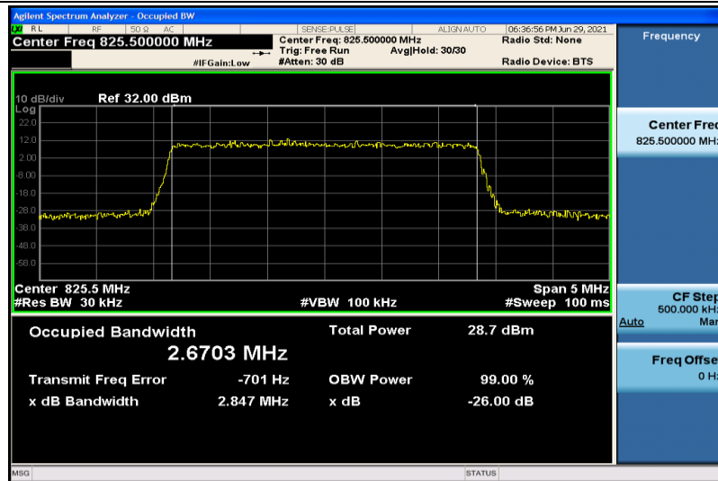
Band5-3MHz-16QAM-20415-15RB#0-2.6703
