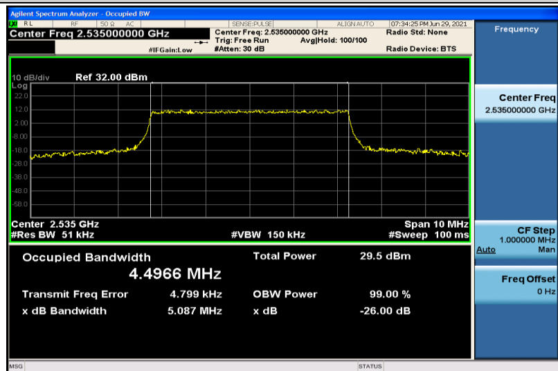
Band7-5MHz-16QAM-21100-25RB#0-4.4966
