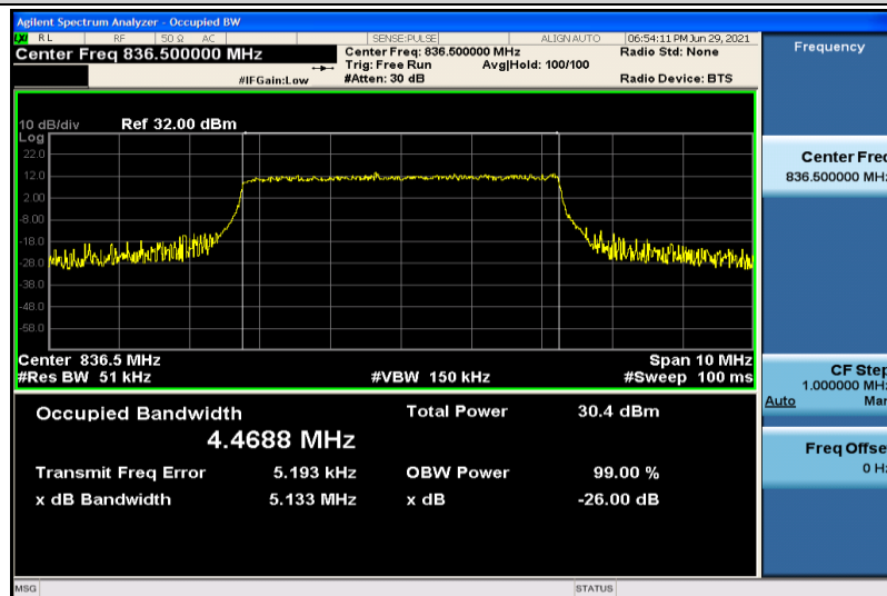
Band5-5MHz-QPSK-20525-25RB#0-4.4688
