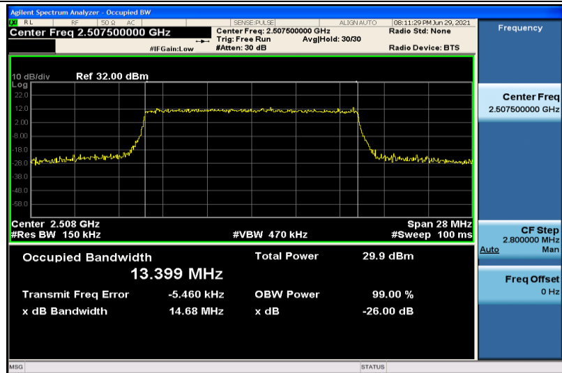
Band7-15MHz-16QAM-20825-75RB#0-13.399
