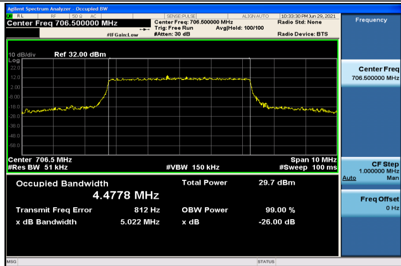
Band17-5MHz-16QAM-23755-25RB#0-4.4778
