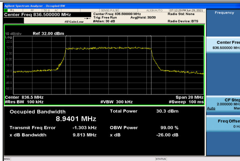
Band5-10MHz-QPSK-20525-50RB#0-8.9401
