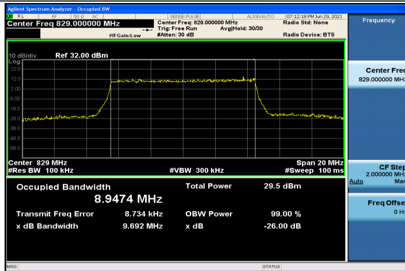
Band5-10MHz-16QAM-20450-50RB#0-8.9474
