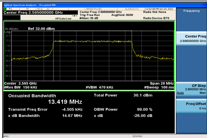
Band38-15MHz-QPSK-38000-75RB#0-13.419
