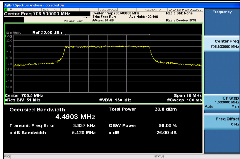
Band17-5MHz-QPSK-23755-25RB#0-4.4903
