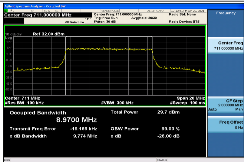
Band12-10MHz-16QAM-23130-50RB#0-8.9700
