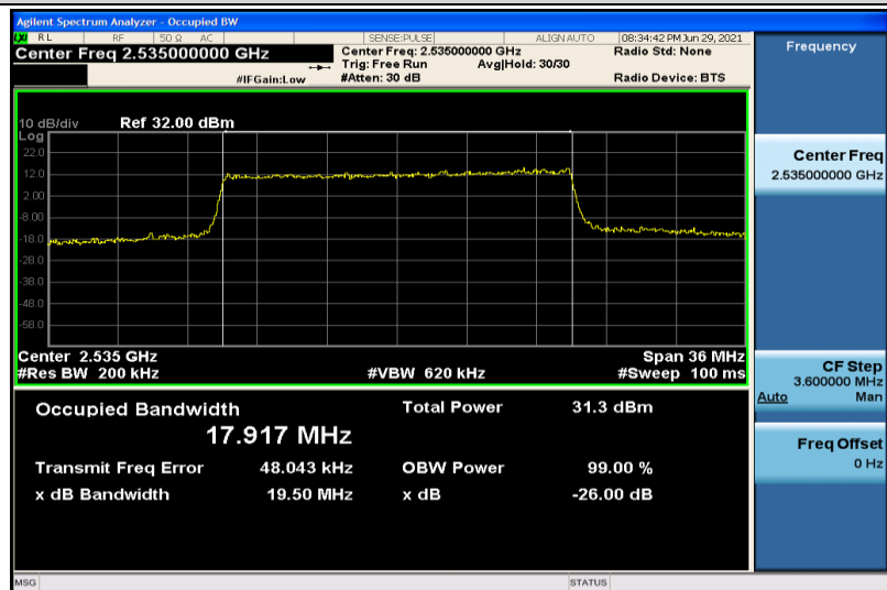
Band7-20MHz-QPSK-21100-100RB#0-17.917
