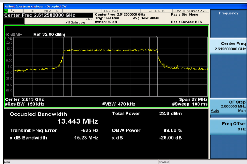
Band38-15MHz-16QAM-38175-75RB#0-13.443
