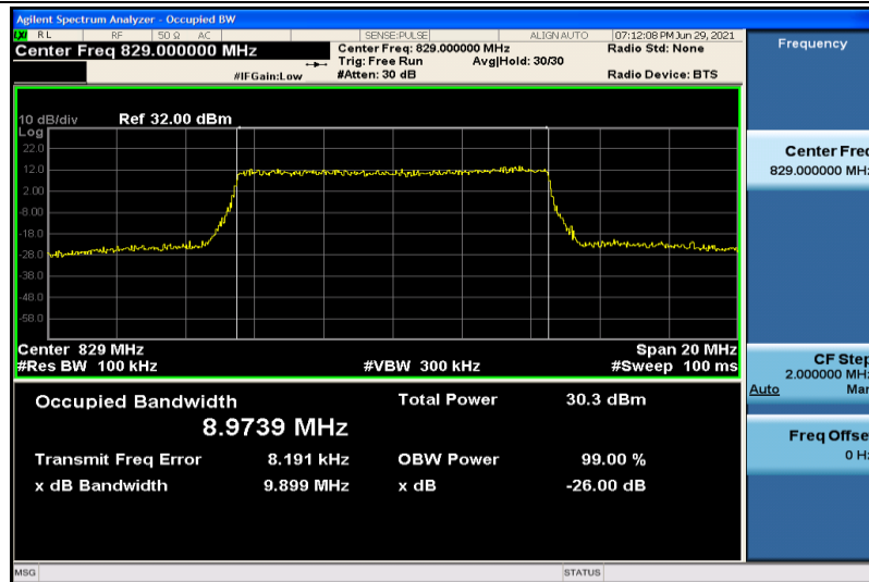
Band5-10MHz-QPSK-20450-50RB#0-8.9739
