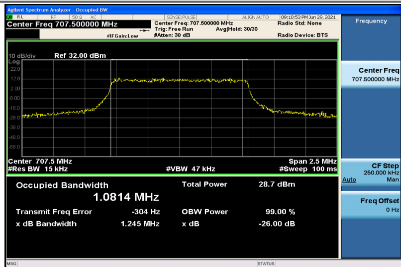
Band12-1.4MHz-16QAM-23095-6RB#0-1.0814
