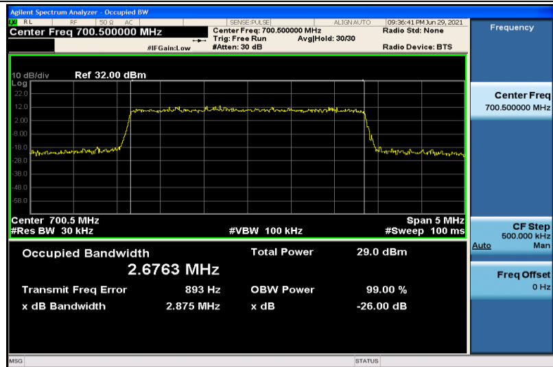
Band12-3MHz-16QAM-23025-15RB#0-2.6763
