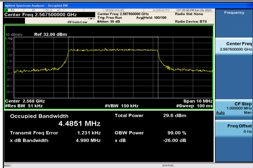
Band7-5MHz-16QAM-21425-25RB#0-4.4851
