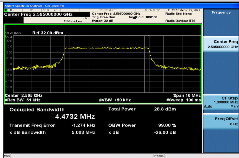
Band38-5MHz-16QAM-38000-25RB#0-4.4732
