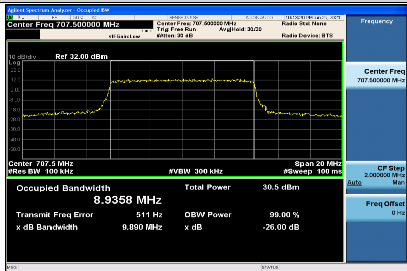
Band12-10MHz-QPSK-23095-50RB#0-8.9358
