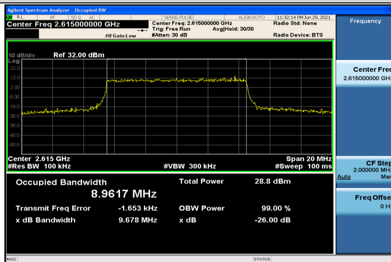
Band38-10MHz-16QAM-38200-50RB#0-8.9617
