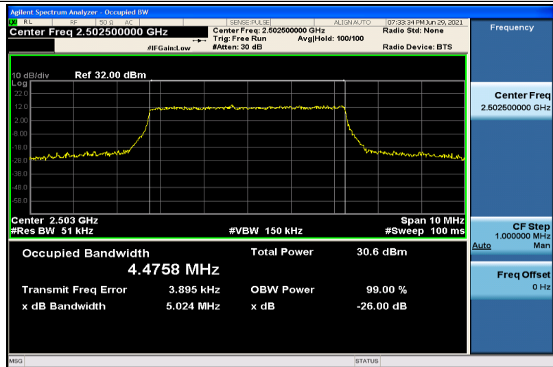
Band7-5MHz-QPSK-20775-25RB#0-4.4758
