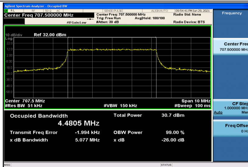
Band12-5MHz-QPSK-23095-25RB#0-4.4805
