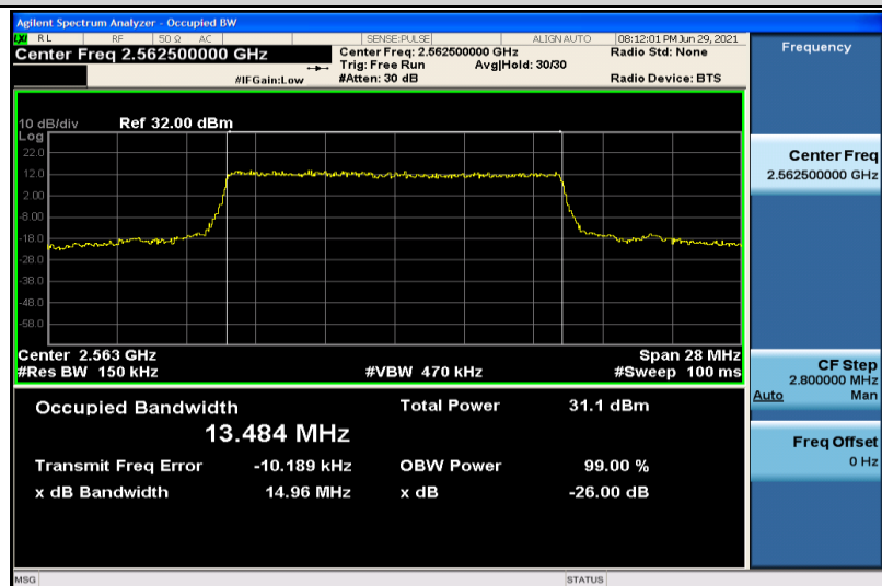
Band7-15MHz-QPSK-21375-75RB#0-13.484
