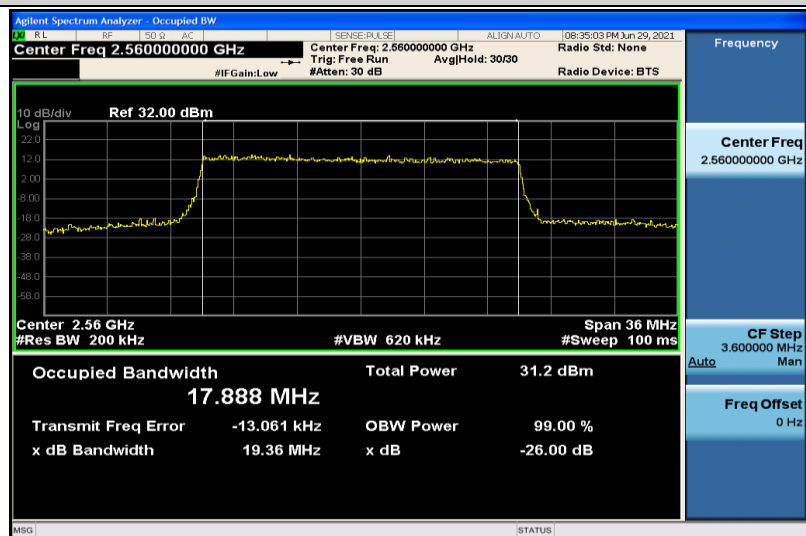
Band7-20MHz-QPSK-21350-100RB#0-17.888
