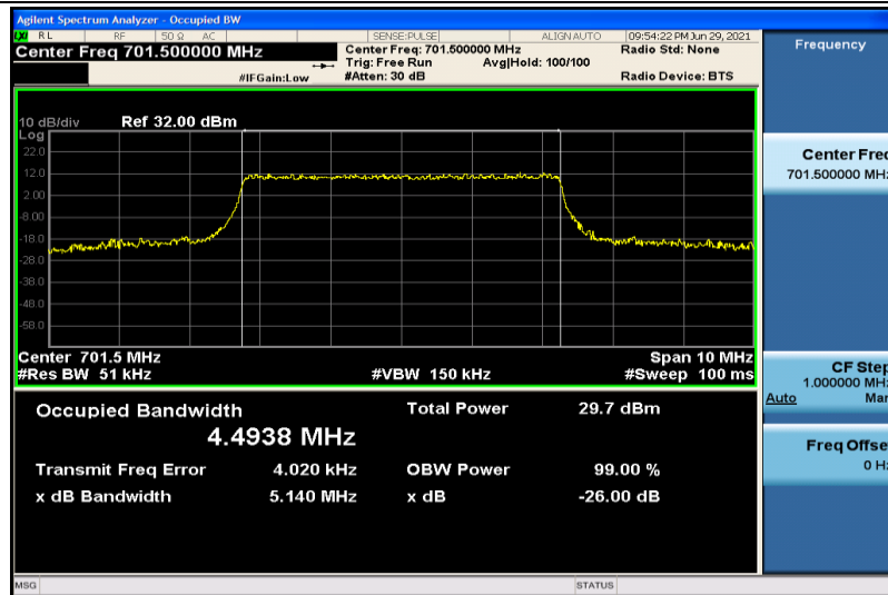
Band12-5MHz-16QAM-23035-25RB#0-4.4938
