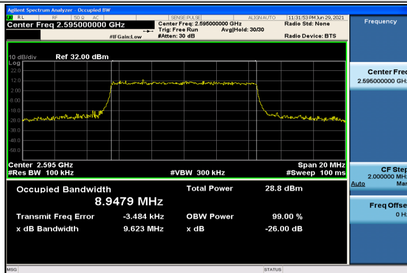
Band38-10MHz-16QAM-38000-50RB#0-8.9479
