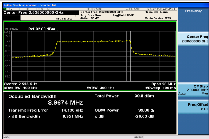
Band7-10MHz-QPSK-21100-50RB#0-8.9674
