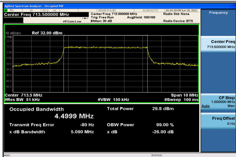
Band17-5MHz-16QAM-23825-25RB#0-4.4999
