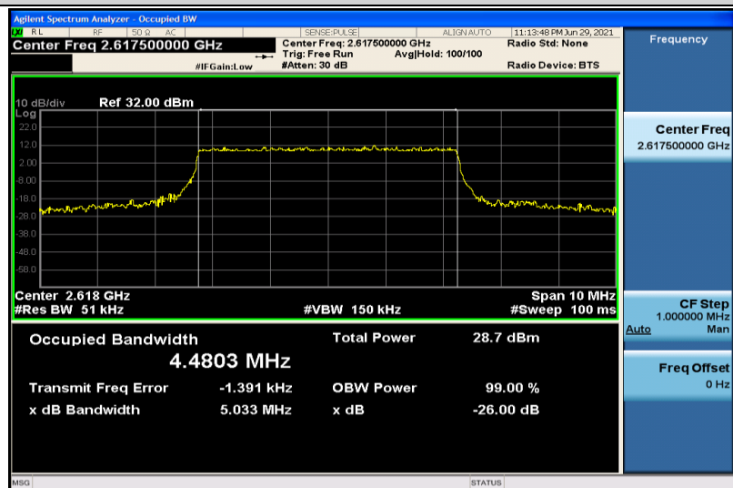
Band38-5MHz-16QAM-38225-25RB#0-4.4803
