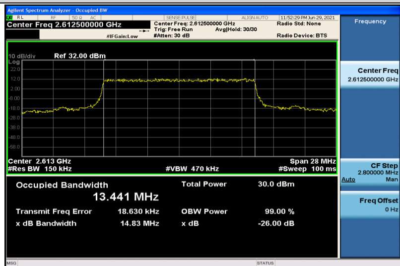
Band38-15MHz-QPSK-38175-75RB#0-13.441
