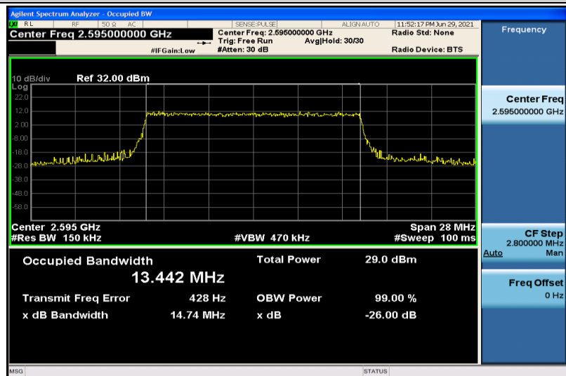
Band38-15MHz-16QAM-38000-75RB#0-13.442
