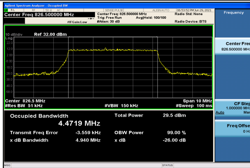
Band5-5MHz-16QAM-20425-25RB#0-4.4719
