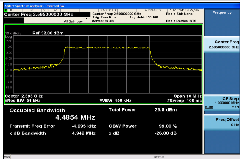
Band38-5MHz-QPSK-38000-25RB#0-4.4854
