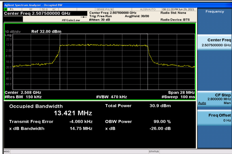
Band7-15MHz-QPSK-20825-75RB#0-13.421
