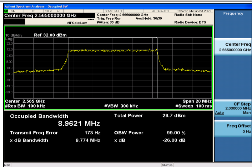
Band7-10MHz-16QAM-21400-50RB#0-8.9621
