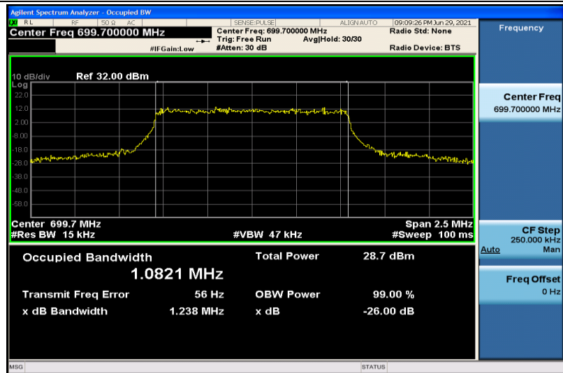
Band12-1.4MHz-16QAM-23017-6RB#0-1.0821
