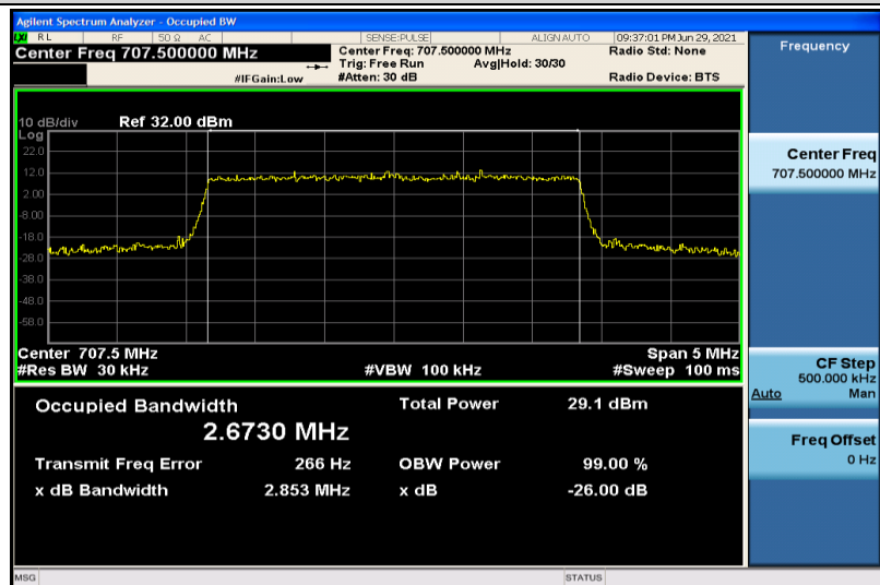
Band12-3MHz-16QAM-23095-15RB#0-2.6730
