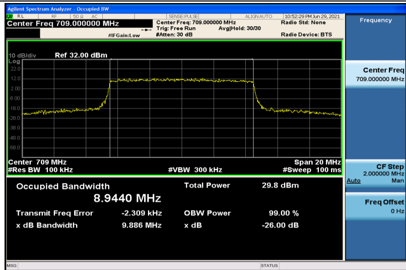
Band17-10MHz-16QAM-23780-50RB#0-8.9440
