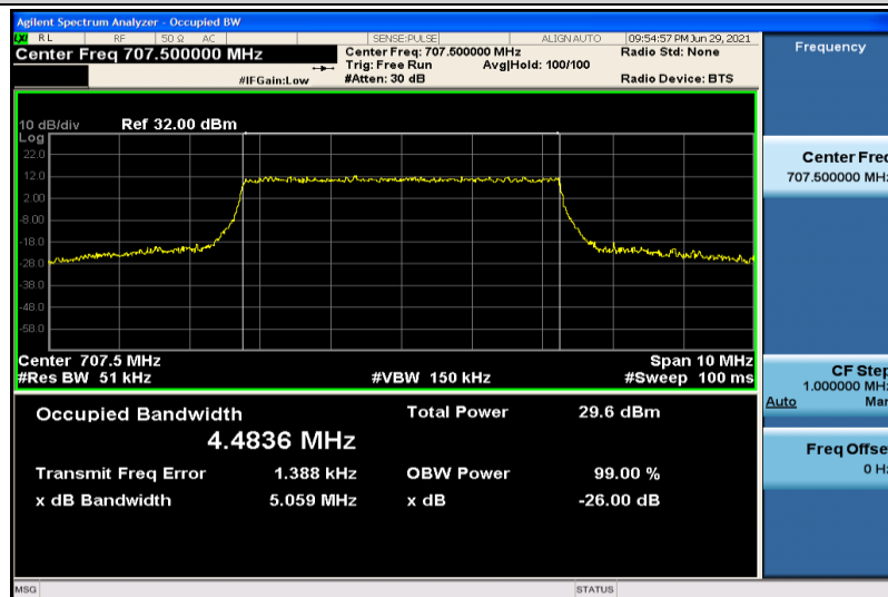
Band12-5MHz-16QAM-23095-25RB#0-4.4836
