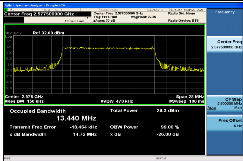
Band38-15MHz-16QAM-37825-75RB#0-13.440
