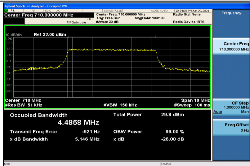
Band17-5MHz-16QAM-23790-25RB#0-4.4858
