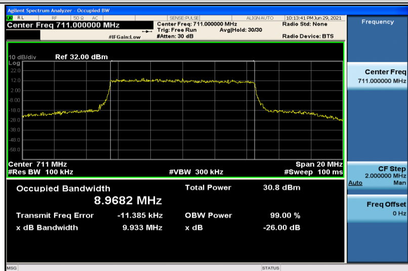
Band12-10MHz-QPSK-23130-50RB#0-8.9682
