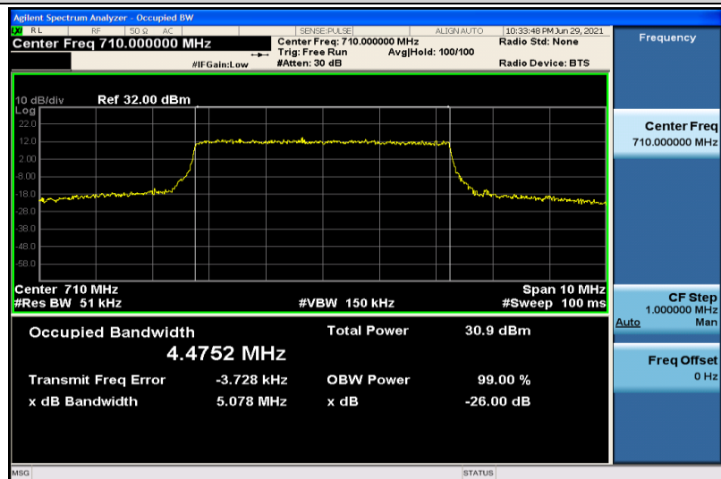
Band17-5MHz-QPSK-23790-25RB#0-4.4752
