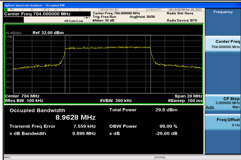
Band12-10MHz-16QAM-23060-50RB#0-8.9628
