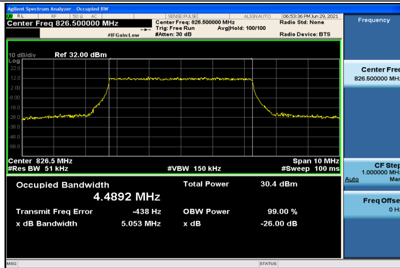
Band5-5MHz-QPSK-20425-25RB#0-4.4892
