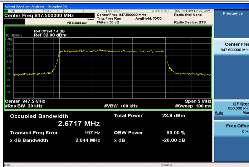
Band5-3MHz-16QAM-20635-15RB#0-2.6717
