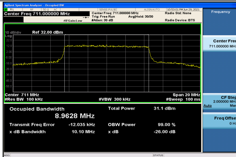
Band17-10MHz-QPSK-23800-50RB#0-8.9628
