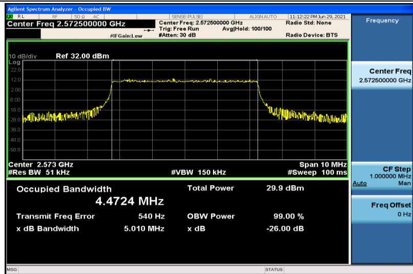
Band38-5MHz-QPSK-37775-25RB#0-4.4724
