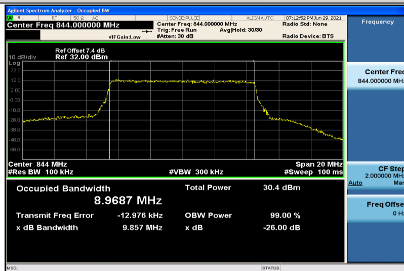
Band5-10MHz-QPSK-20600-50RB#0-8.9687
