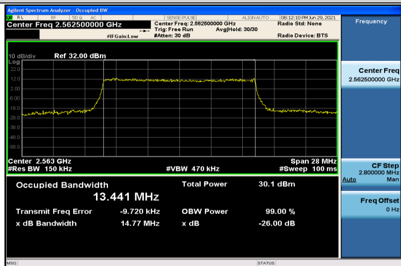
Band7-15MHz-16QAM-21375-75RB#0-13.441
