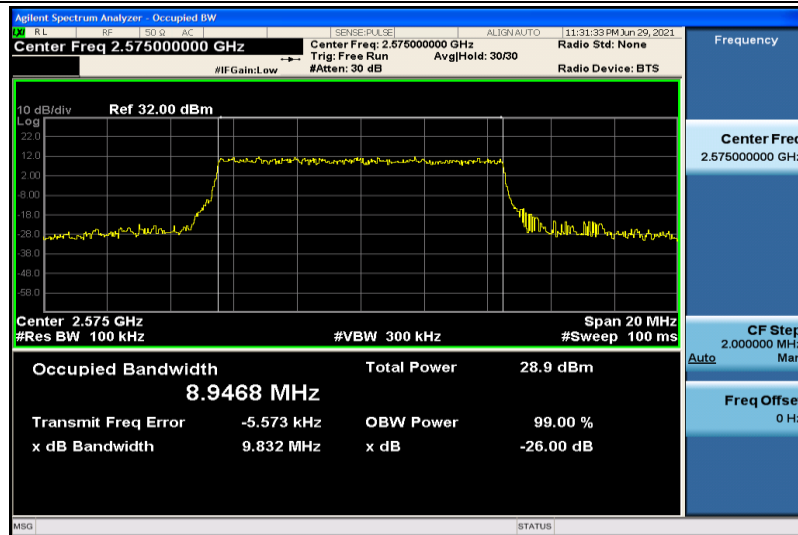
Band38-10MHz-16QAM-37800-50RB#0-8.9468
