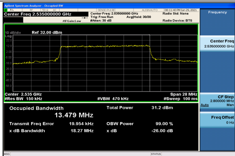
Band7-15MHz-QPSK-21100-75RB#0-13.479
