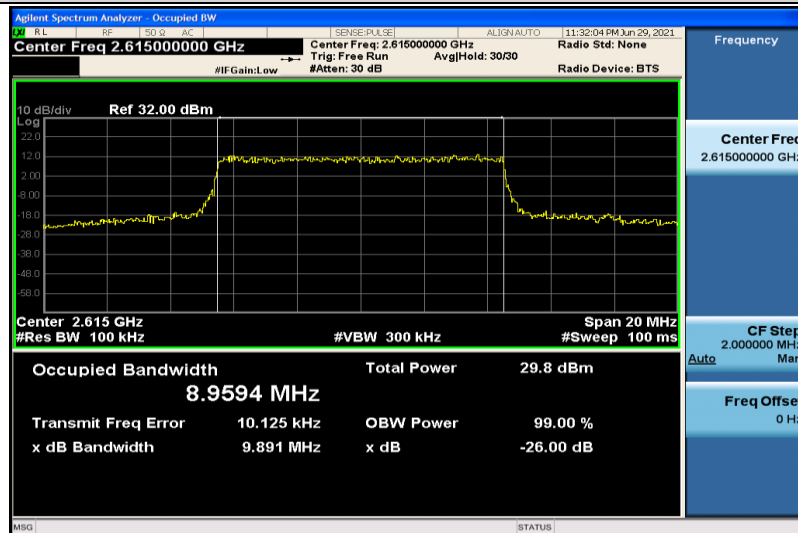
Band38-10MHz-QPSK-38200-50RB#0-8.9594
