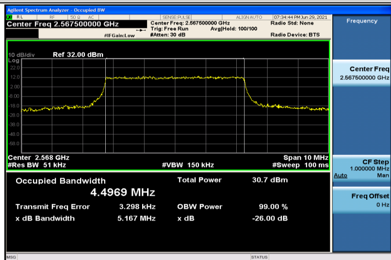
Band7-5MHz-QPSK-21425-25RB#0-4.4969
