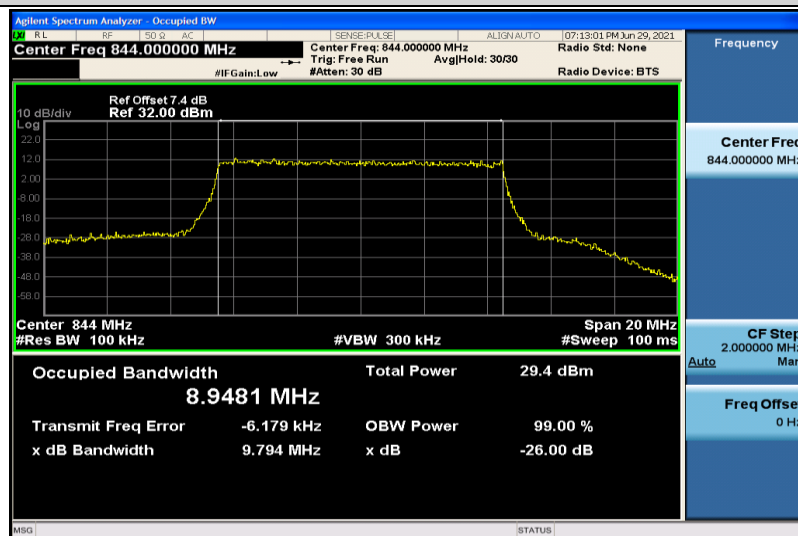
Band5-10MHz-16QAM-20600-50RB#0-8.9481
