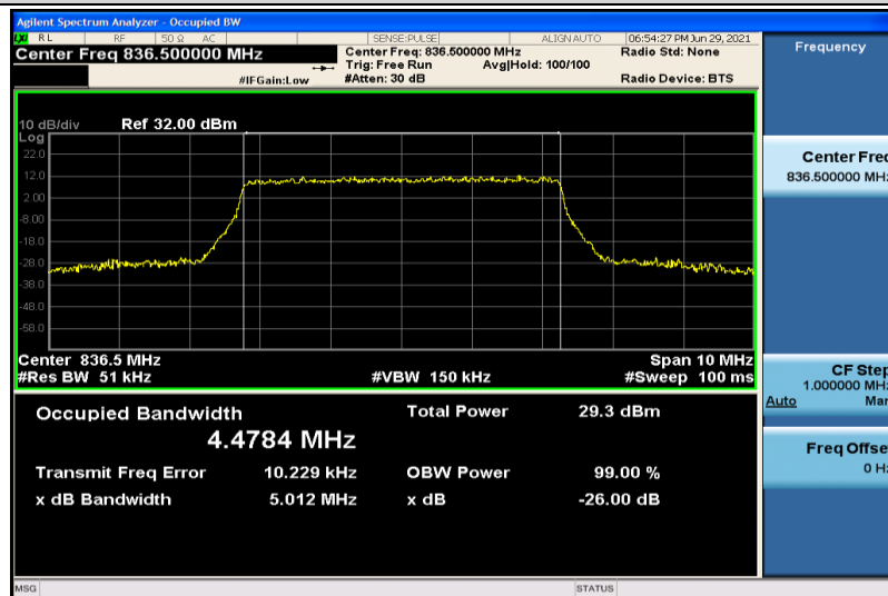
Band5-5MHz-16QAM-20525-25RB#0-4.4784
