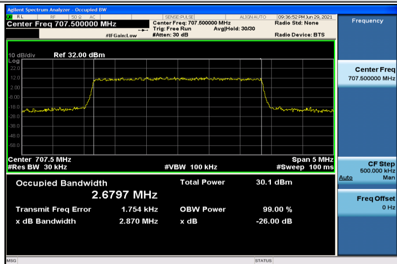
Band12-3MHz-QPSK-23095-15RB#0-2.6797
