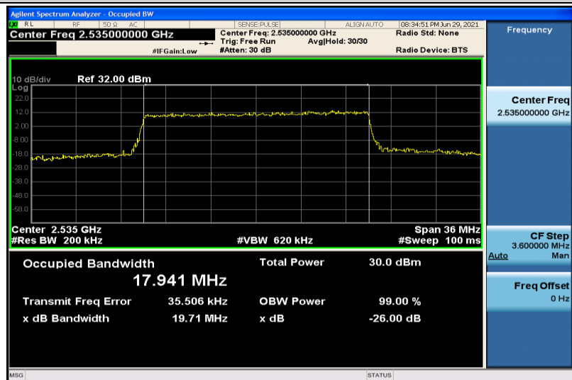
Band7-20MHz-16QAM-21100-100RB#0-17.941
