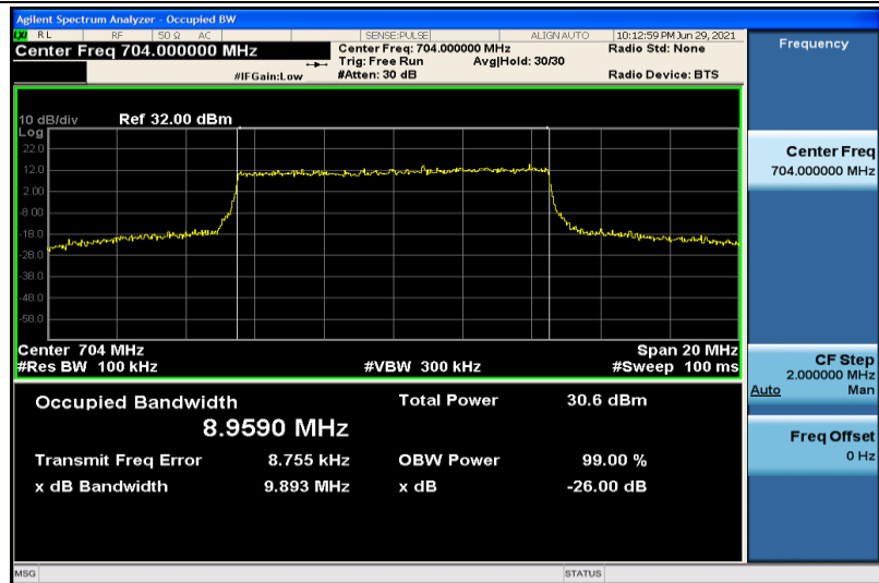
Band12-10MHz-QPSK-23060-50RB#0-8.9590
