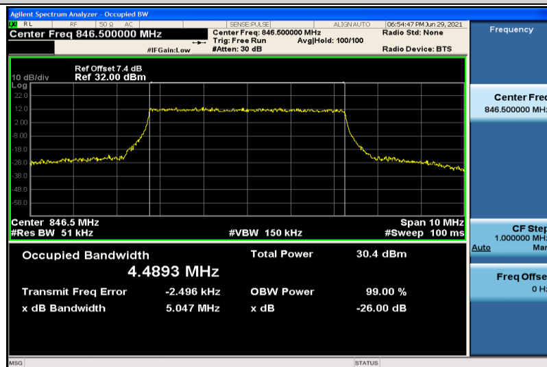
Band5-5MHz-QPSK-20625-25RB#0-4.4893
