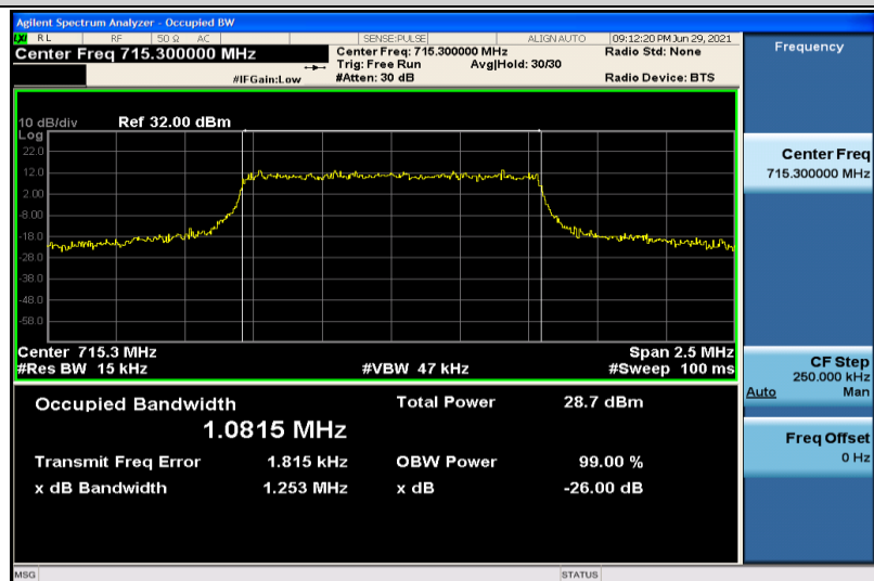
Band12-1.4MHz-16QAM-23173-6RB#0-1.0815
