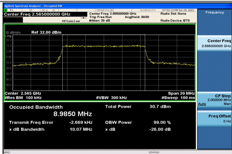
Band7-10MHz-QPSK-21400-50RB#0-8.9850
