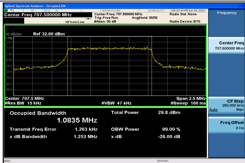
Band12-1.4MHz-QPSK-23095-6RB#0-1.0835
