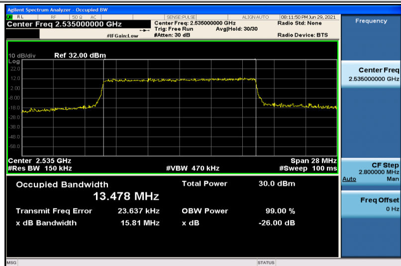
Band7-15MHz-16QAM-21100-75RB#0-13.478
