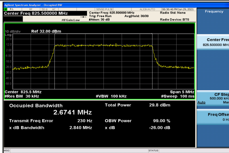
Band5-3MHz-QPSK-20415-15RB#0-2.6741
