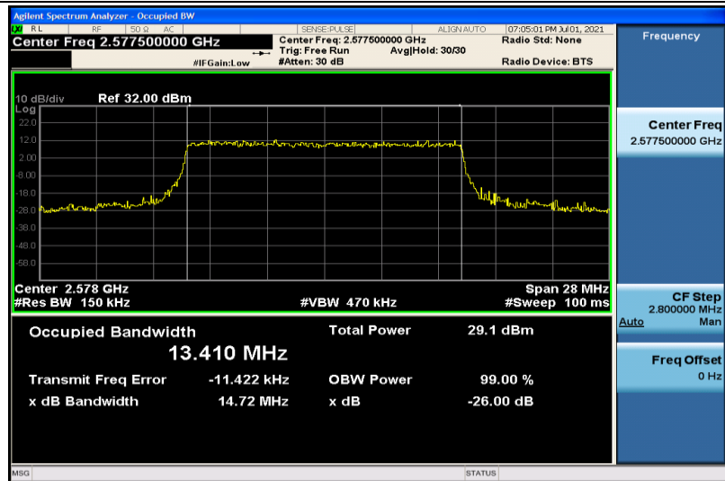
Band38-15MHz-QPSK-37825-75RB#0-13.410
