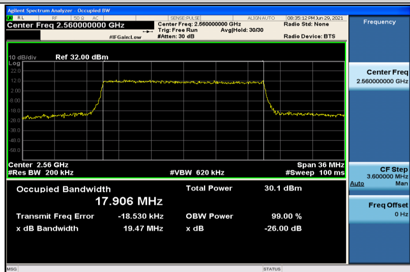
Band7-20MHz-16QAM-21350-100RB#0-17.906
