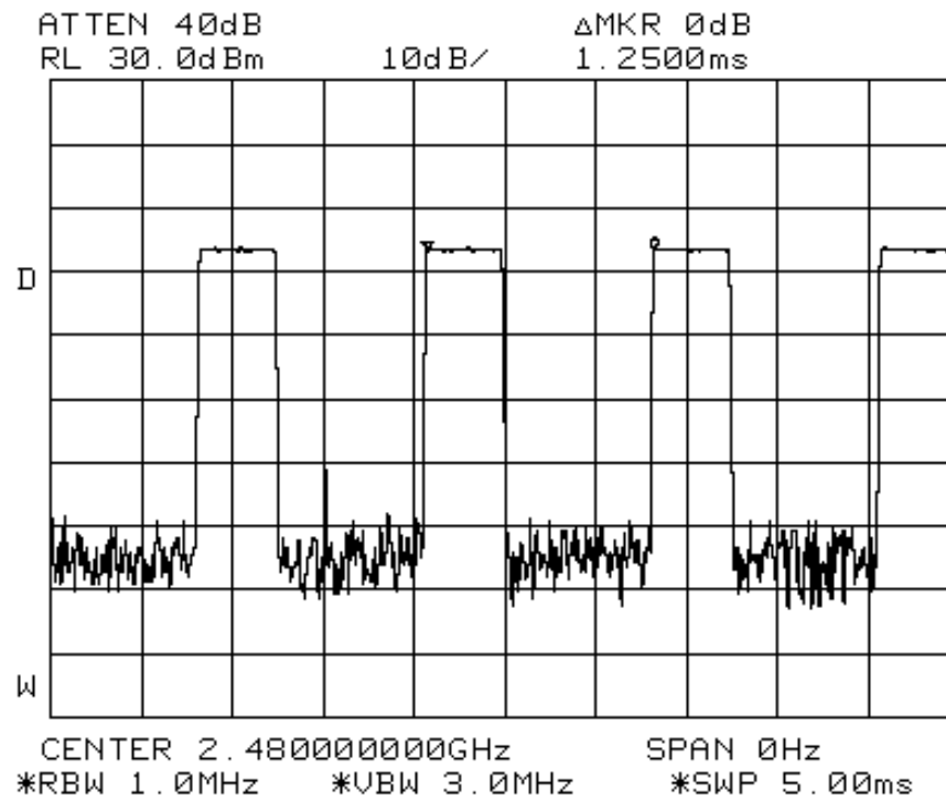
Plot 14 – Channel 78
