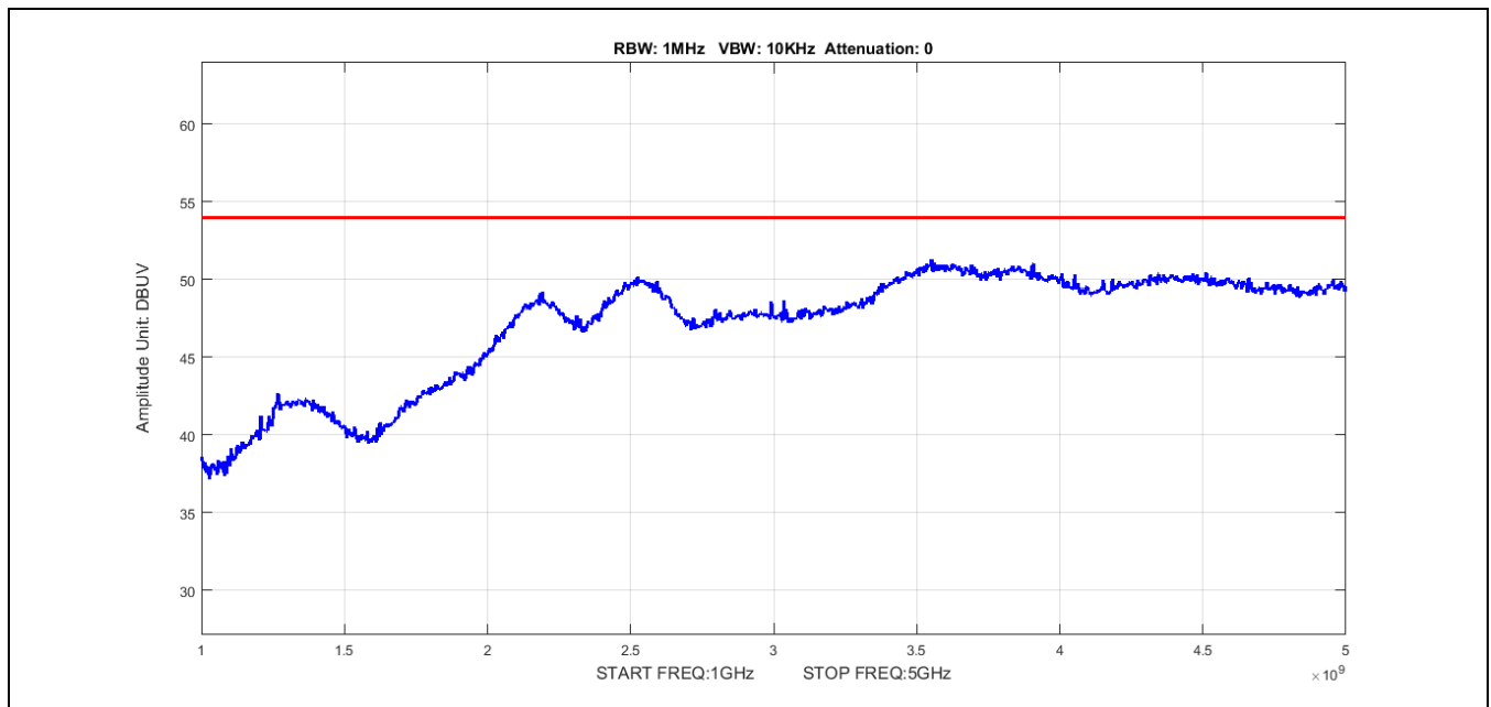
Plot 13. Radiated Spurious Emissions, 1 - 5 GHz Mid Channel Average
