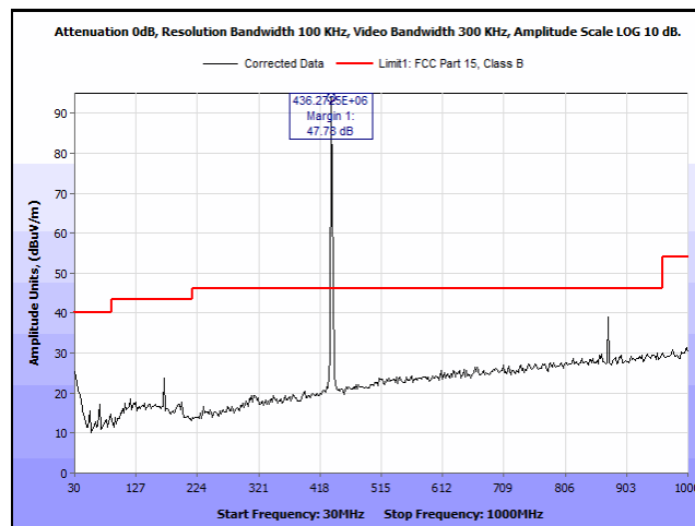
Plot 9. Radiated Spurious Emissions, 436.6 MHz High Channel Below 1 GHz
