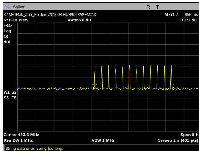
Plot 6. Duty Cycle, Period
