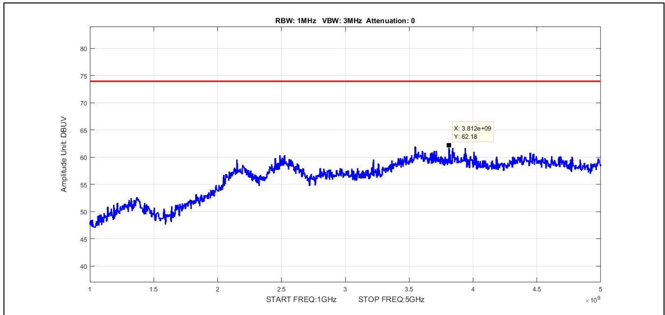
Plot 10. Radiated Spurious Emissions, 1 - 5 GHz Low Channel Peak
