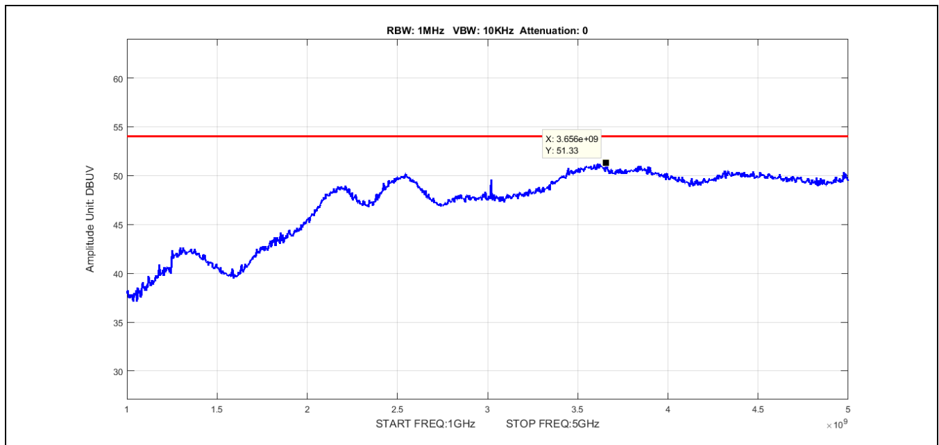
Plot 11. Radiated Spurious Emissions, 1 - 5 GHz Low Channel Average
