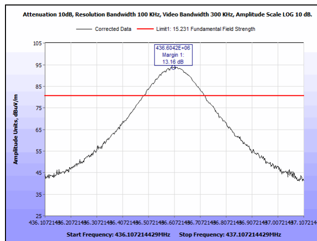
Plot 6. 436.6 MHz High Channel
