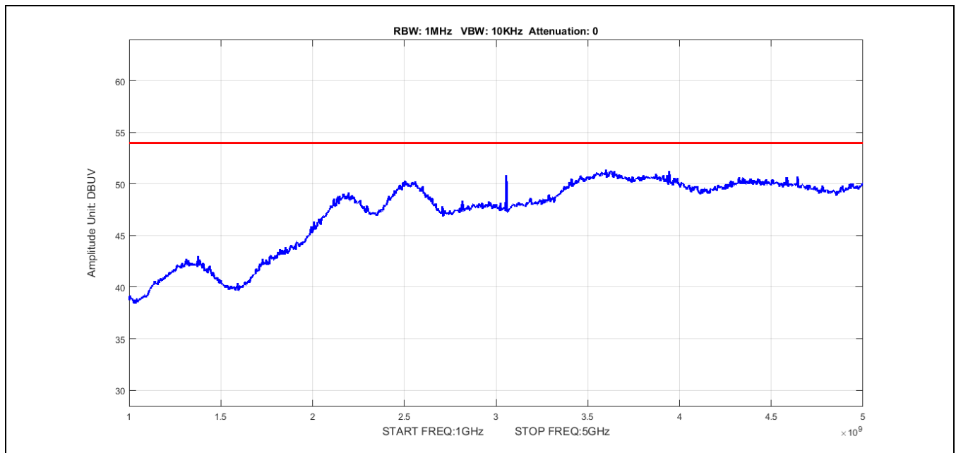
Plot 7. Radiated Spurious Emissions, 1 – 5 GHz High Channel Average
