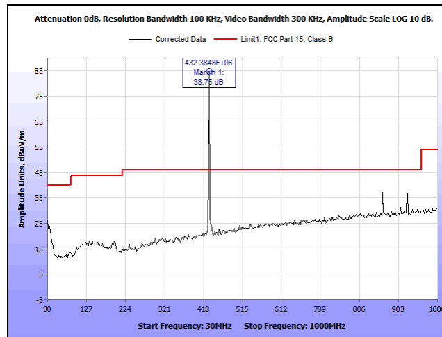
Plot 7. Radiated Spurious Emissions, 431.6 MHz Low Channel Below 1 GHz
