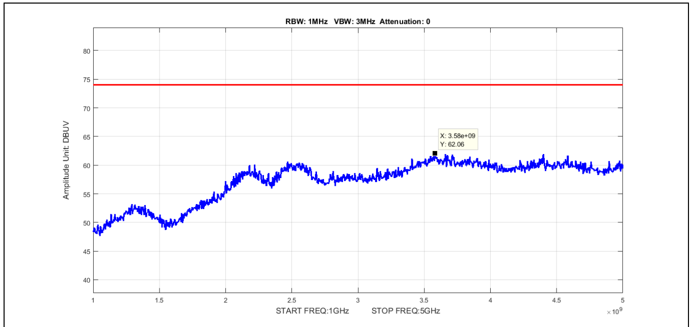
Plot 12. Radiated Spurious Emissions, 1 - 5 GHz Mid Channel Peak
