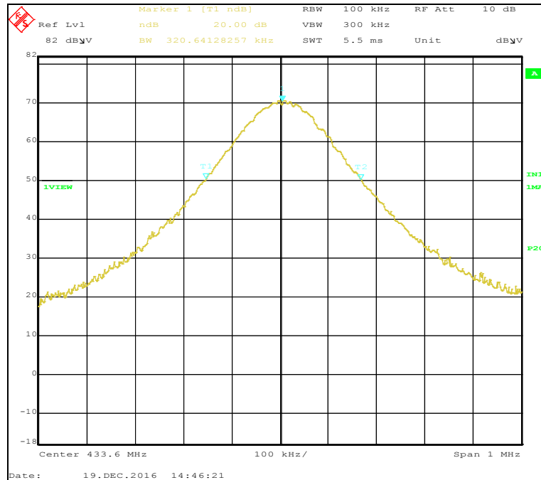
Plot 8. 20 dB Bandwidth Plot, 433.6 MHz Mid Channel
