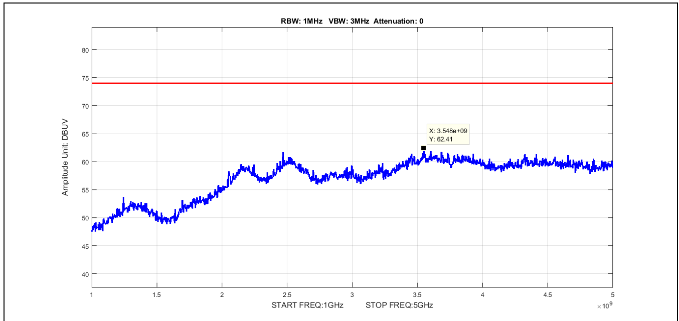
Plot 14. Radiated Spurious Emissions, 1 - 5 GHz High Channel Peak
