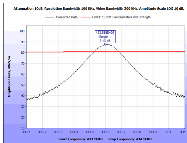
Plot 5. 433.6 MHz Channel, Mid Channel
