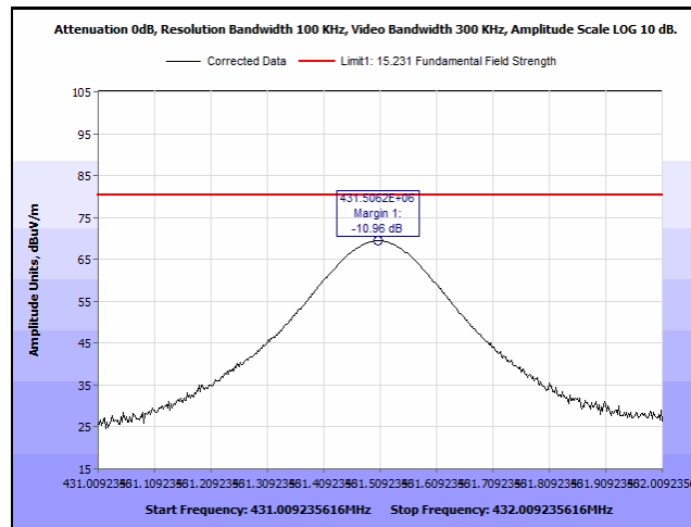
Plot 4. 431.5 MHz Low Channel
