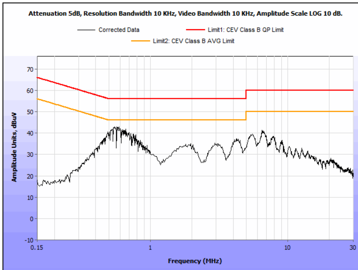
Plot 2. Conducted Emissions, 15.207(a), Neutral Line
