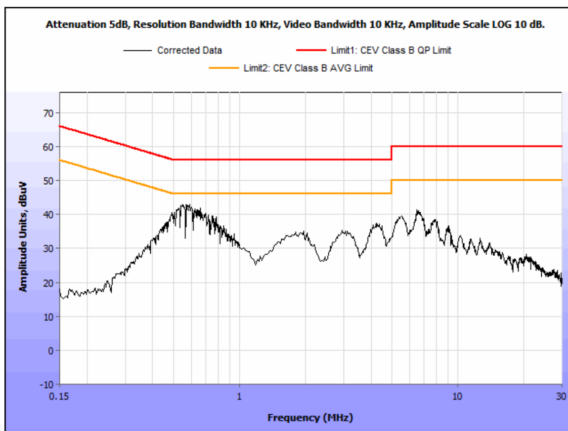
Plot 1. Conducted Emissions, 15.207(a), Phase Line
