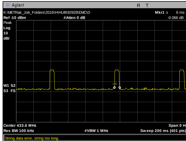
Plot 5. Duty Cycle, On OFF Time
