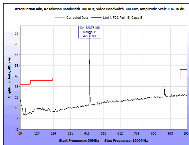
Plot 8. Radiated Spurious Emissions, 433.6 MHz Mid Channel Below 1 GHz
