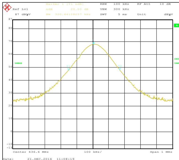
Plot 8. 20 dB Bandwidth Plot, 436.6 MHz High Channel
