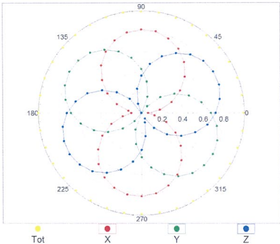
f=600 MHz,TEM
