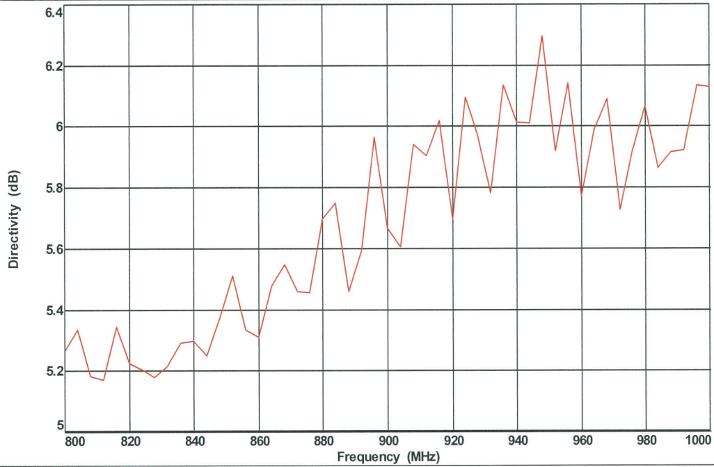
Directivity
