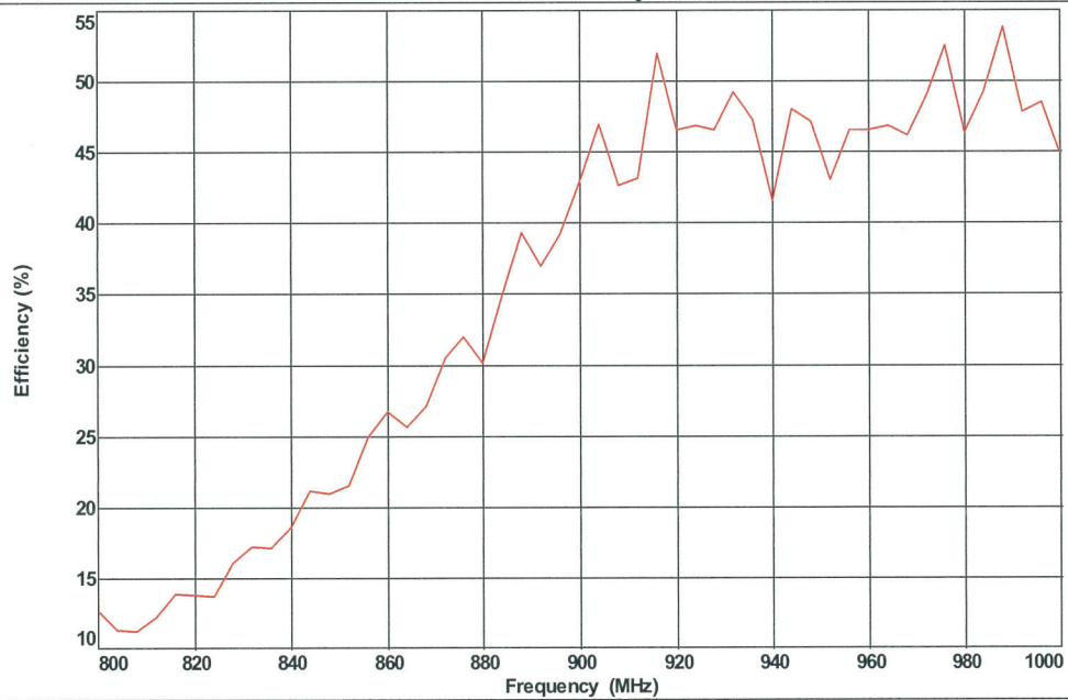
Efficiency
