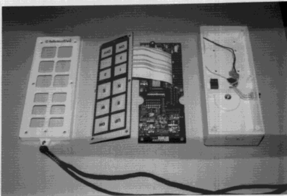
PHOTO C3 - INTERIOR VIEW OF OPEN CASE SHOWING FRONT SIDE OF CIRCUIT BOARDS
