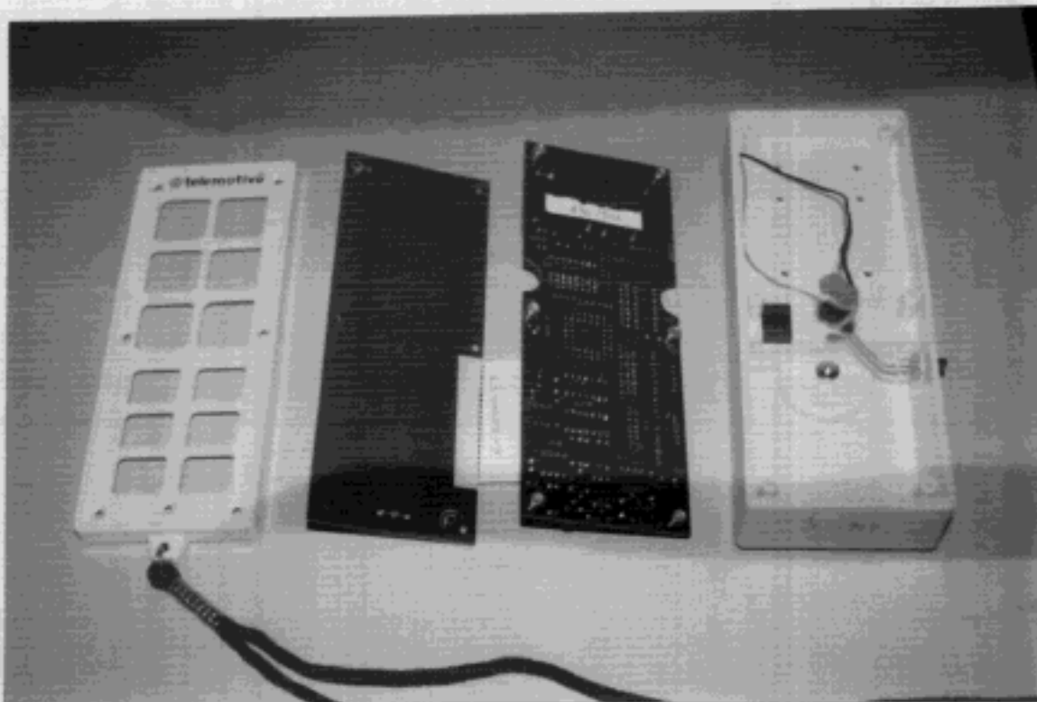
PHOTO C4 - INTERIOR VIEW OF OPEN CASE SIDE BACK SIDE OF CIRCUIT BOARDS
