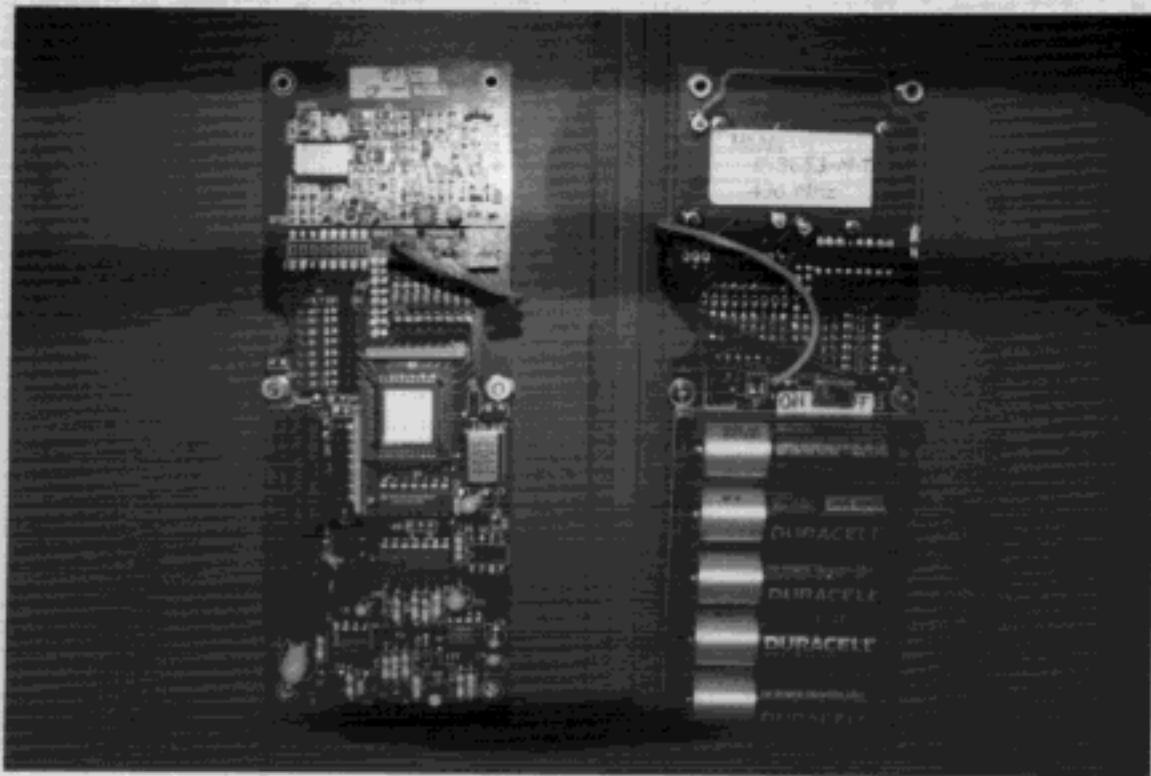
PHOTO C1: View of RF module circuit board, front and back
