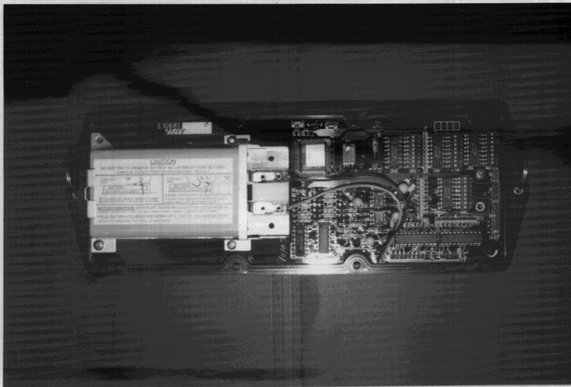
PHOTO C2: Interior view of open case (Back half) showing CPU.
