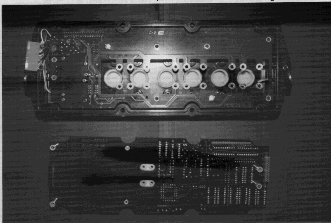
PHOTO C3: Interior view of open case (Front Half) showing switches and RF module.
