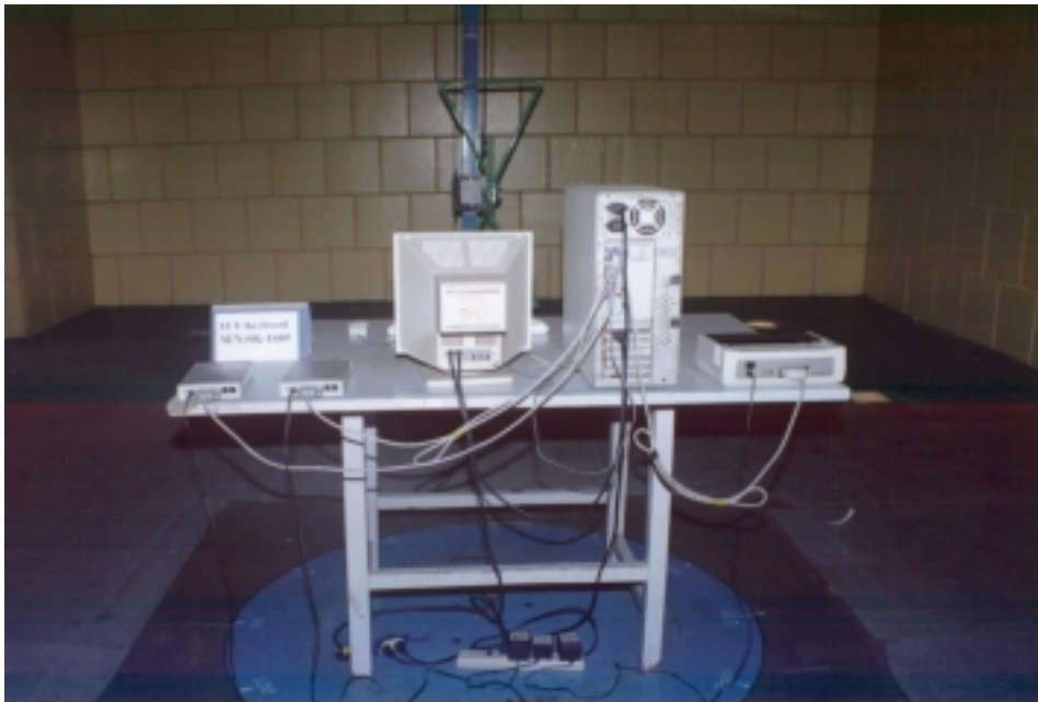
REAR VIEW OF RADIATED EMISSION TEST
