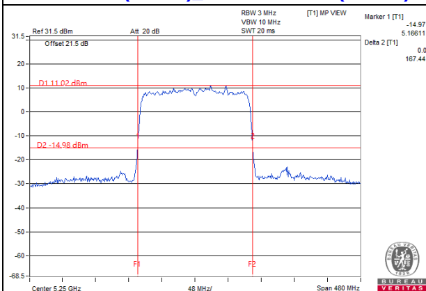
802.11ax (HE160)_Chain 1 / CH50 (U-NII-1)
