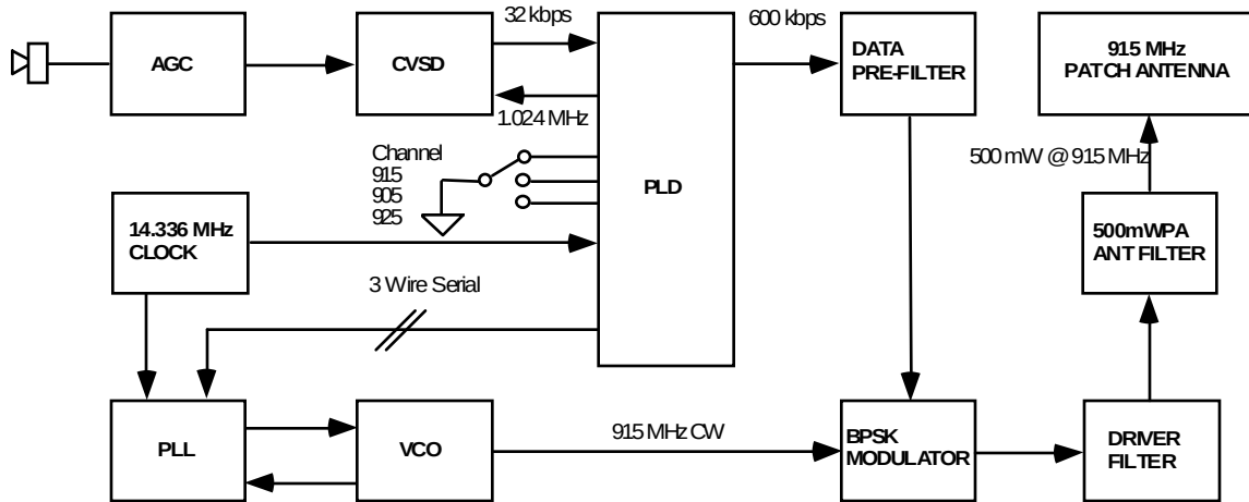
H25DSS950TX BLOCK DIAGRAM
