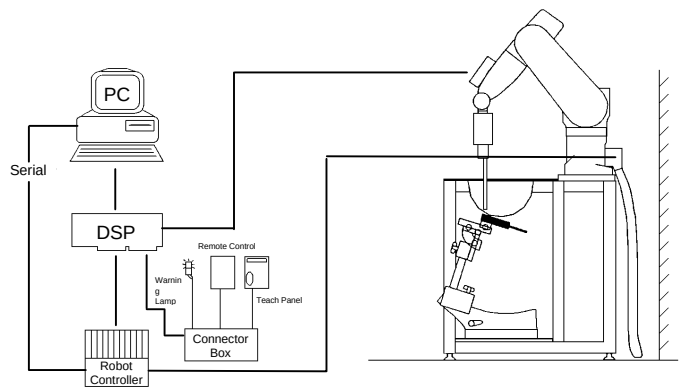
Figure 2. PCTEST SAR Lab II Test Measurement Set-up
