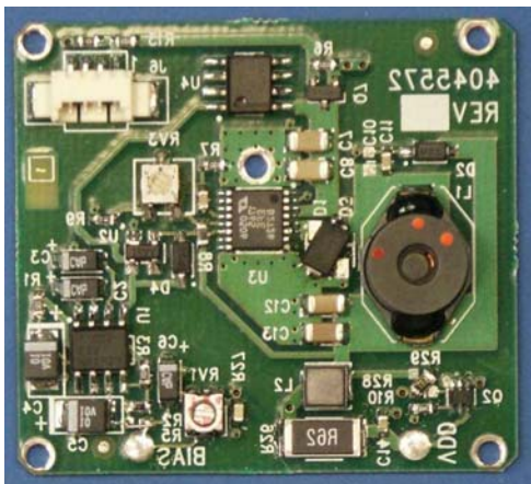
PA power supply Top and Bottom
