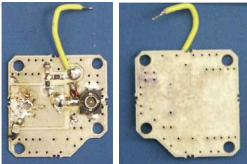
PA input Top and Bottom
