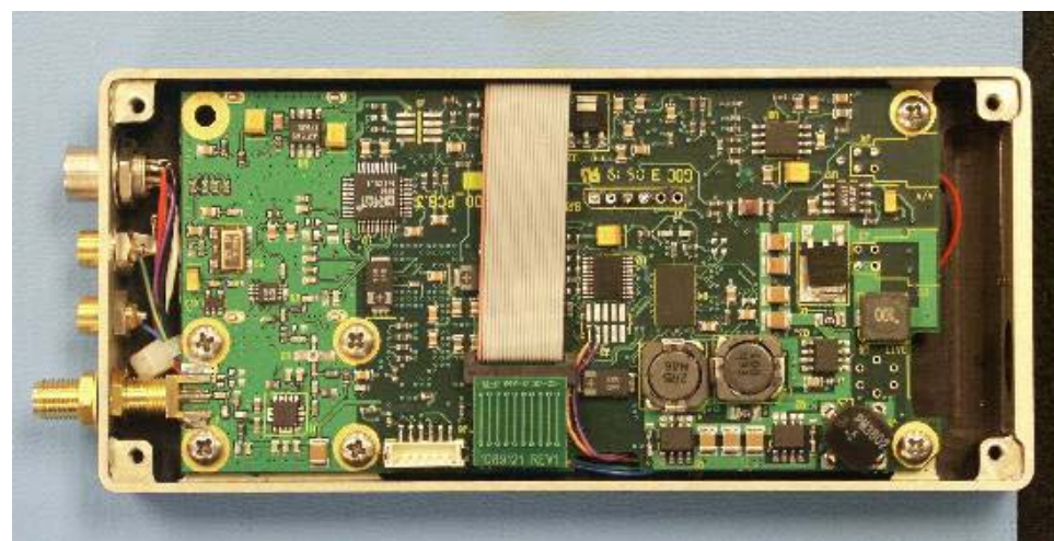
PCB In Housing
