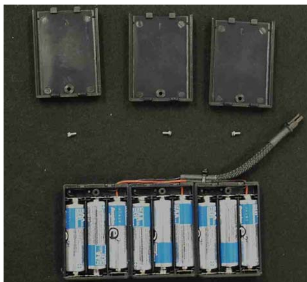
9 x AA Battery Assembly
