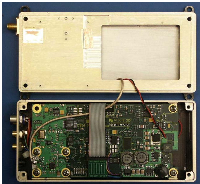
PCB In Housing
