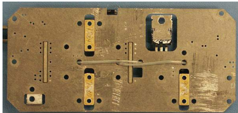
Stealth Microwave SM2325-37H Solid State RF Power Amplifier PCB
