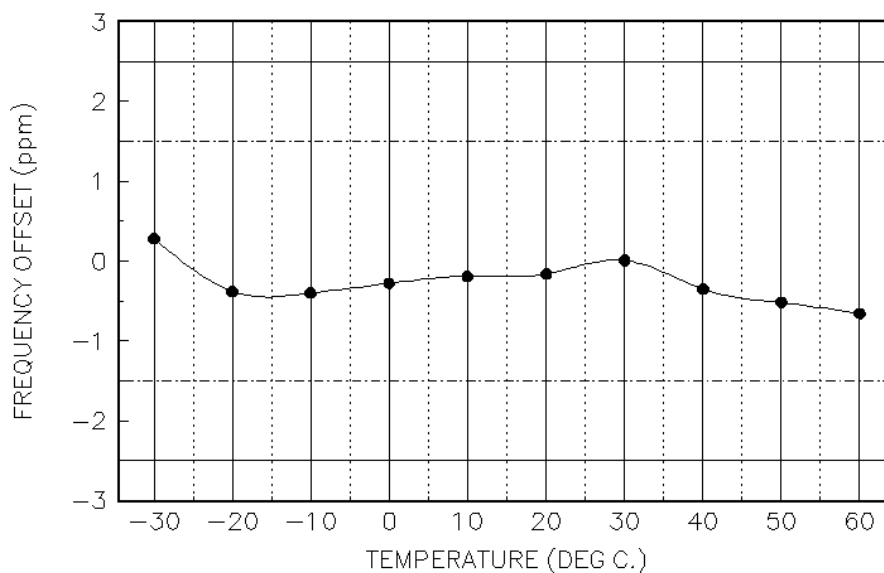
T2001 PROTO 1 FREQ OFFSET VS TEMP
