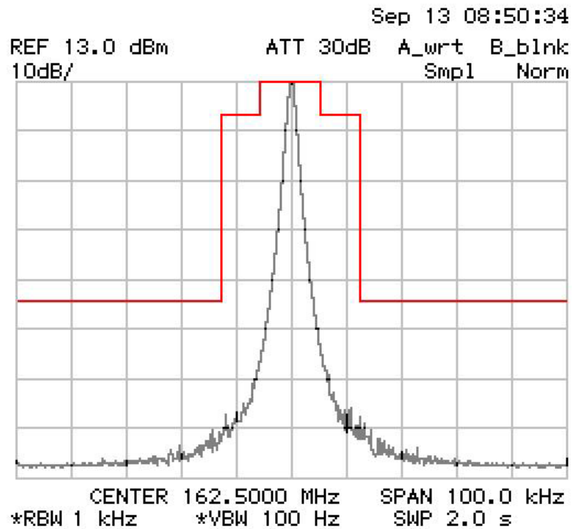
Figure 8 – Unmodulated Carrier
