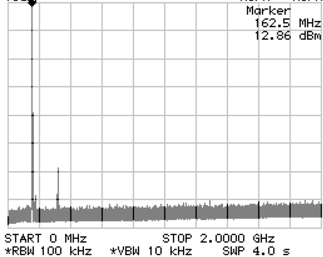
Figure 16 – Wide Band Spurious Emissions – Spectral Display
