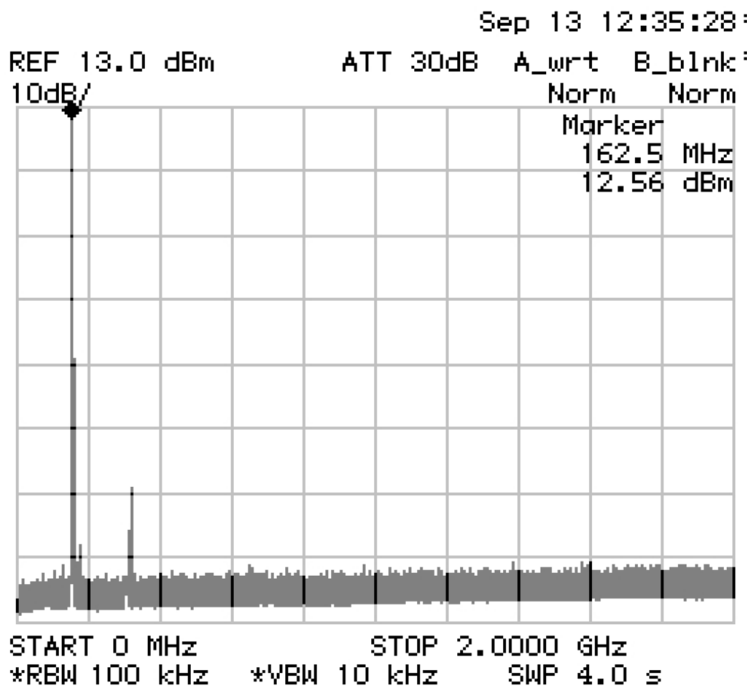
Figure 15 – Narrow Band Spurious Emissions – Spectral Display
