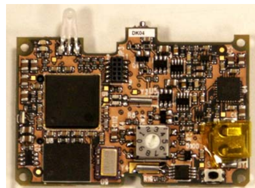
Digital board, top view
