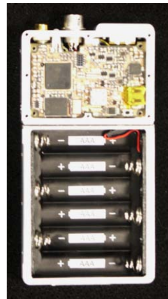
Top and bottom of unit with all covers removed
