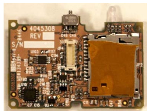
Digital board, bottom view
