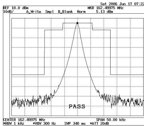
Figure 4 – Unmodulated Carrier
