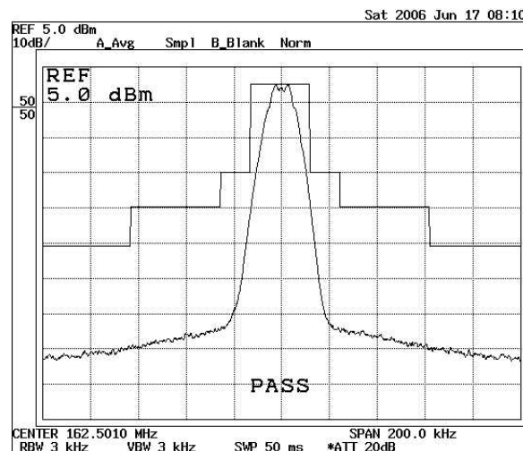
Figure 6 – Wide Band
