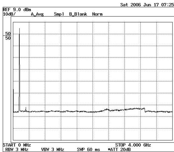
Fig 7 – Narrow Band Spurious Emissions – Spectral Display
