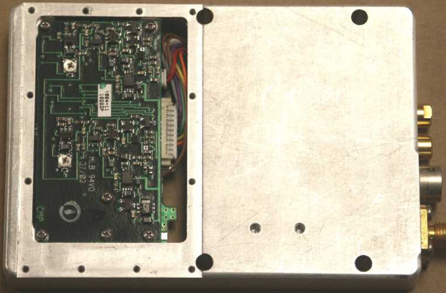
Audio PCB in VMS2000 chassis / back veiw
