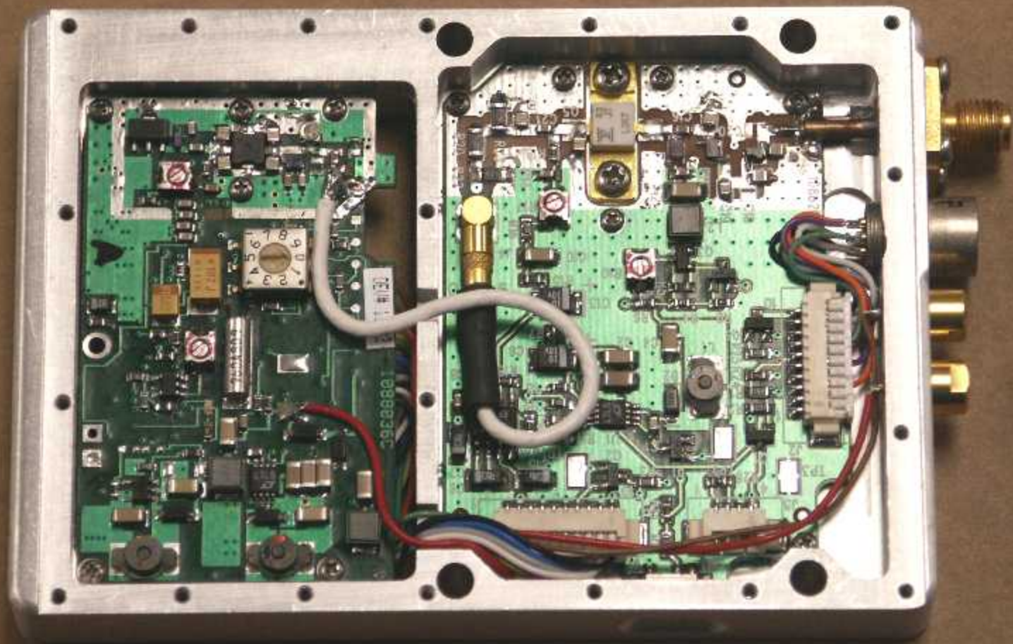
Video/RF driver PCB and 2 Watt Amplifier PCB in VMS2000 chassis - front view
