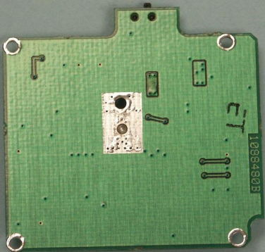
Power Supply Brd Back
