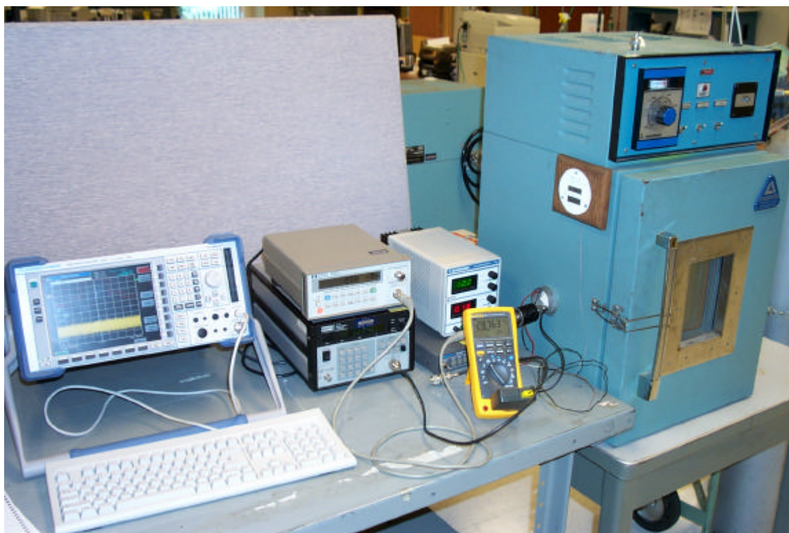
Frequency and RF power over temperature test setup:
