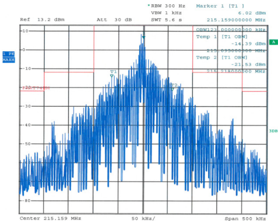
Figure 19: Emission Mask (High CH)
