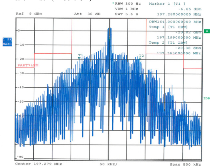
Figure 18: Emission Mask (Middle CH)
