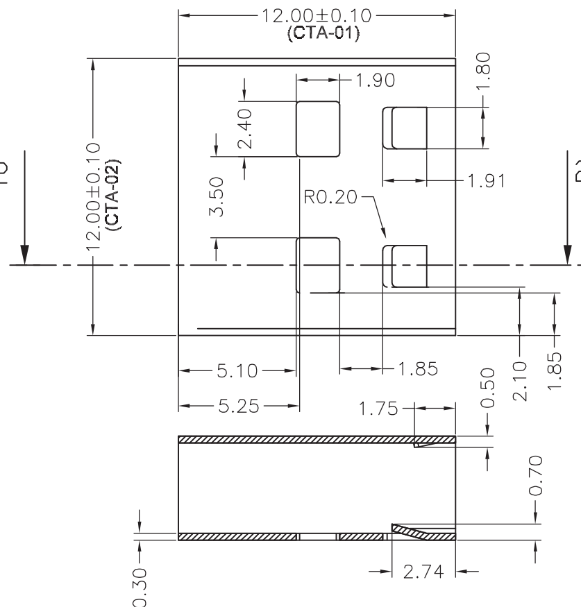
SECTION 2-2
