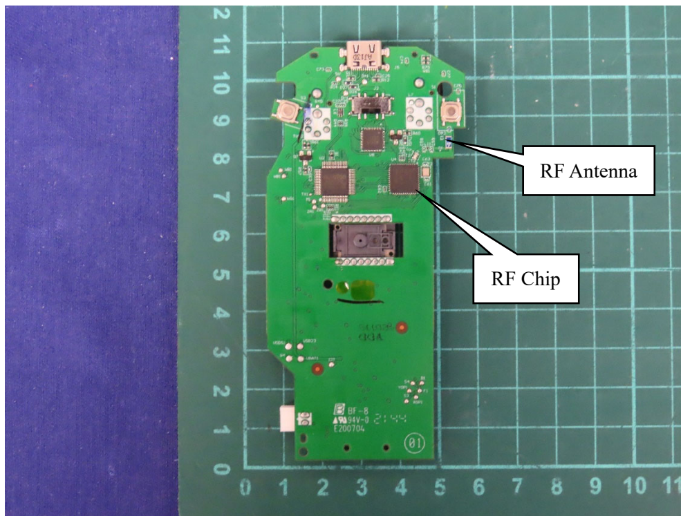
(22) EUT Photo
