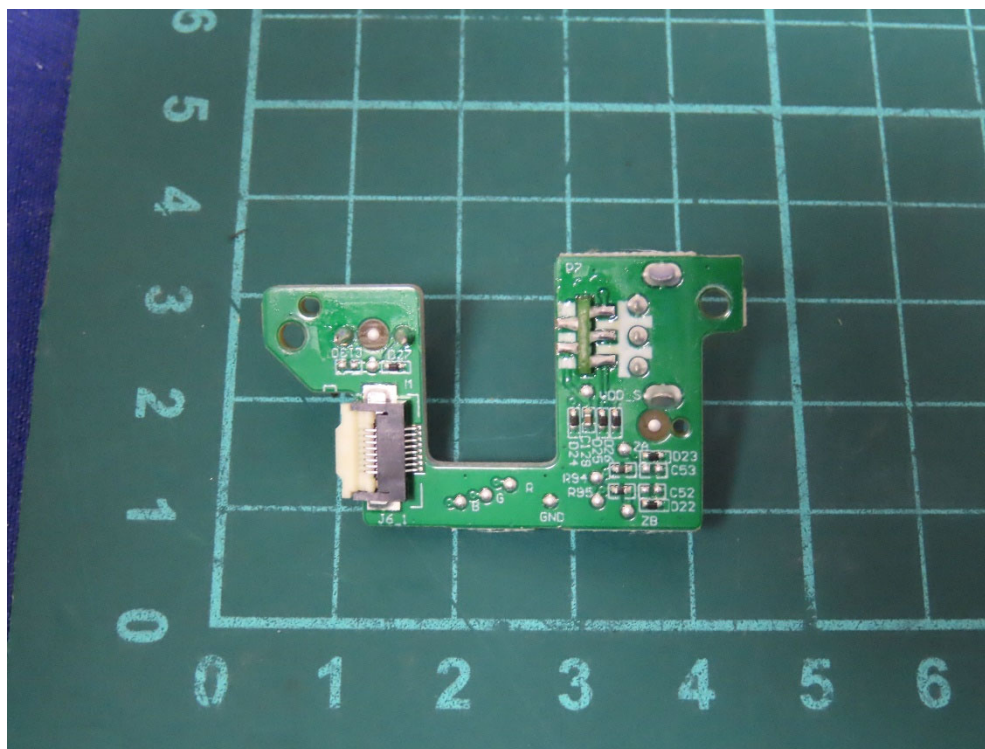
(11) EUT Photo
