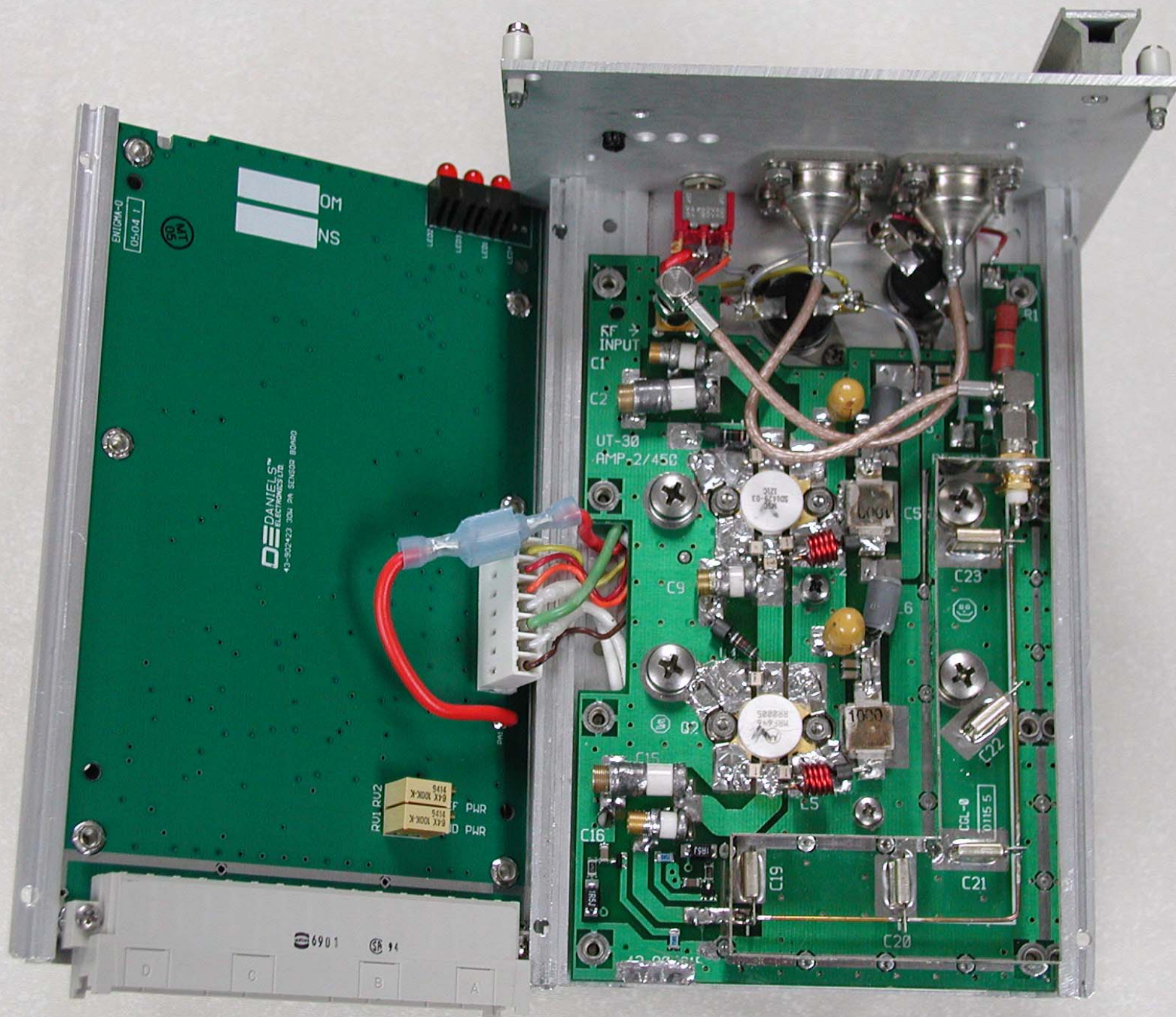
BOTH BOARDS (SHIELDS REMOVED)
