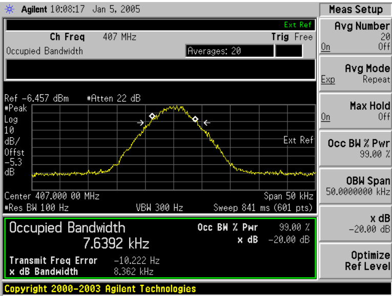
Amplifier Output 407 MHz F1E Modulation Input
