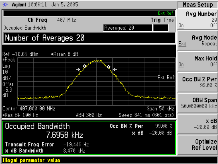
Exciter Output (Amplifier Input) 407 MHz F1E Modulation
