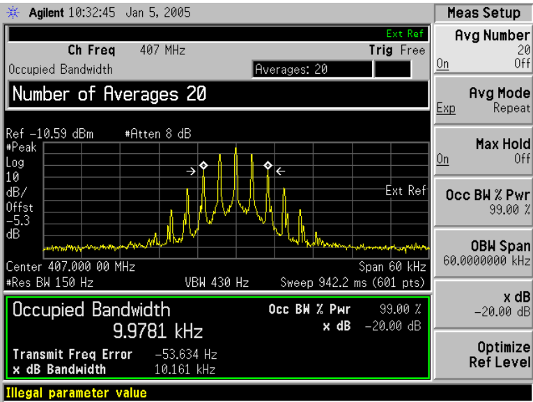
Exciter Output (Amplifier Input) 407 MHz F3E Modulation
