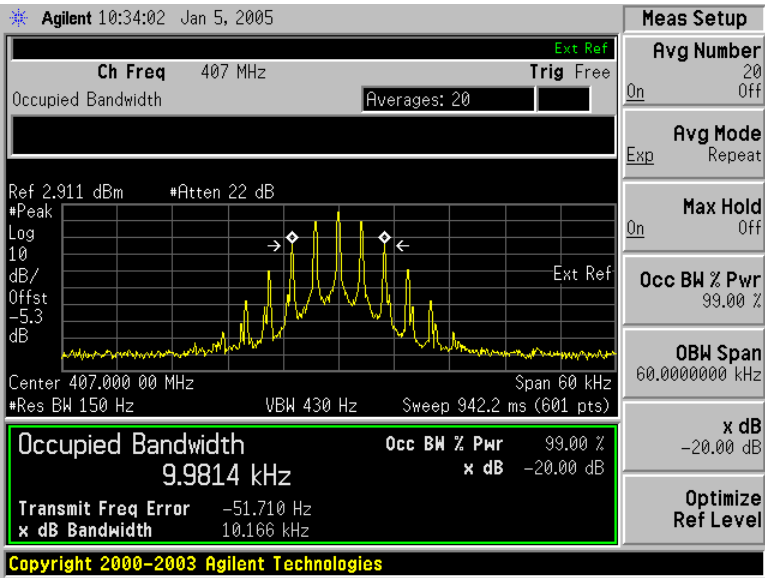
Amplifier Output 407 MHz F3E Modulation Input
