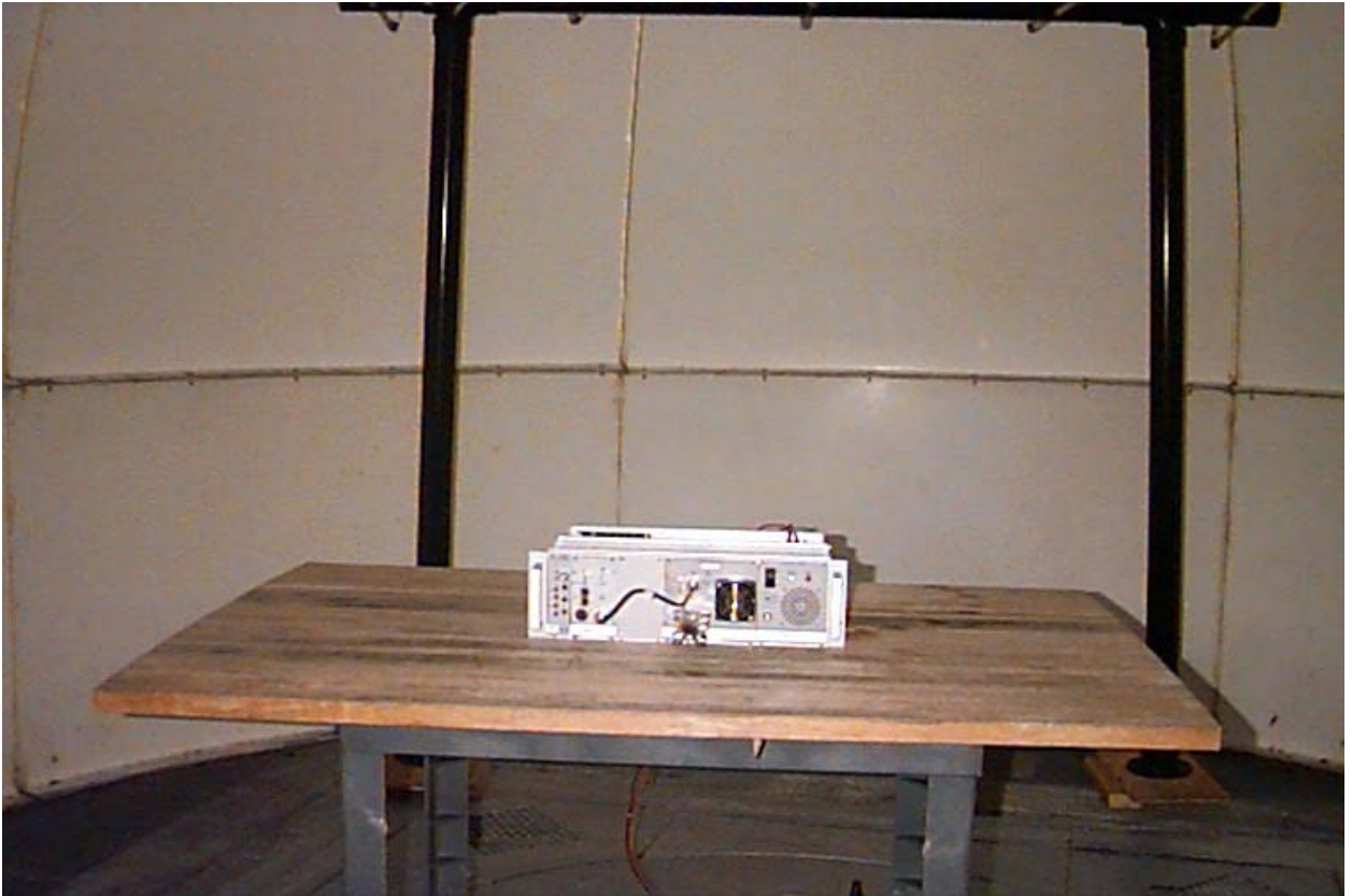
Radiated Emissions Set-Up Photo
