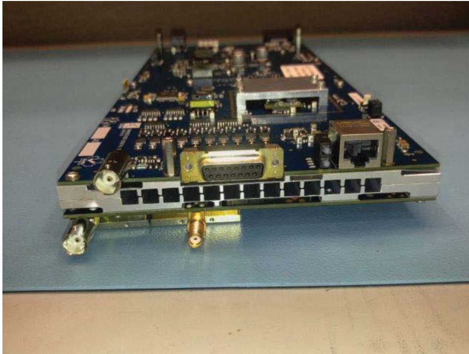
Transceiver- Top
