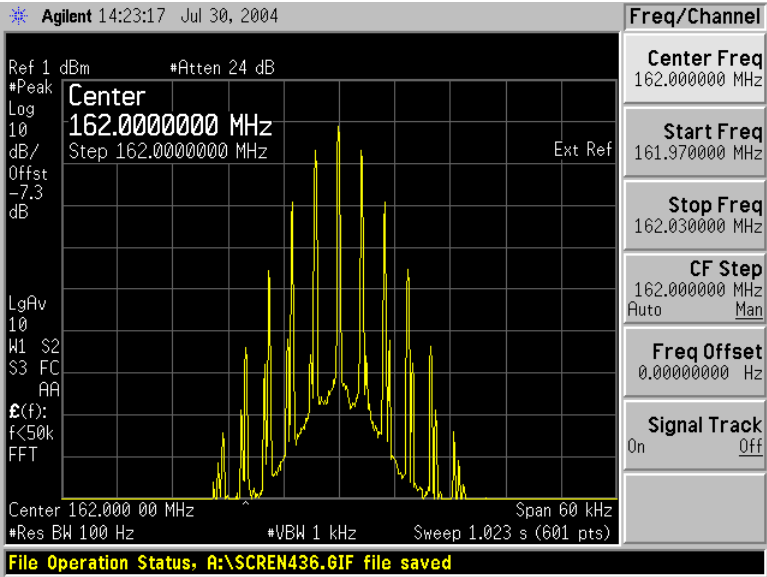
Exciter Output (Amplifier Input) 162 MHz F3E Modulation
