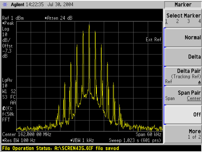
Amplifier Output 162 MHz F3E Modulation Input
