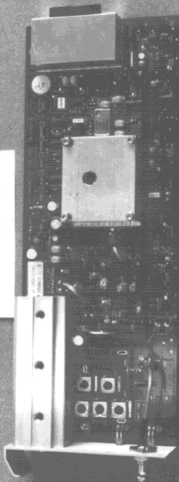
UHF TRANSMITTER TYPE 2950 HAWK SINGLE & DUAL CHANNEL POINT TO POINT LINK
