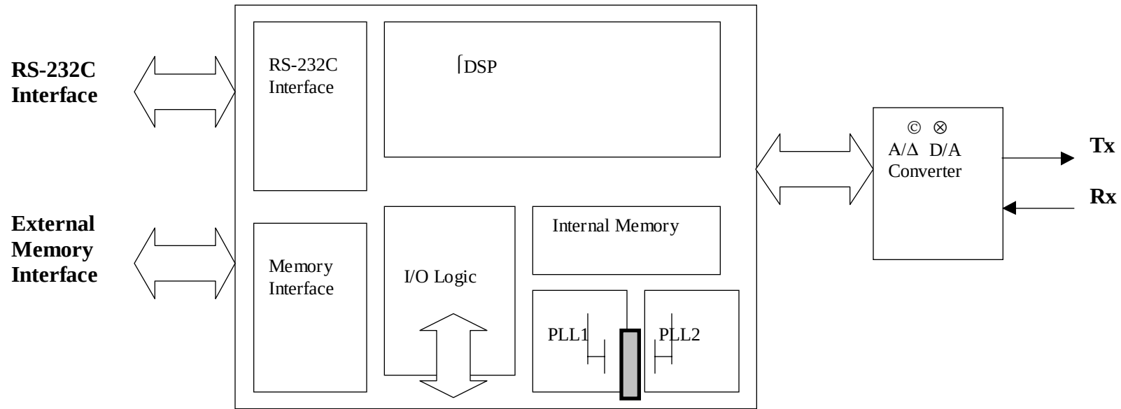
Block Diagram
