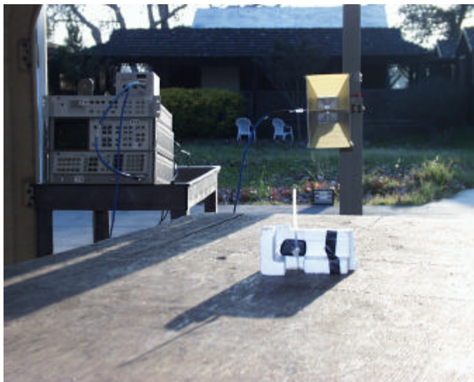
High Frequency Test Set-up
