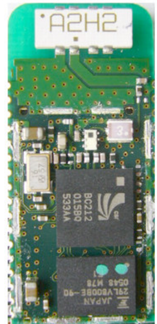
Bottom View of a Bluetooth Module
