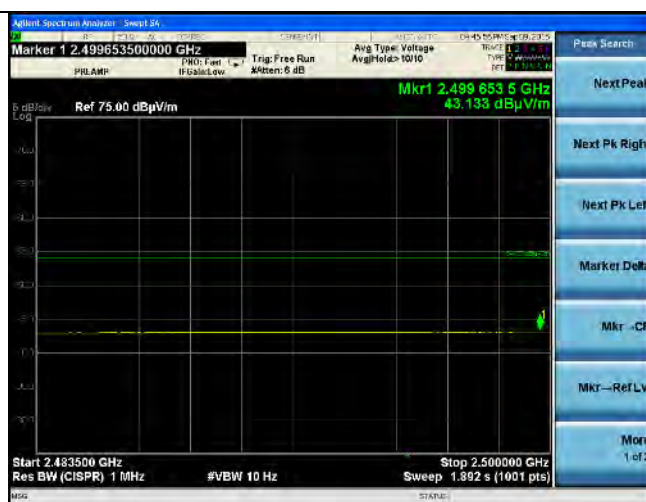
11MBPS Upper band edge Average
