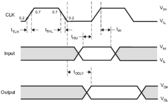
Figure 5 SDIO Clock Timing
